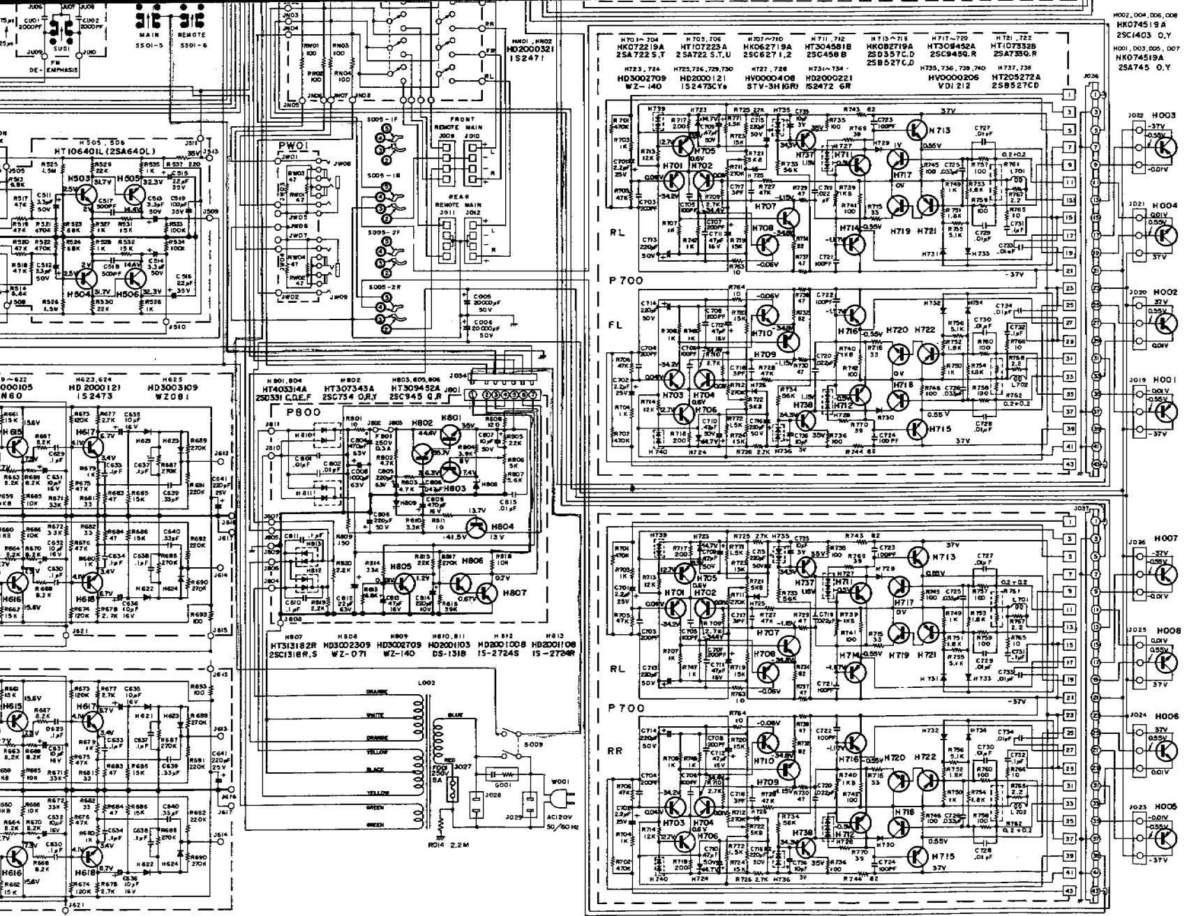
This Schematic Diagram should be apply to Serial NO. 1001 to 4500.
