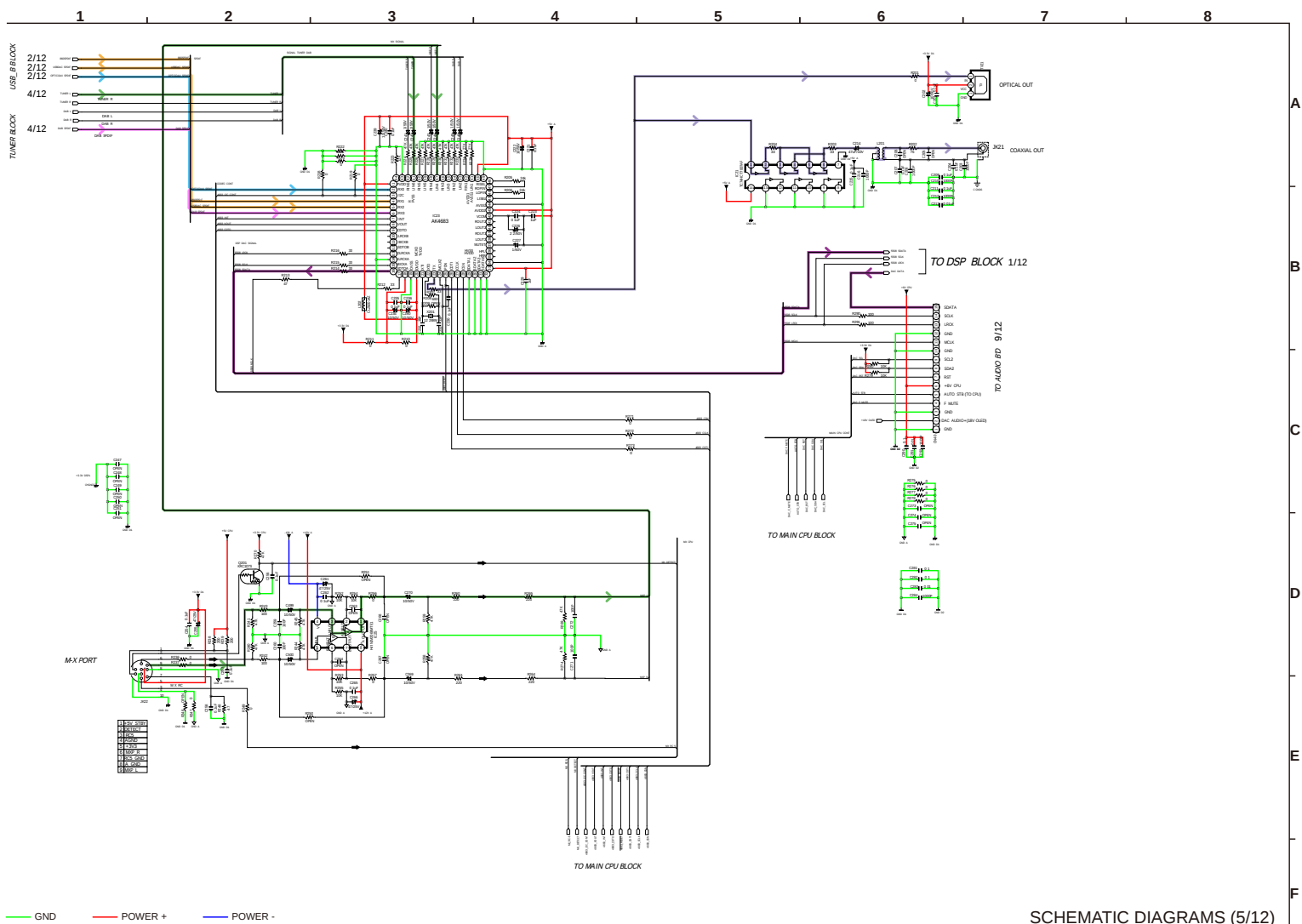
SCHEMATIC DIAGRAMS (5/12)
