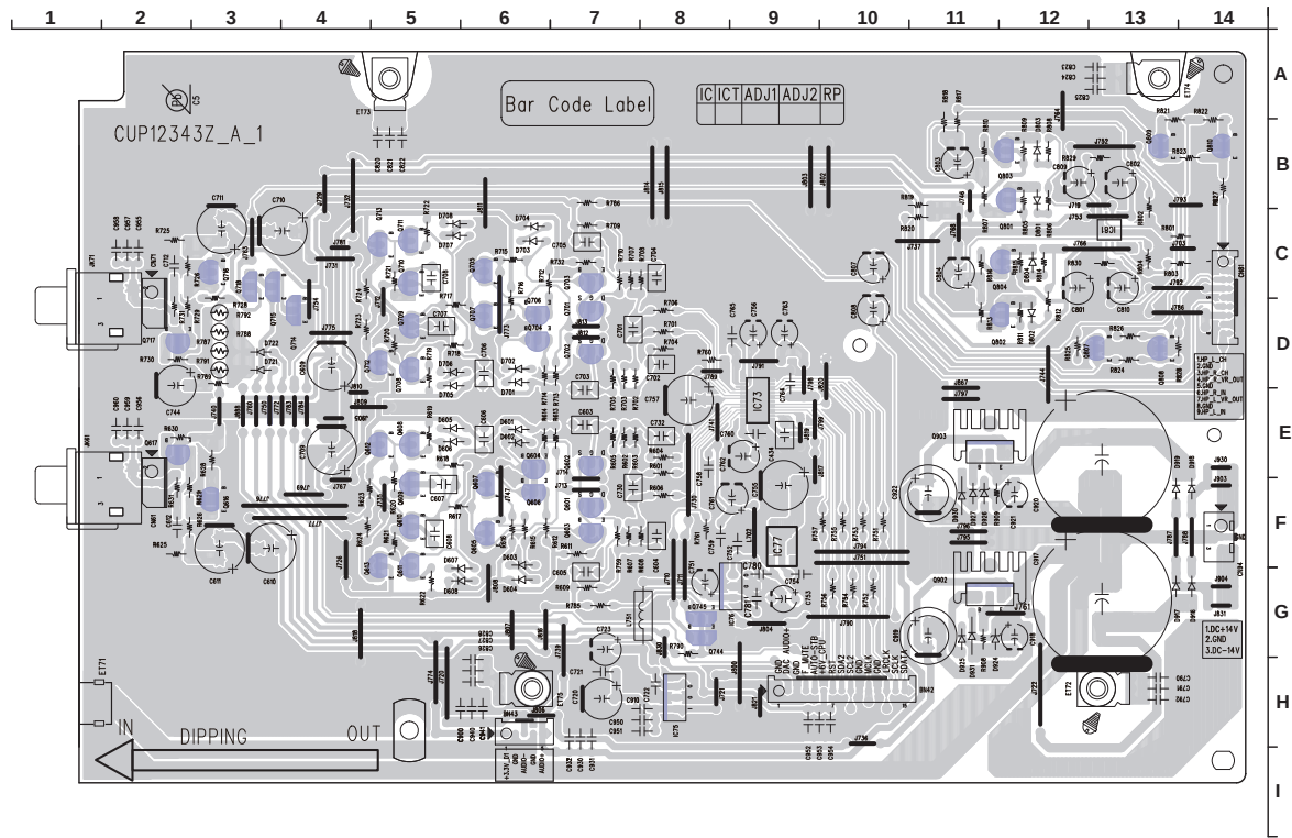
AUDIO PCB (COMPONENT SIDE)
