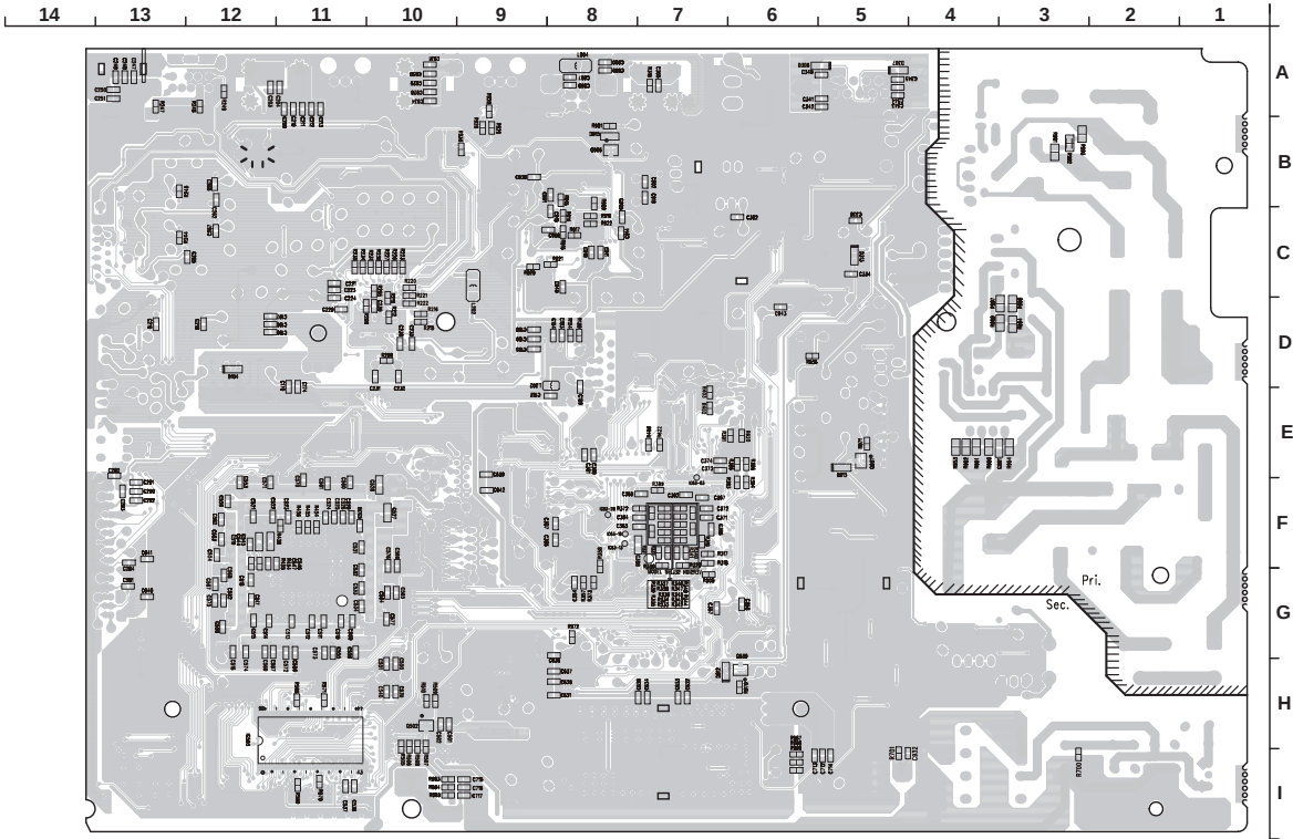
MAIN PCB (FOIL SIDE)
