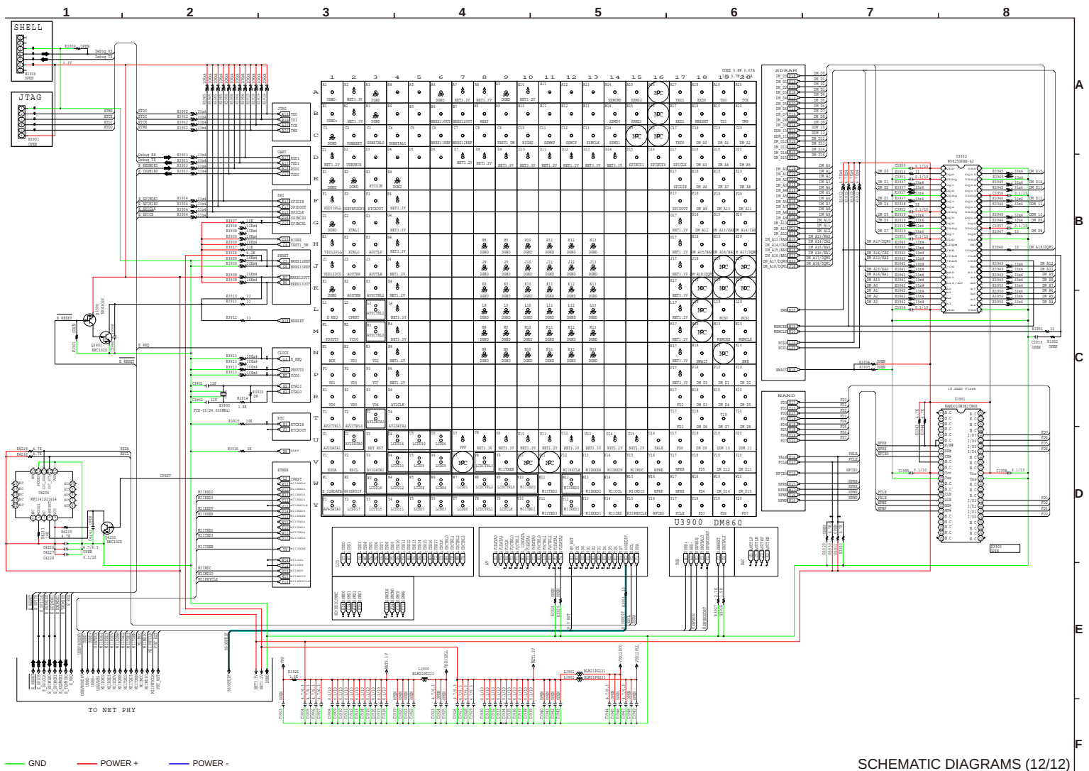
SCHEMATIC DIAGRAMS (12/12)
