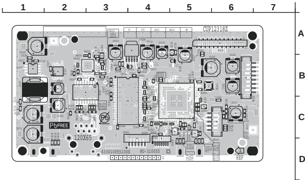
ETHERNET PCB (COMPONENT SIDE)
