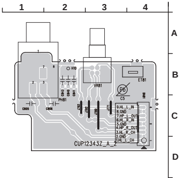
PHONE PCB (COMPONENT SIDE)
