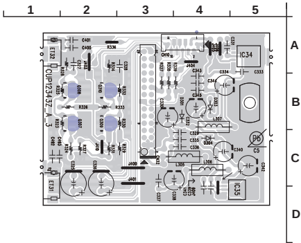
DAB PCB (COMPONENT SIDE)
