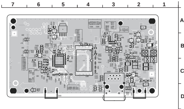
ETHERNET PCB (FOIL SIDE)
