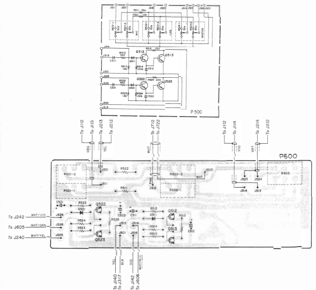
6.9 VOLUME & PEAK BOARD SCHEMATIC DIAGRAM AND COMPONENT LOCATIONS - P500
