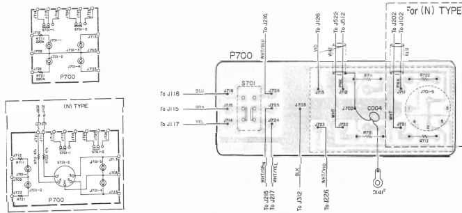
6.7 TERMINALS BOARD SCHEMATIC DIAGRAM AND COMPONENT LOCATIONS - P700
