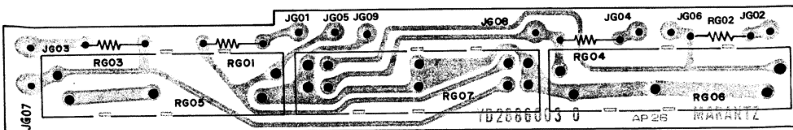
Figure 21. Balance Control Unit Assembly PG01 Component Locations
