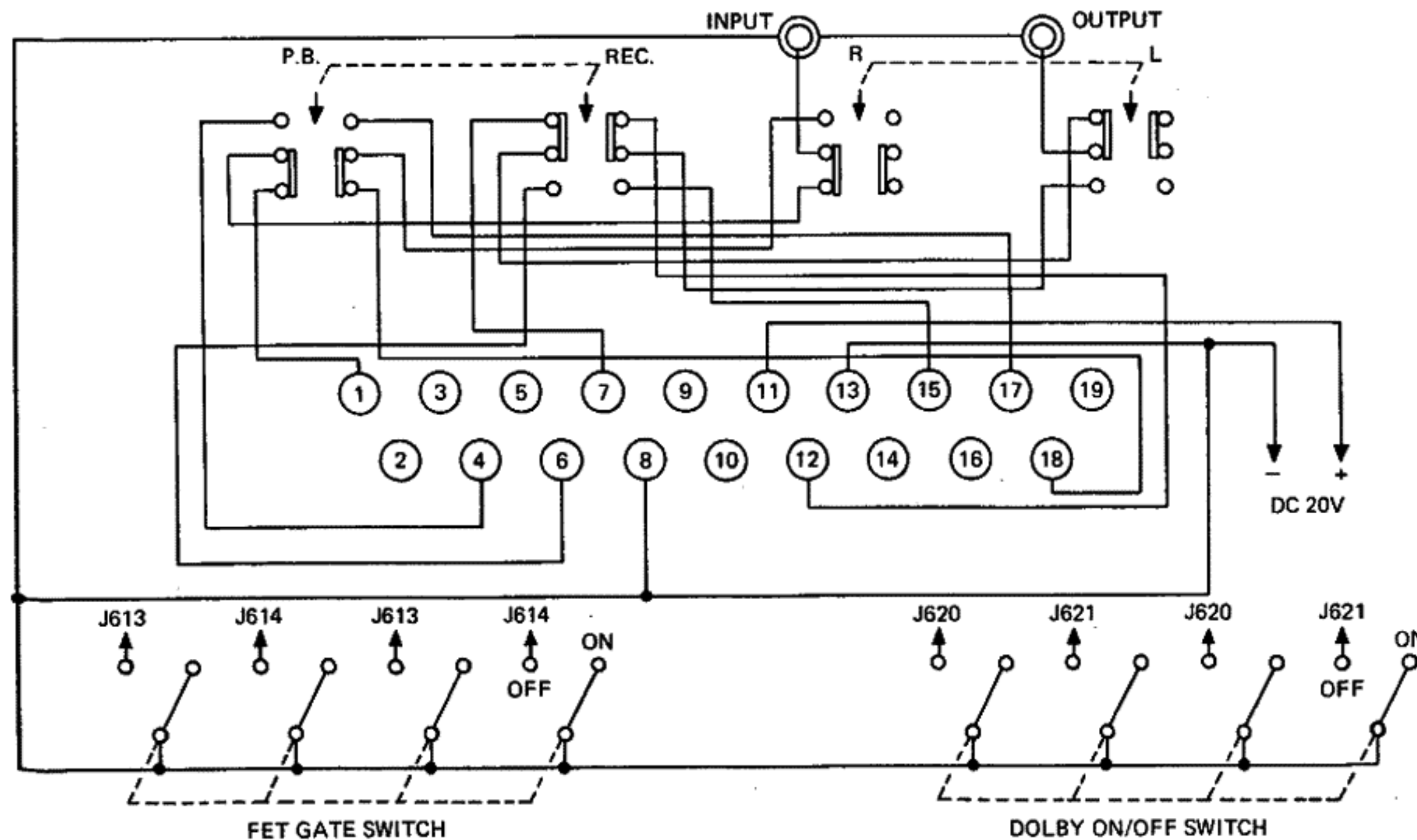
Figure 3. Dolby Alignment Implement Simplified Schematic
