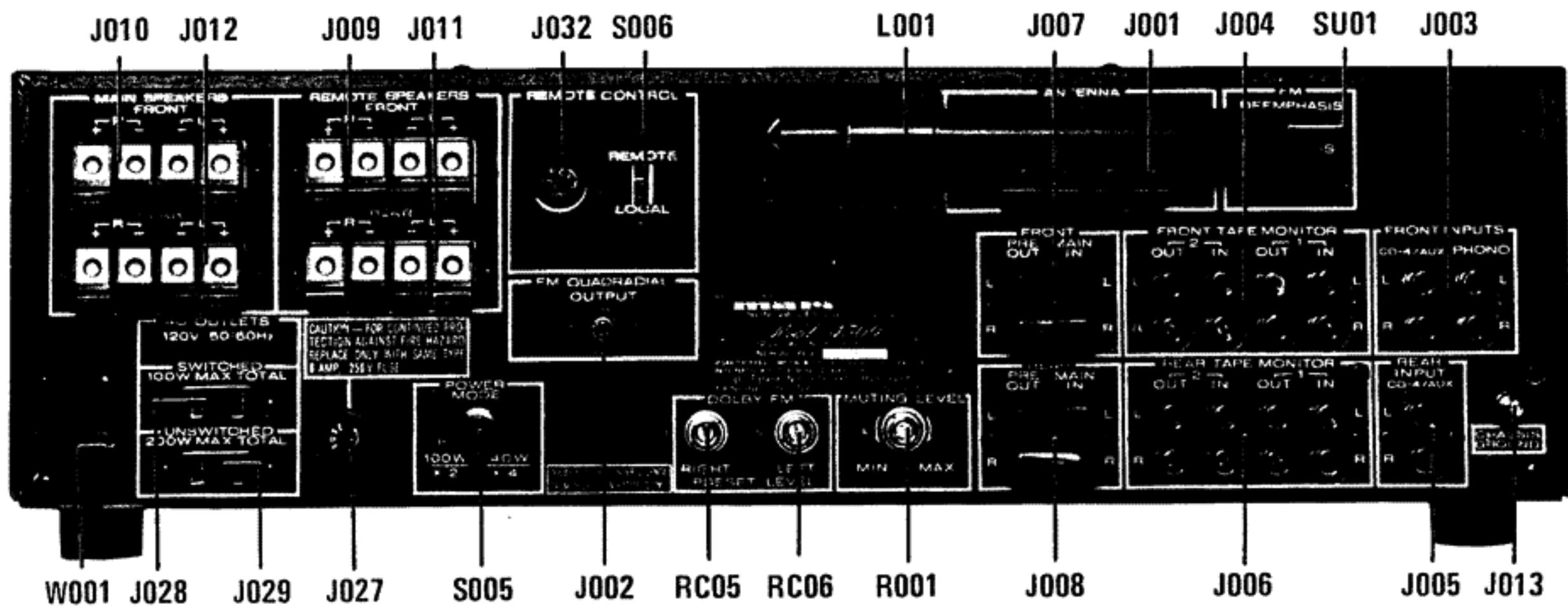
Figure 6. Rear Panel Adjustment and Component Locations
