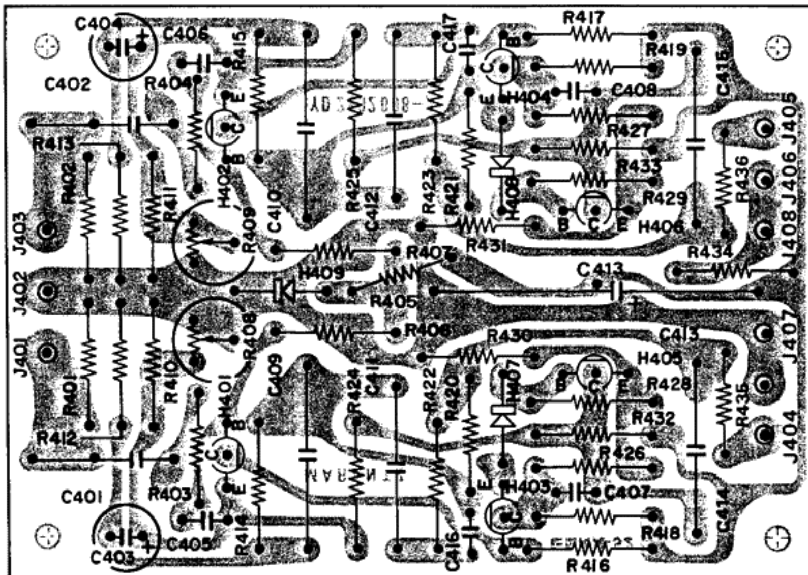
Figure 12. Phono Amplifier Assembly P400 Component Locations
