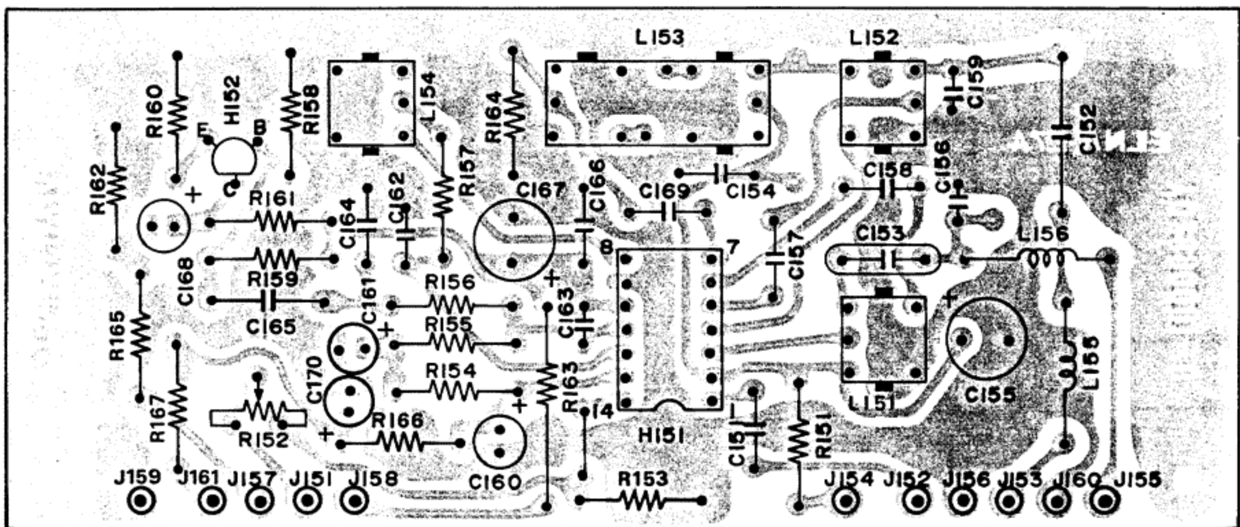
Figure 9. AM Tuner Assembly P150 Component Locations
