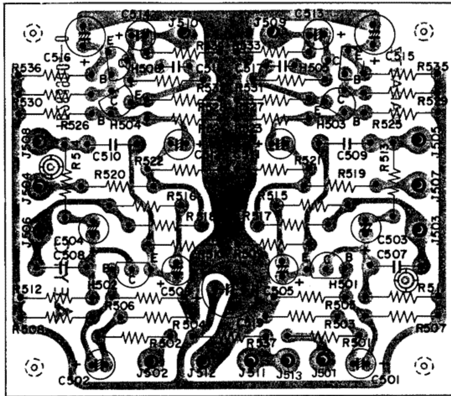
Figure 13. Vari-Matrix Assembly P500 Component Locations
