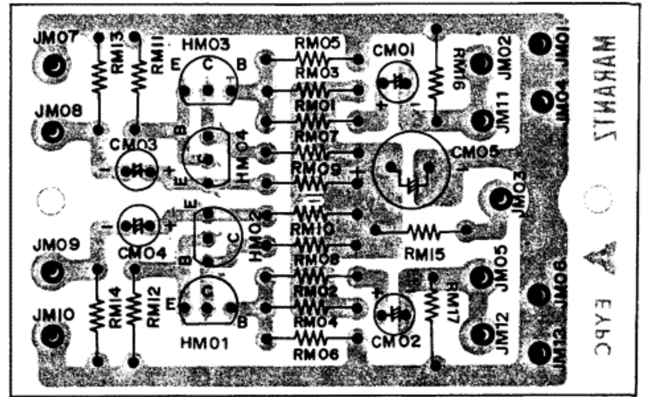
Figure 23. Phase Converter Assembly PM01 Component Locations
