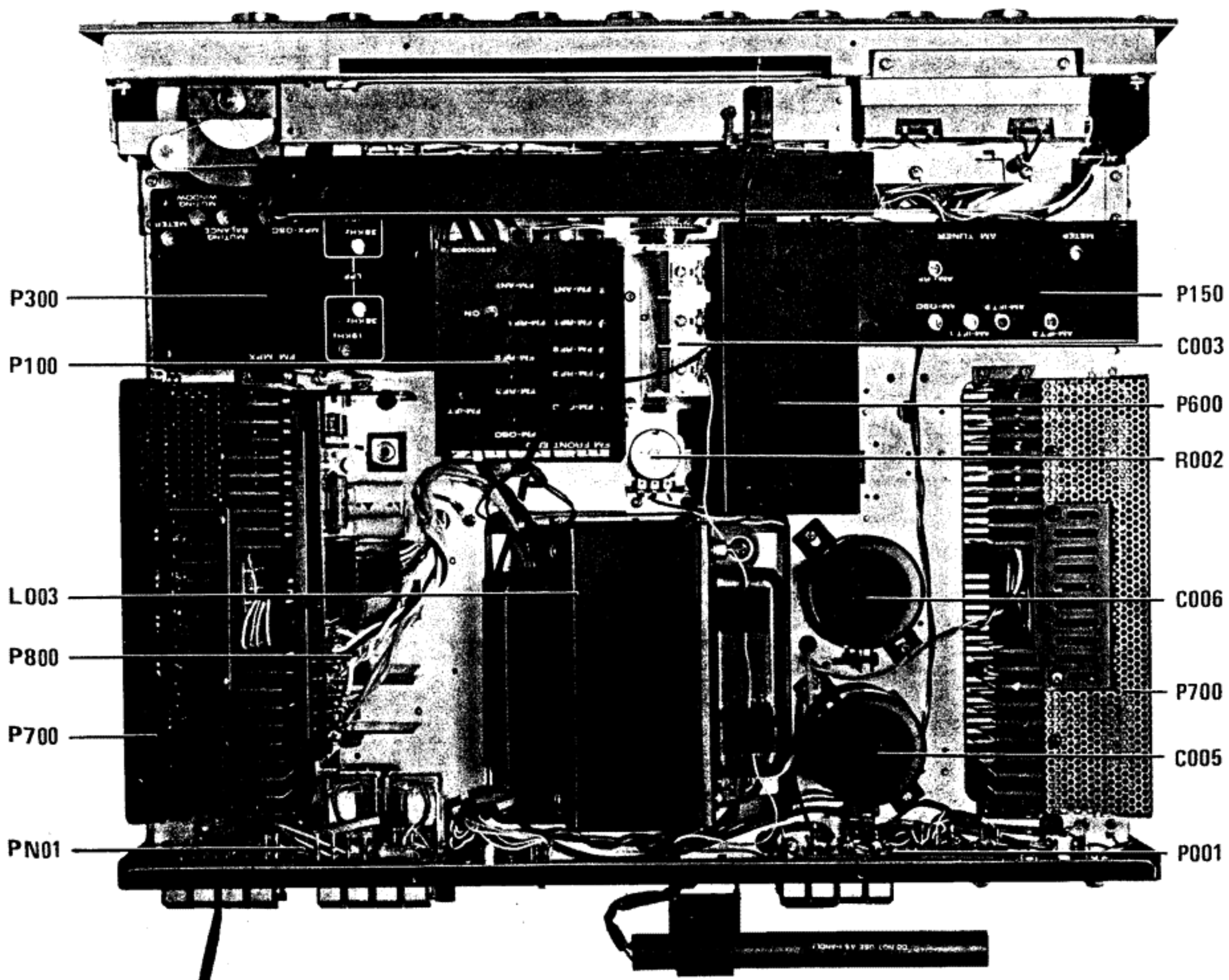
Figure 7. Main Chassis Component Locations (Top View)
