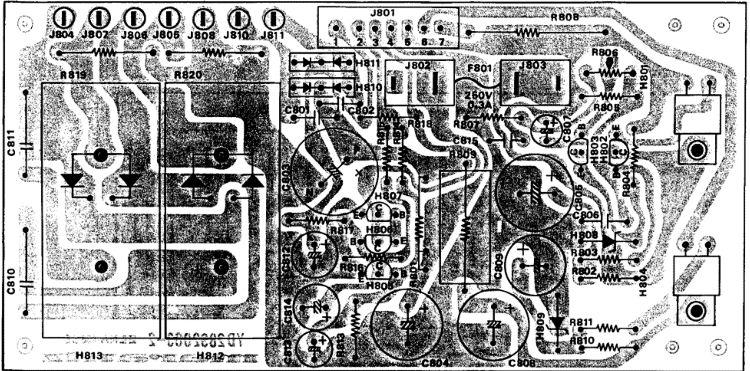
Figure 16. Power Supply Assembly P800 Component Locations
