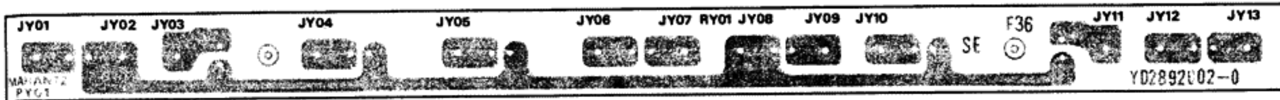
Figure 29. Selector Lamps Assembly PY01 Component Locations
