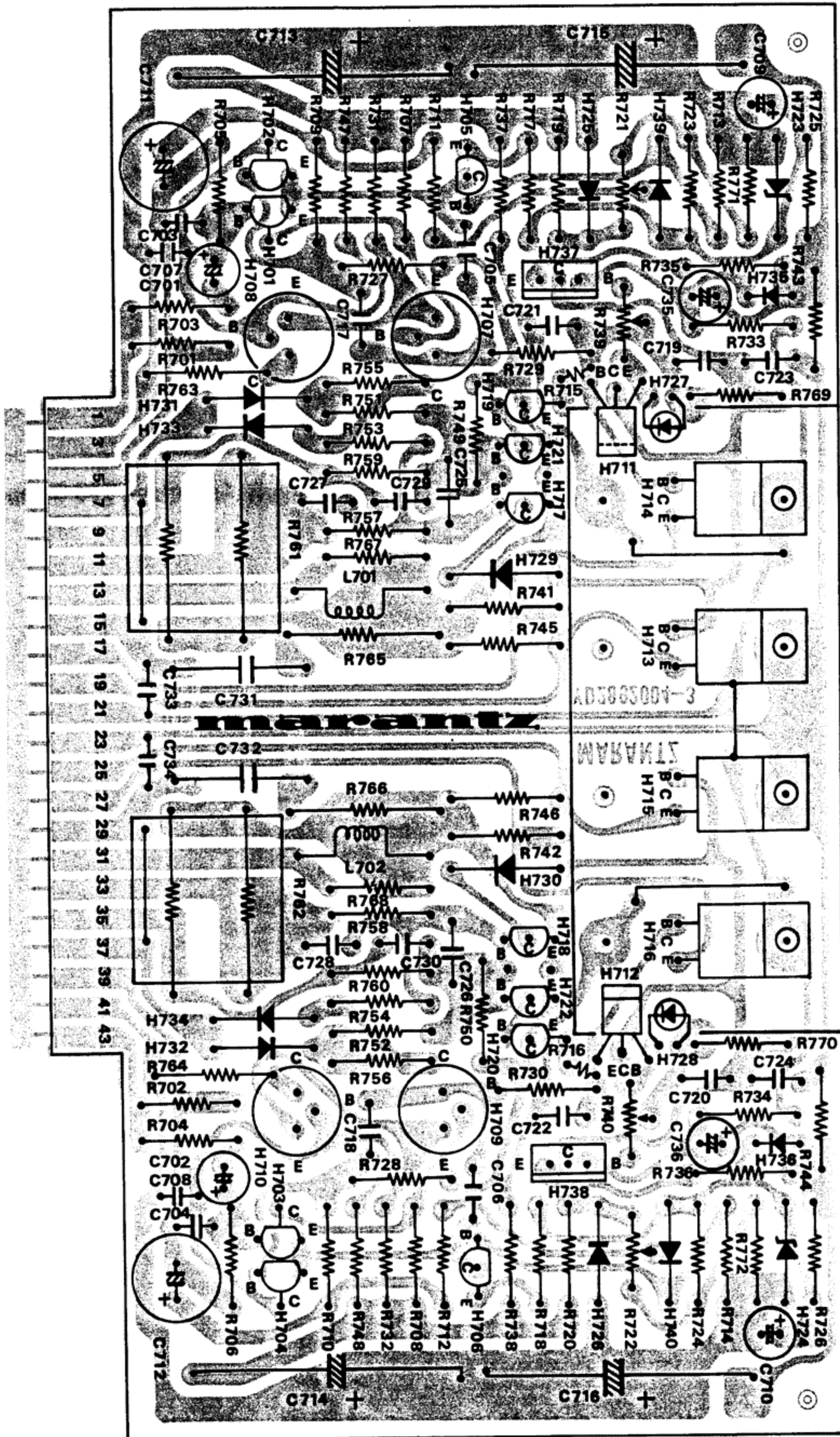
Figure 15. Power Amplifier Assembly P700 Component Locations
