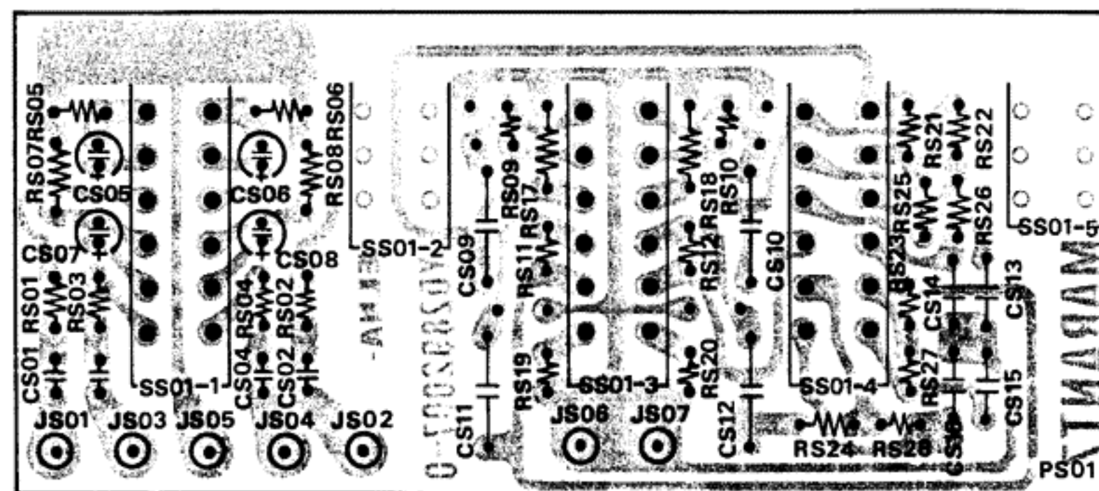
Figure 25. Switch Unit Assembly PS01 Component Locations
