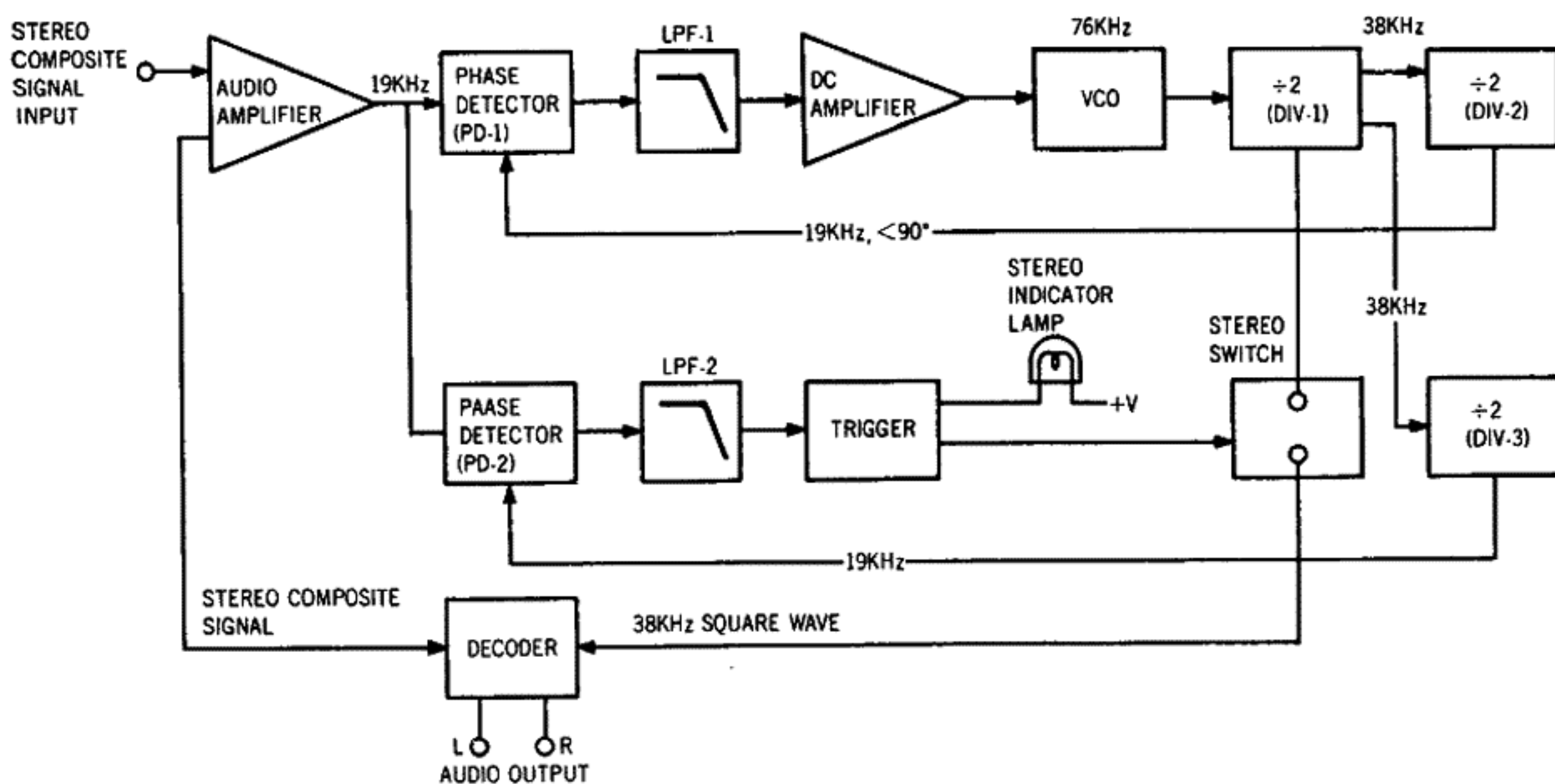
Figure 1. Block Diagram of the HA1156
