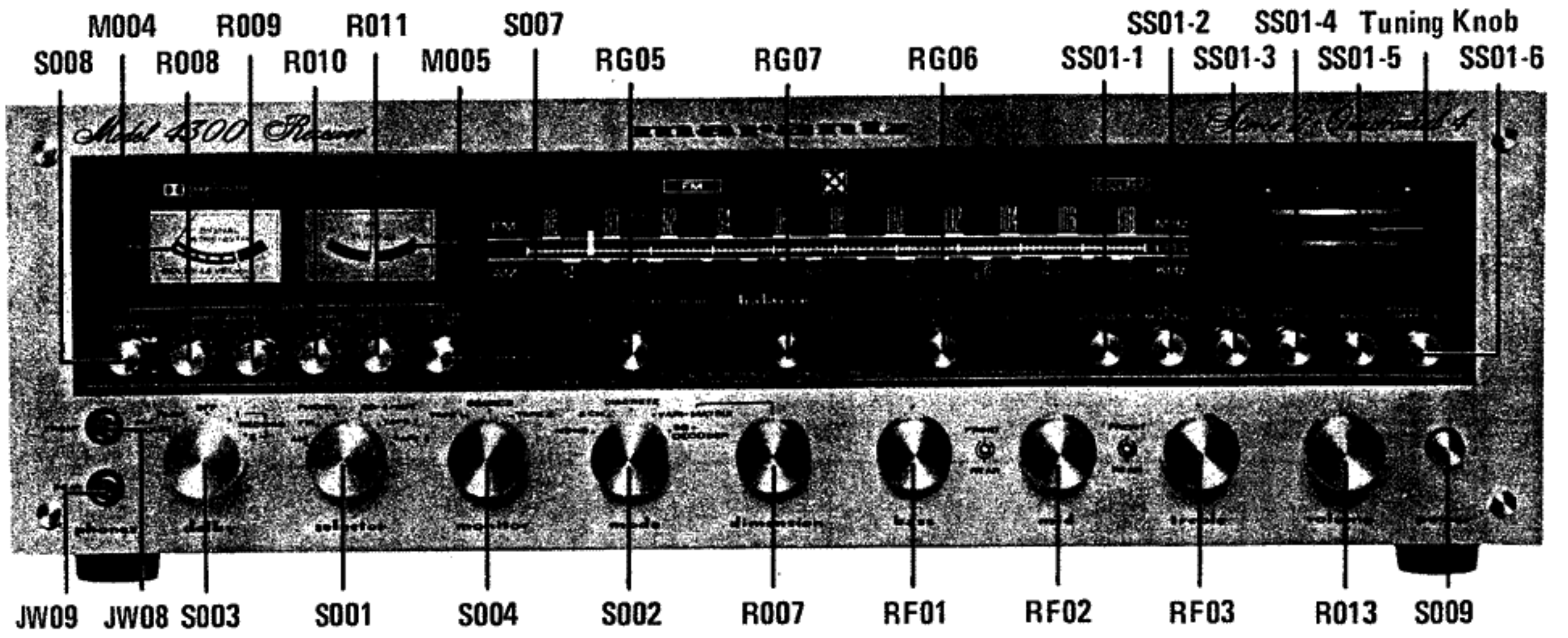
Figure 4. Front Panel Adjustment and Component Locations
