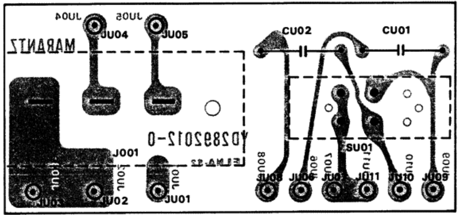
Figure 26. FM De-emphasis Assembly PU01 Component Locations
