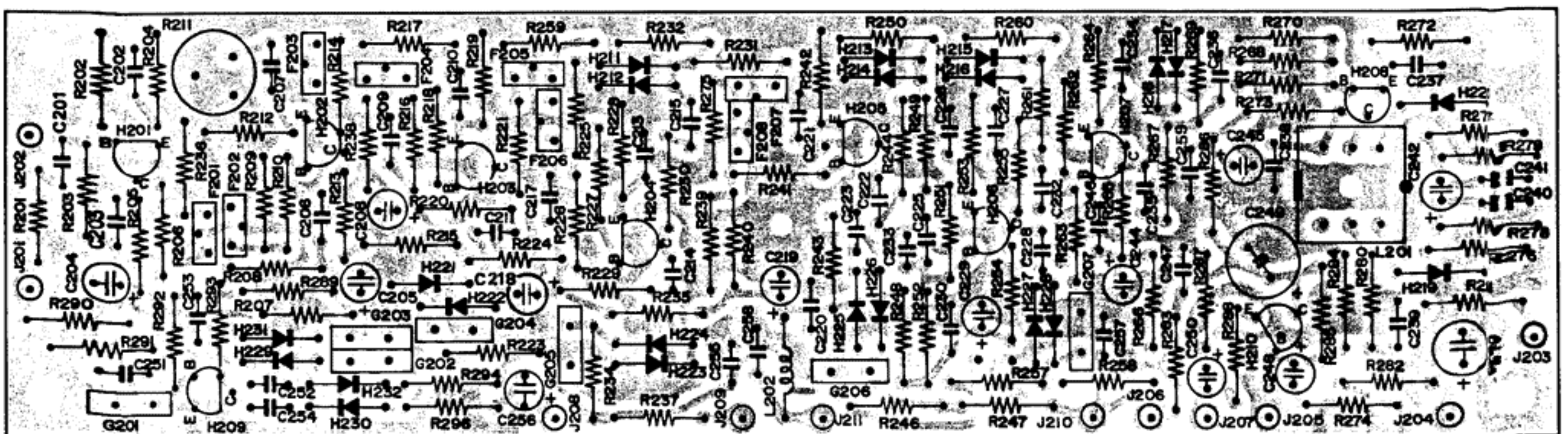
Figure 10. FM IF Amplifier Assembly P200 Component Locations
