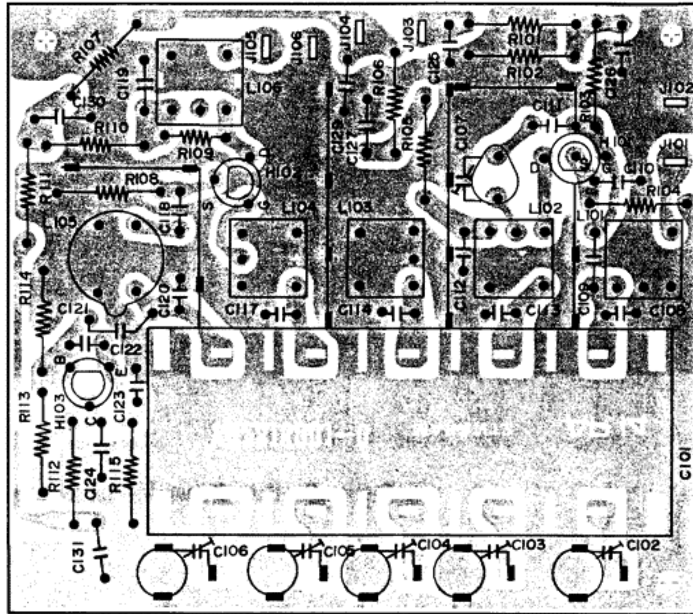
Figure 8. FM Front End Assembly P100 Component Locations
