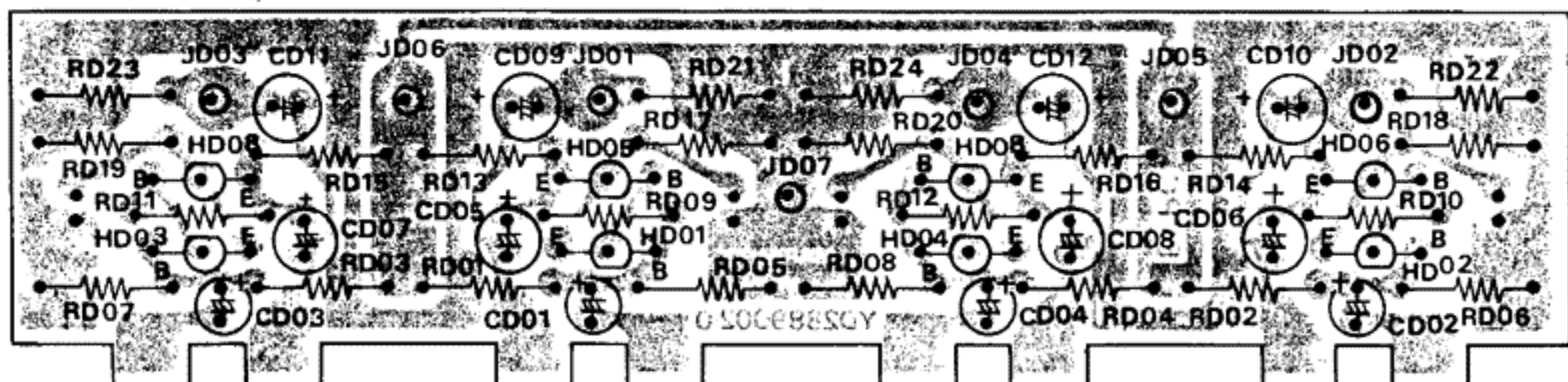
Figure 18. Tone Amplifier Assembly PD01 Component Locations
