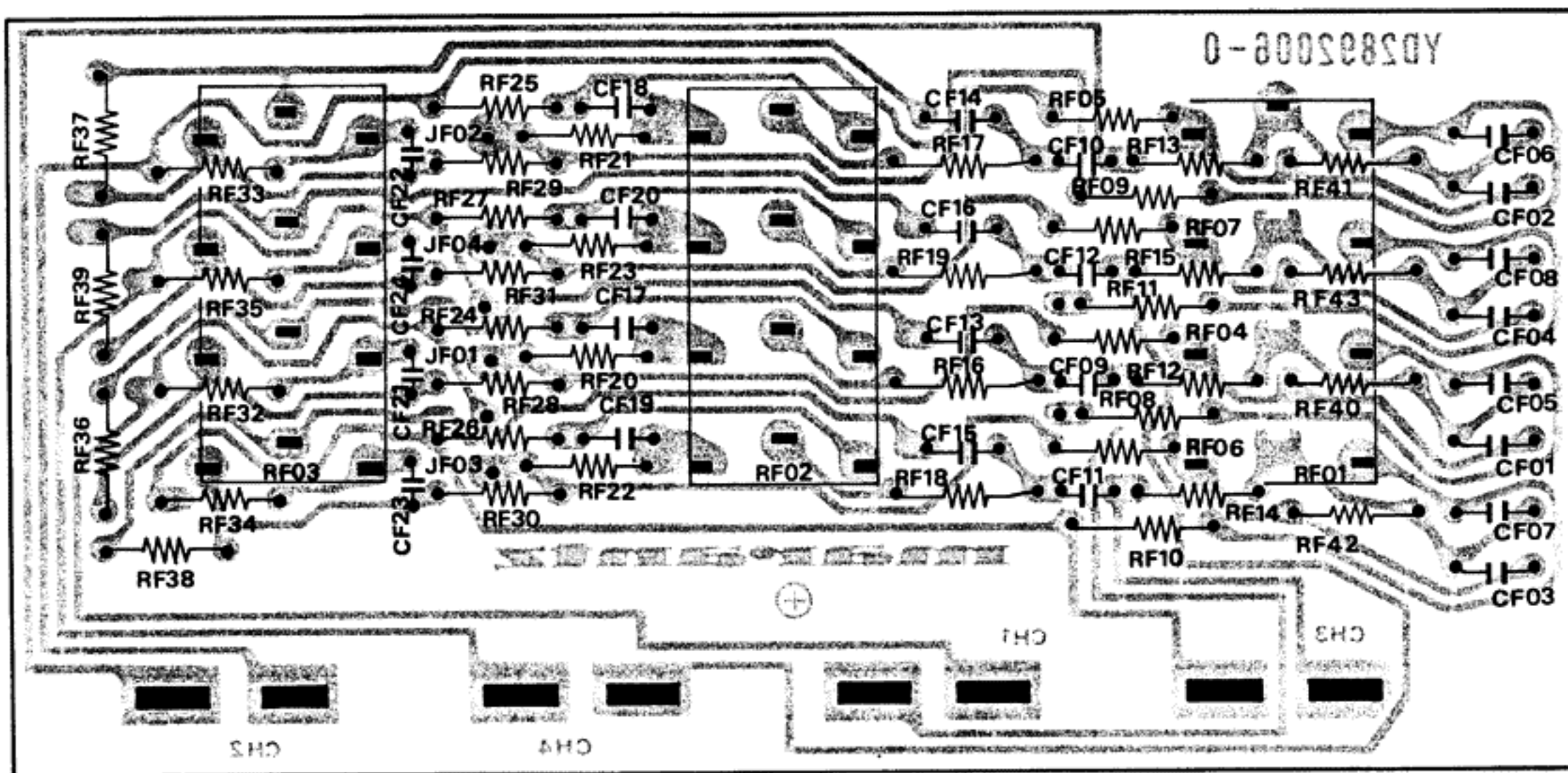
Figure 20. Tone Control Unit Assembly PF01 Component Locations
