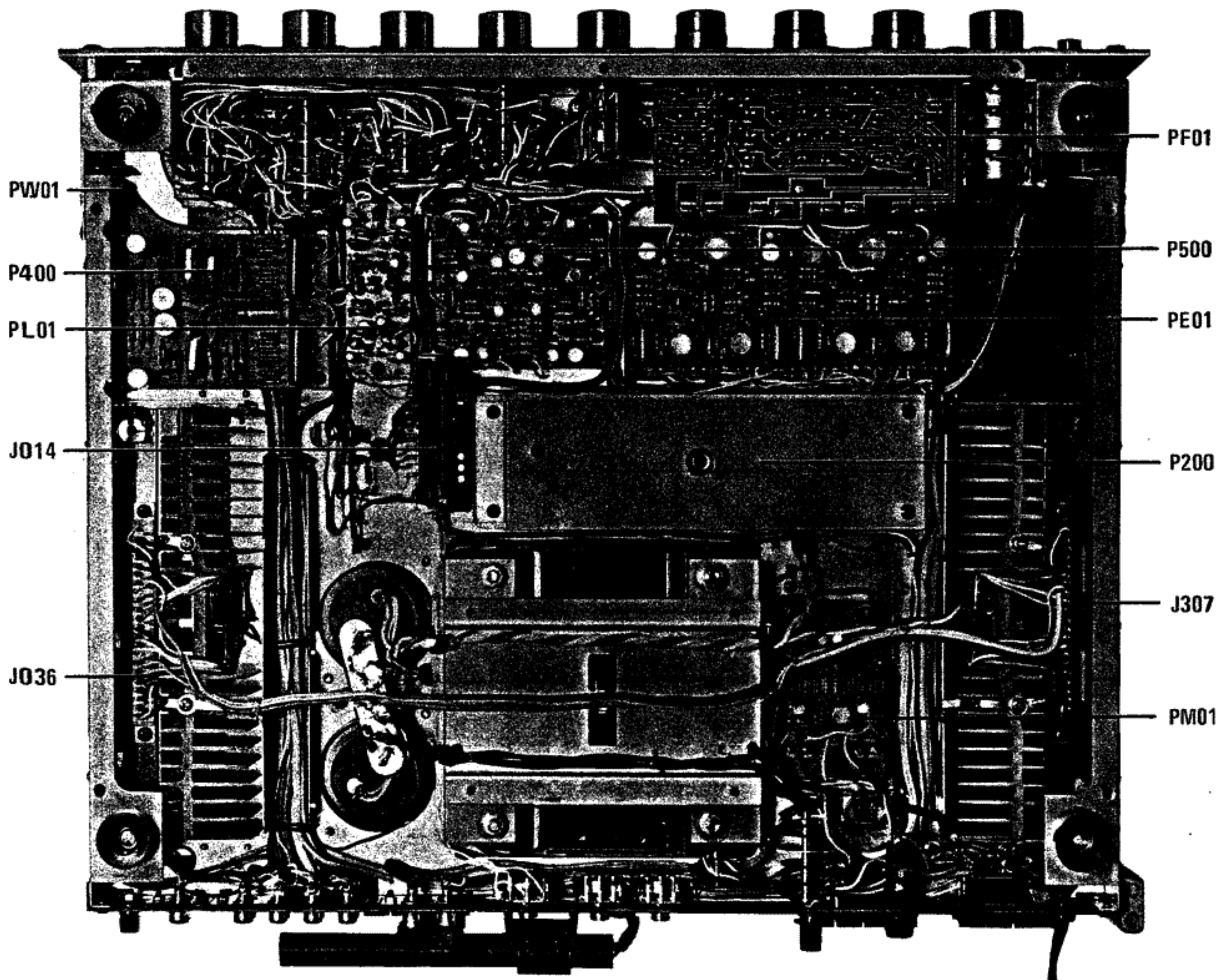
Figure 5. Main Chassis Component Locations (Bottom View)
