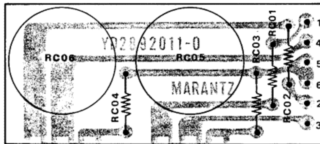
Figure 17. FM Cal. Assembly PC01 Component Locations
