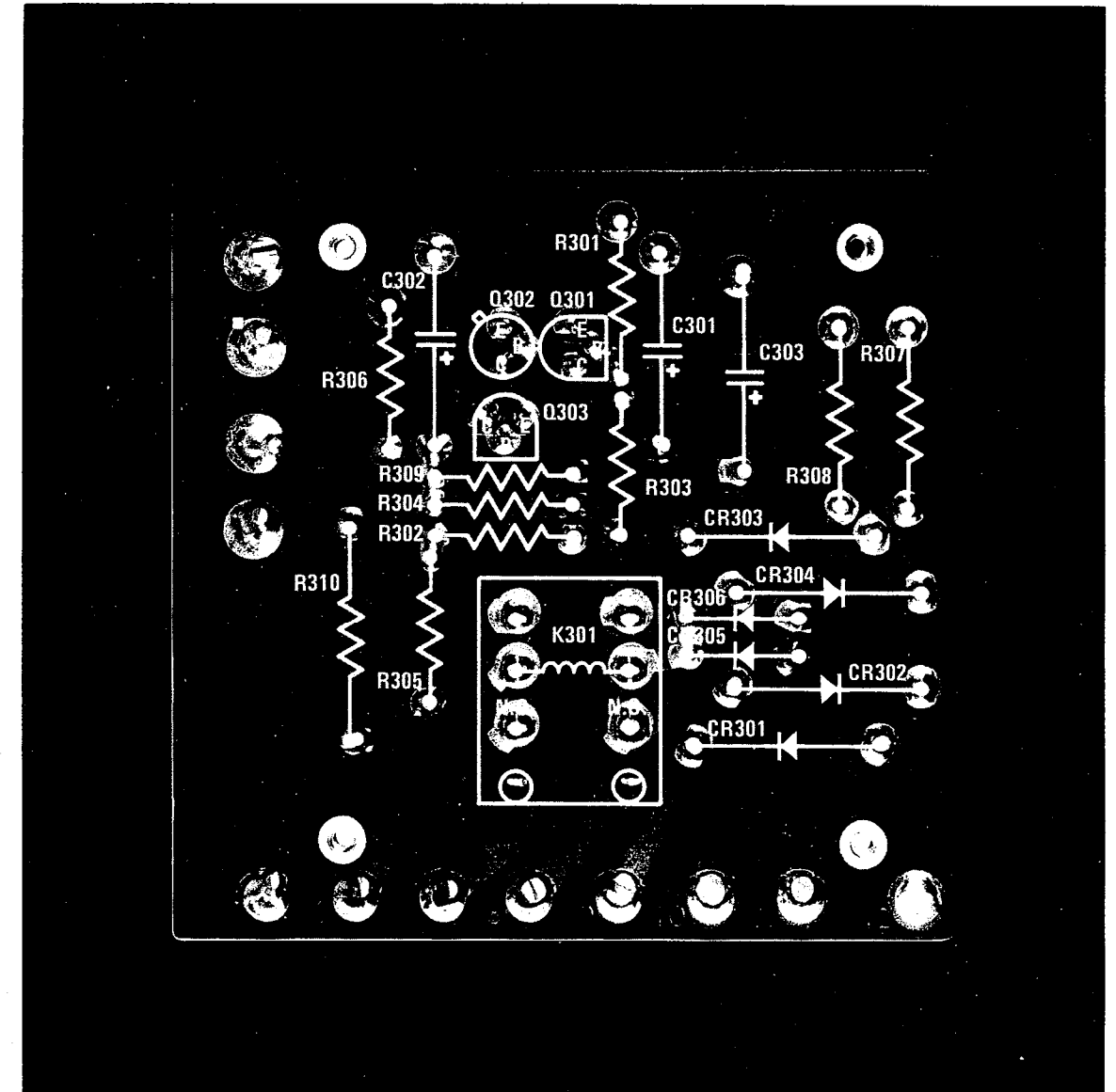
FIGURE 10. RECTIFIER-RELAY BOARD, CIRCUIT SIDE
