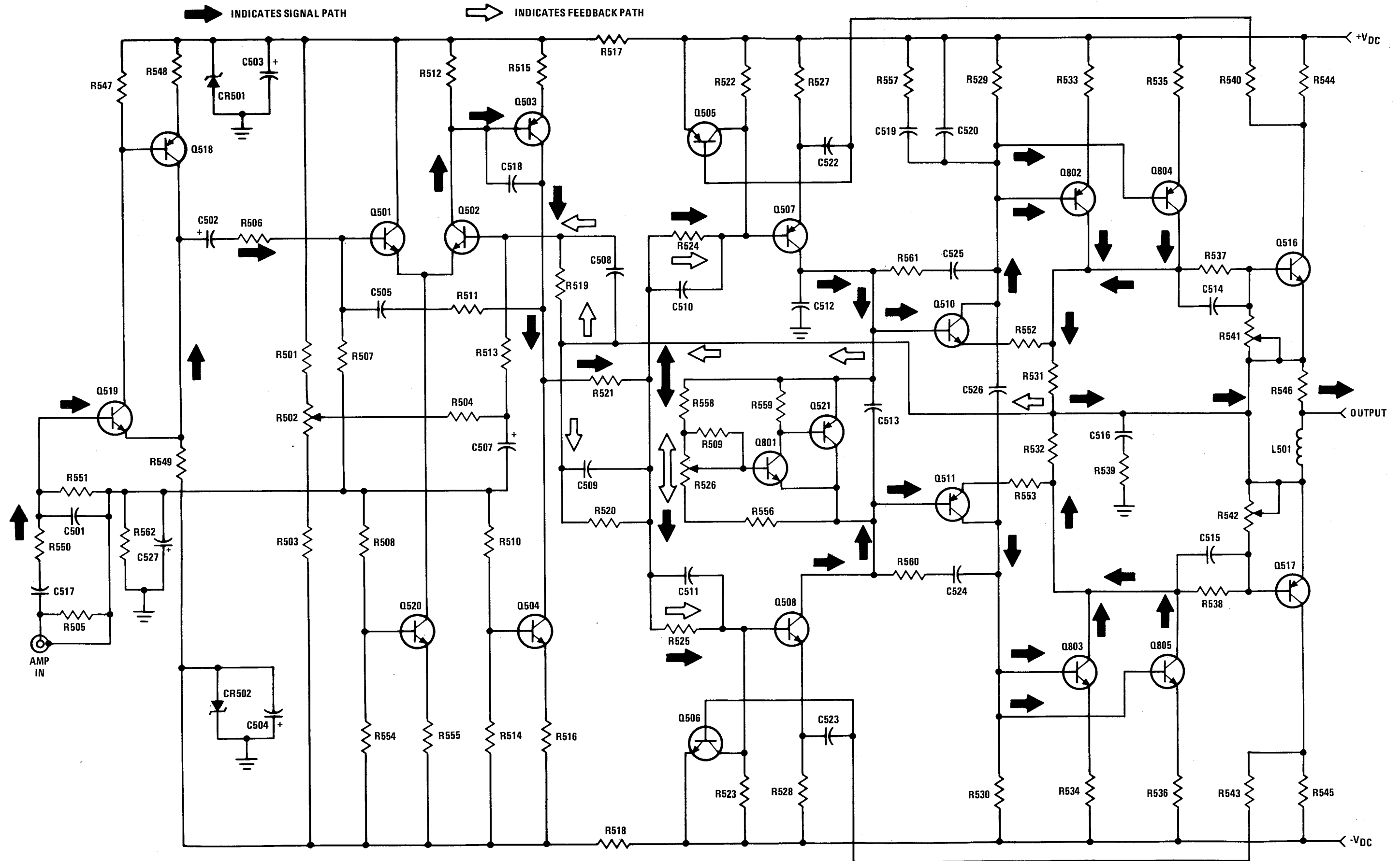
FIGURE 1. Amplifier Simplified Schematic
