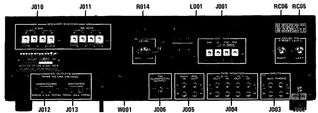
Figure 26. Rear Panel Adjustments and Component Locations
