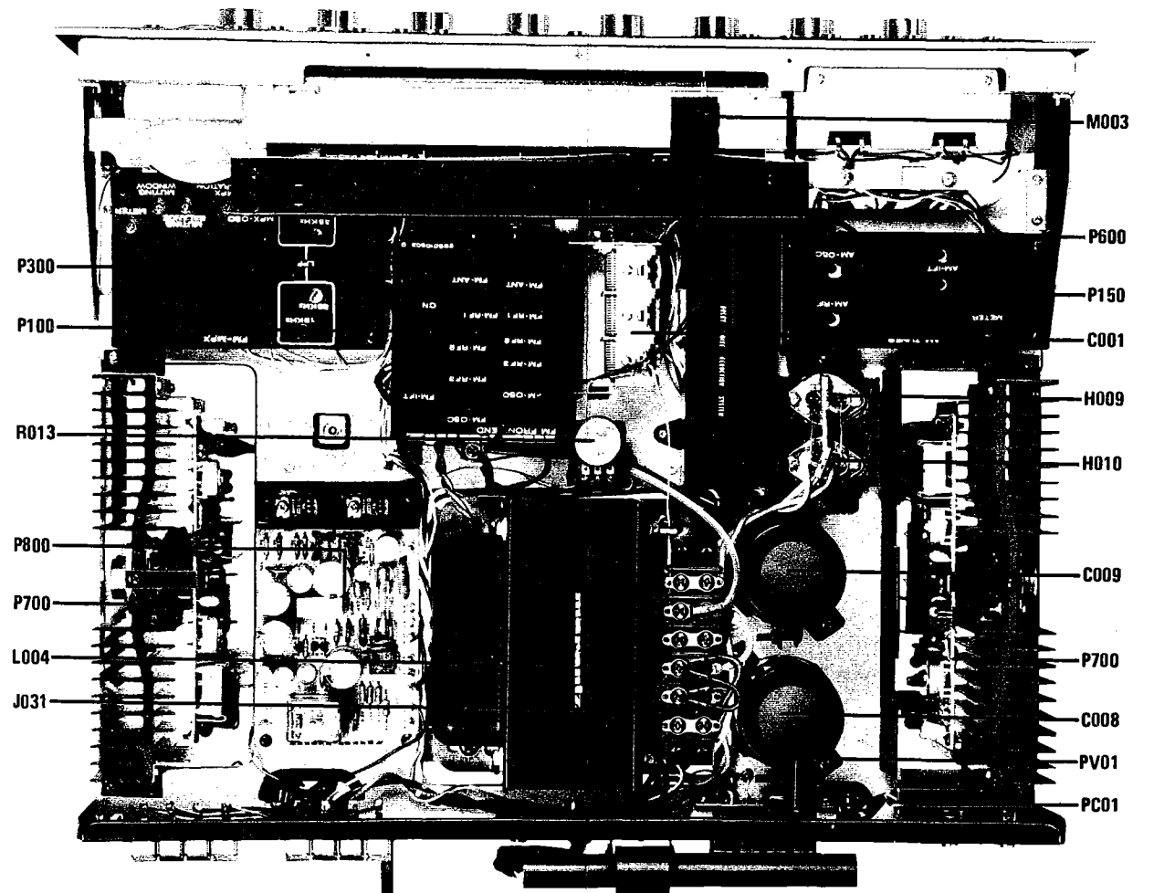
Figure 27. Main Chassis Component Locations (Top View)
