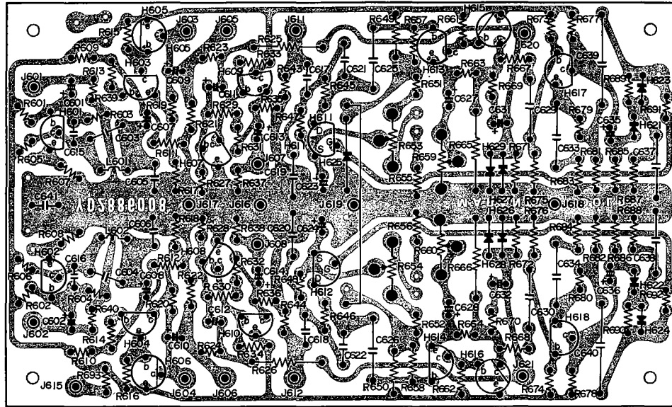
Figure 12. Dolby Unit Assembly P600 Component Locations
