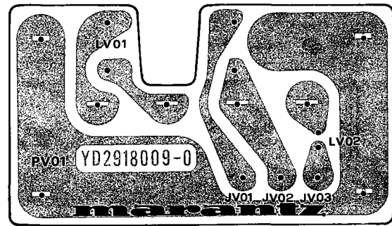
Figure 22. Antenna Terminal Assembly PV01 Component Locations
