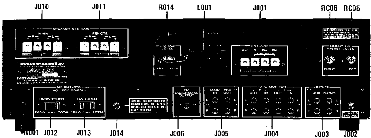
Figure 5. Rear Panel Adjustments and Component Locations
