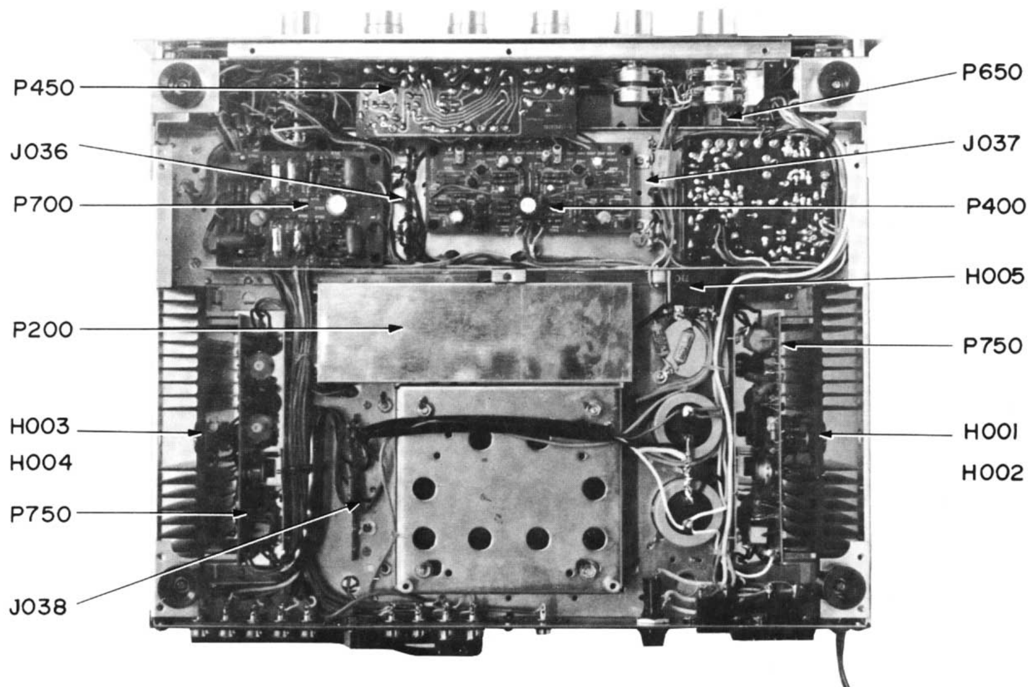
Figure 8 Main Chassis Component Locations (Bottom View)
