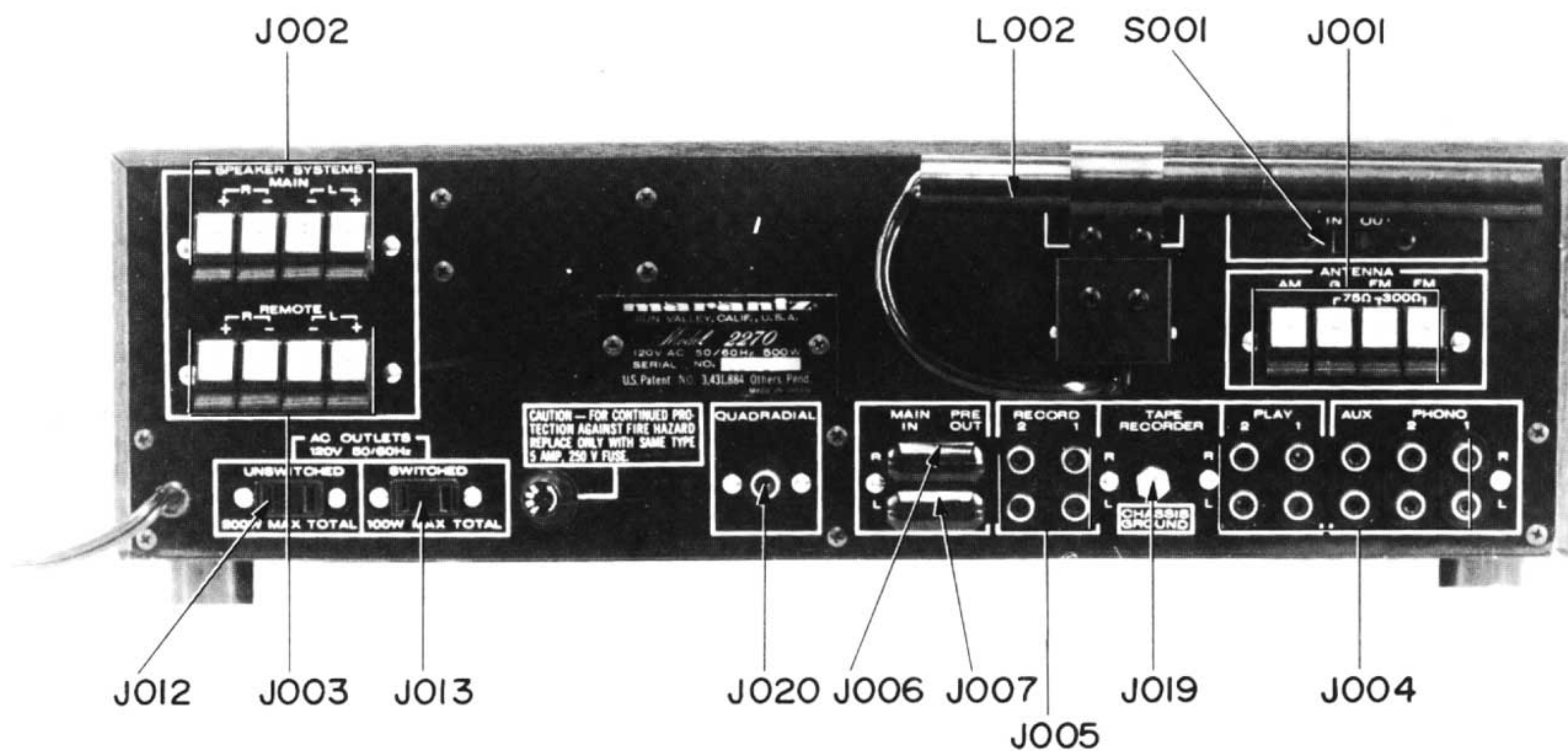
Figure 7 Rear Panel Adjustment and Component Locations
