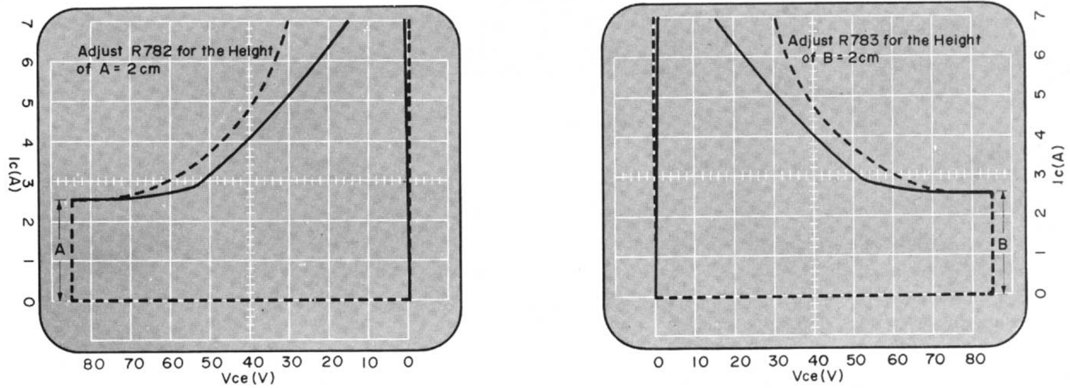
Figure 3 Lissajou Figure on Oscilloscope
