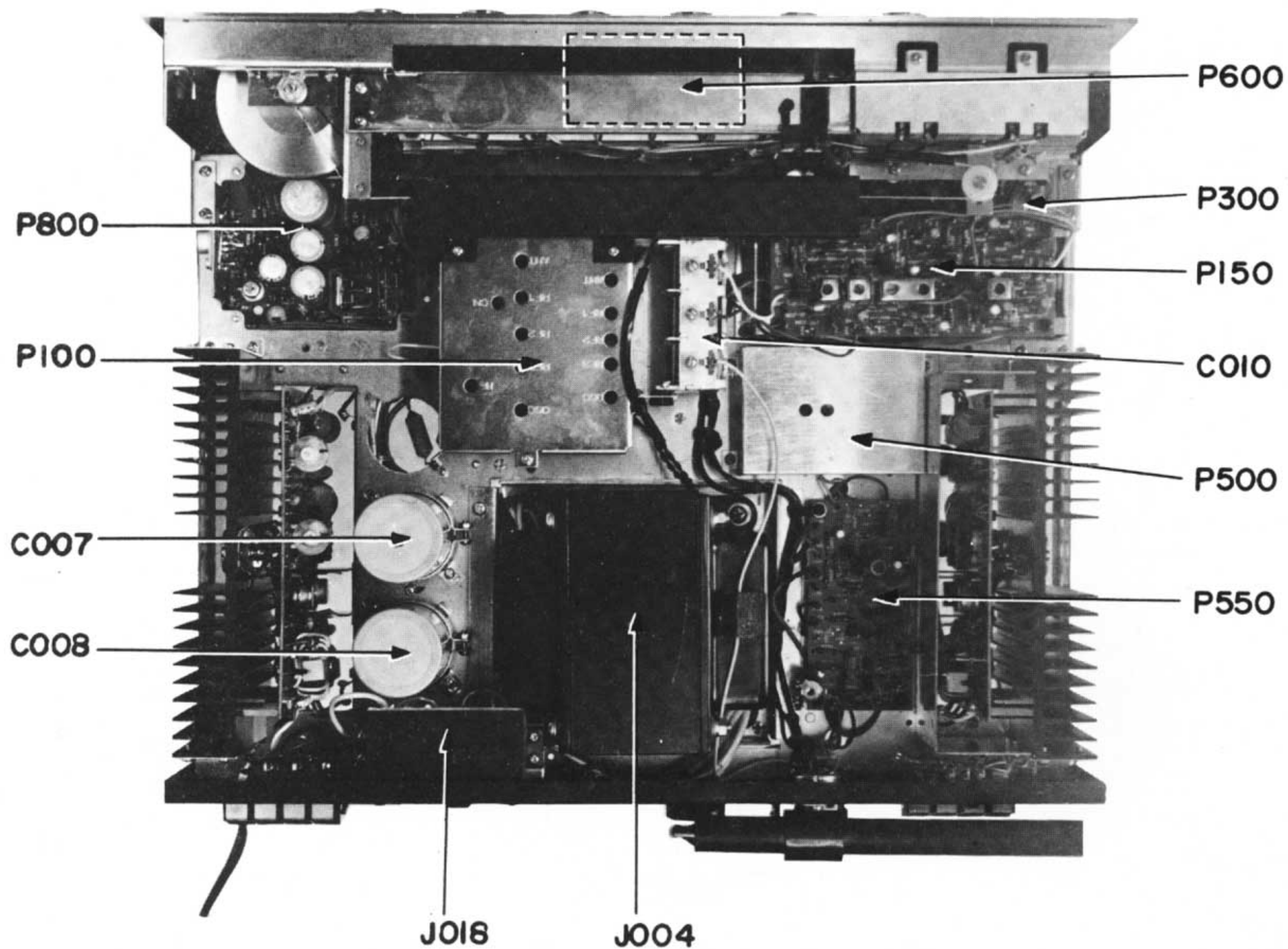
Figure 6 Main Chassis Component Locations (Top View)
