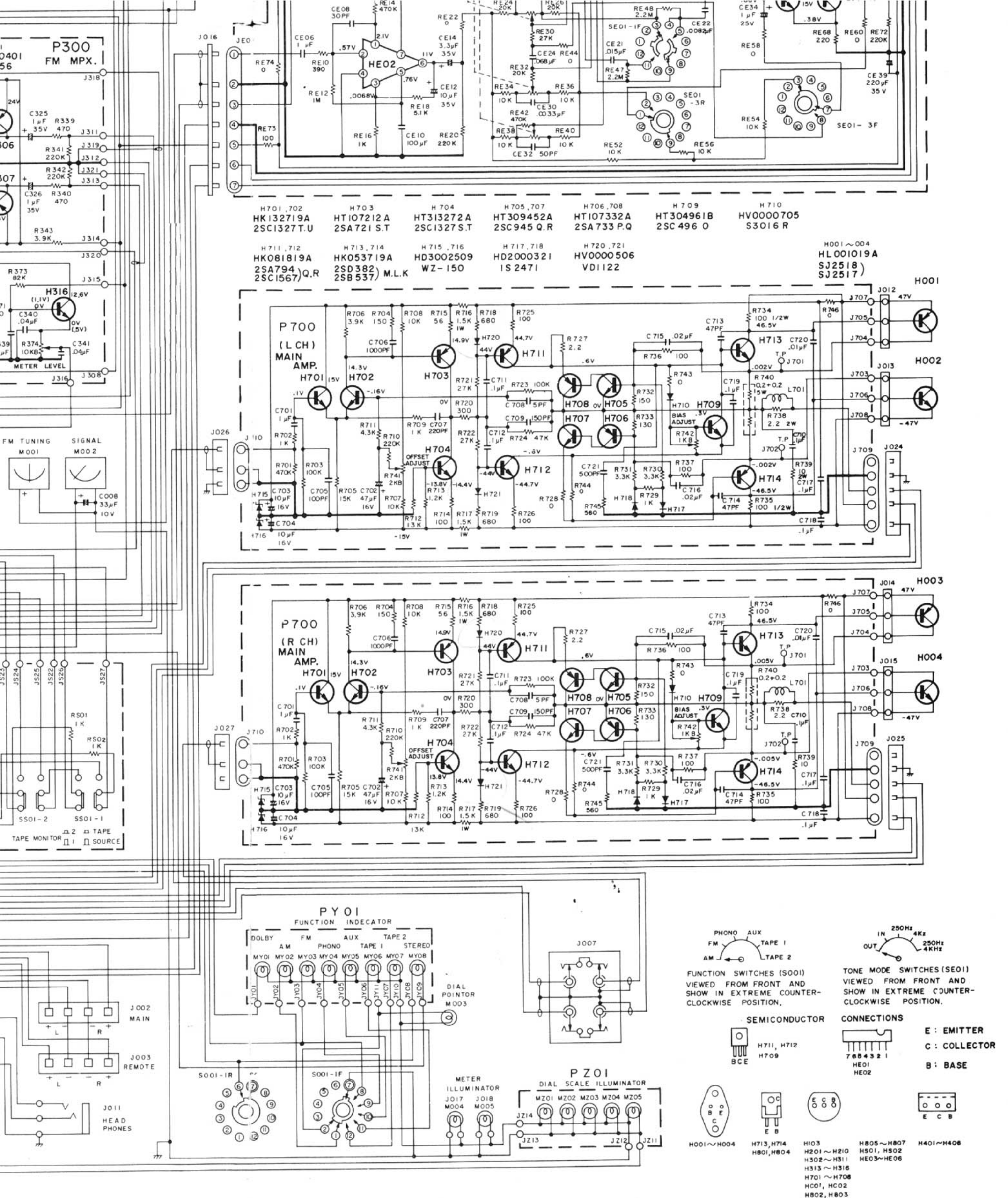
Figure 26. Schematic Diagram for U.S.A. Model
