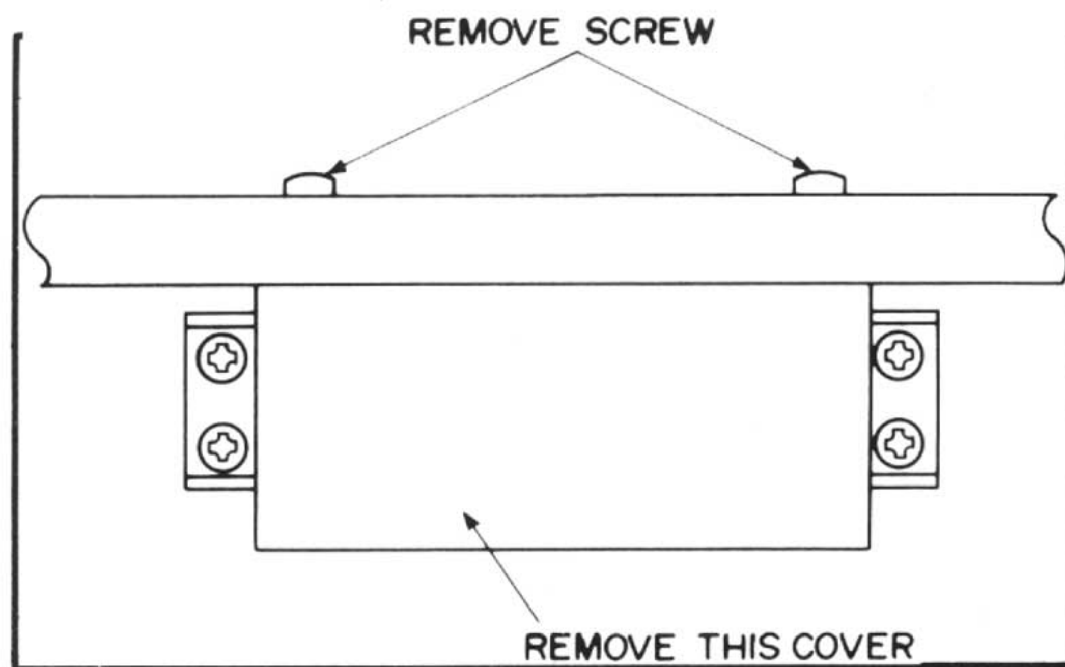
Figure 1 Remove the Terminal Cover
