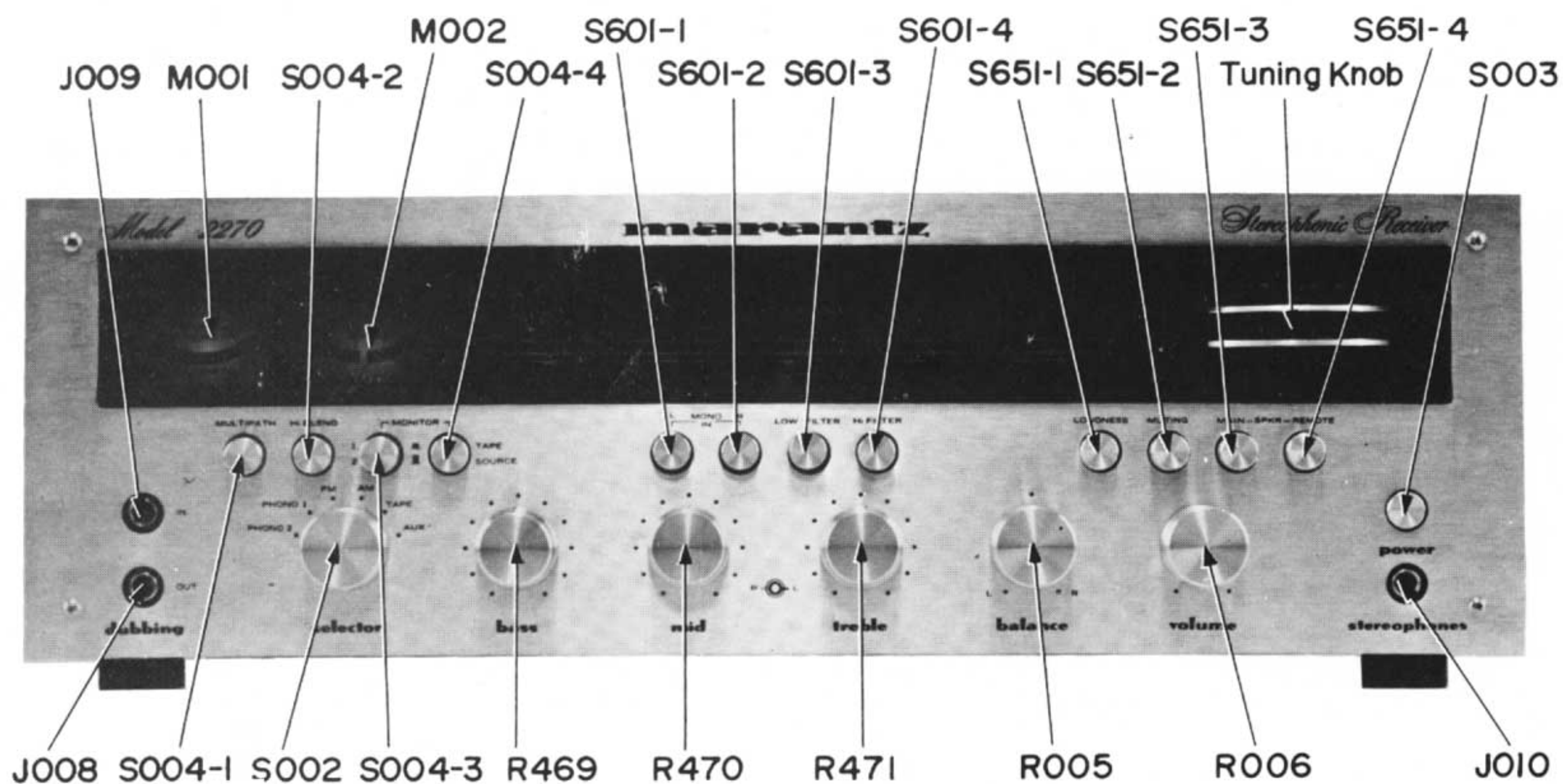
Figure 5 Front Panel Adjustment and Component Locations
