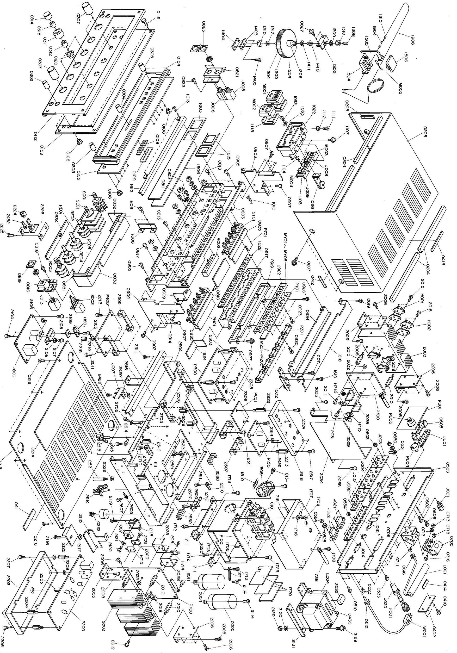
Figure 4. Exploded Mechanical Diagram
