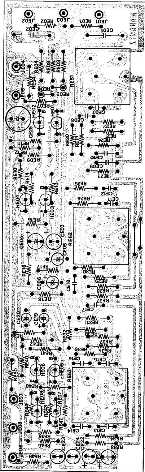
Figure 18. Pre-Tone Amplifier Assembly PE01 Component Locations
