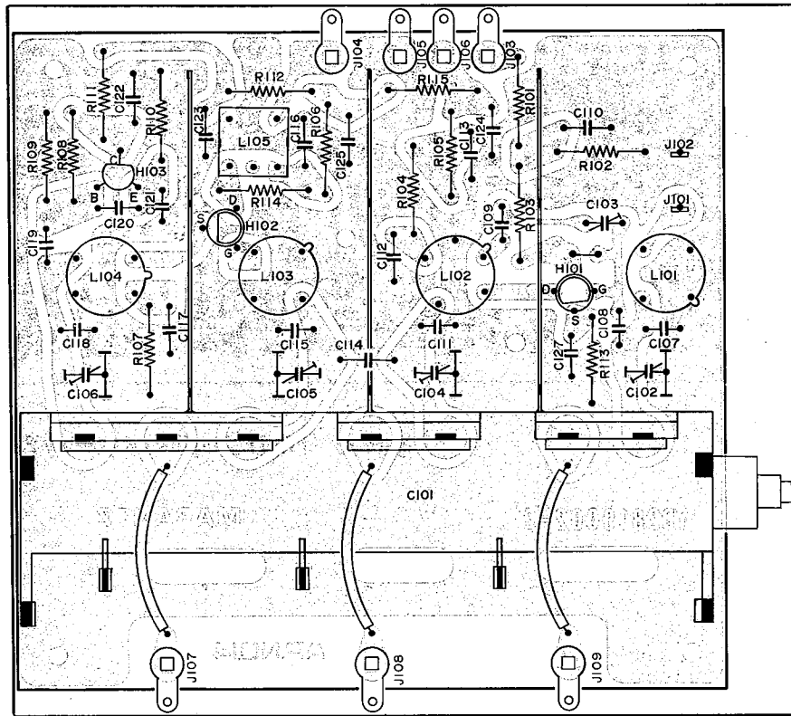
Figure 8. FM Front End Assembly P100 Component Locations
