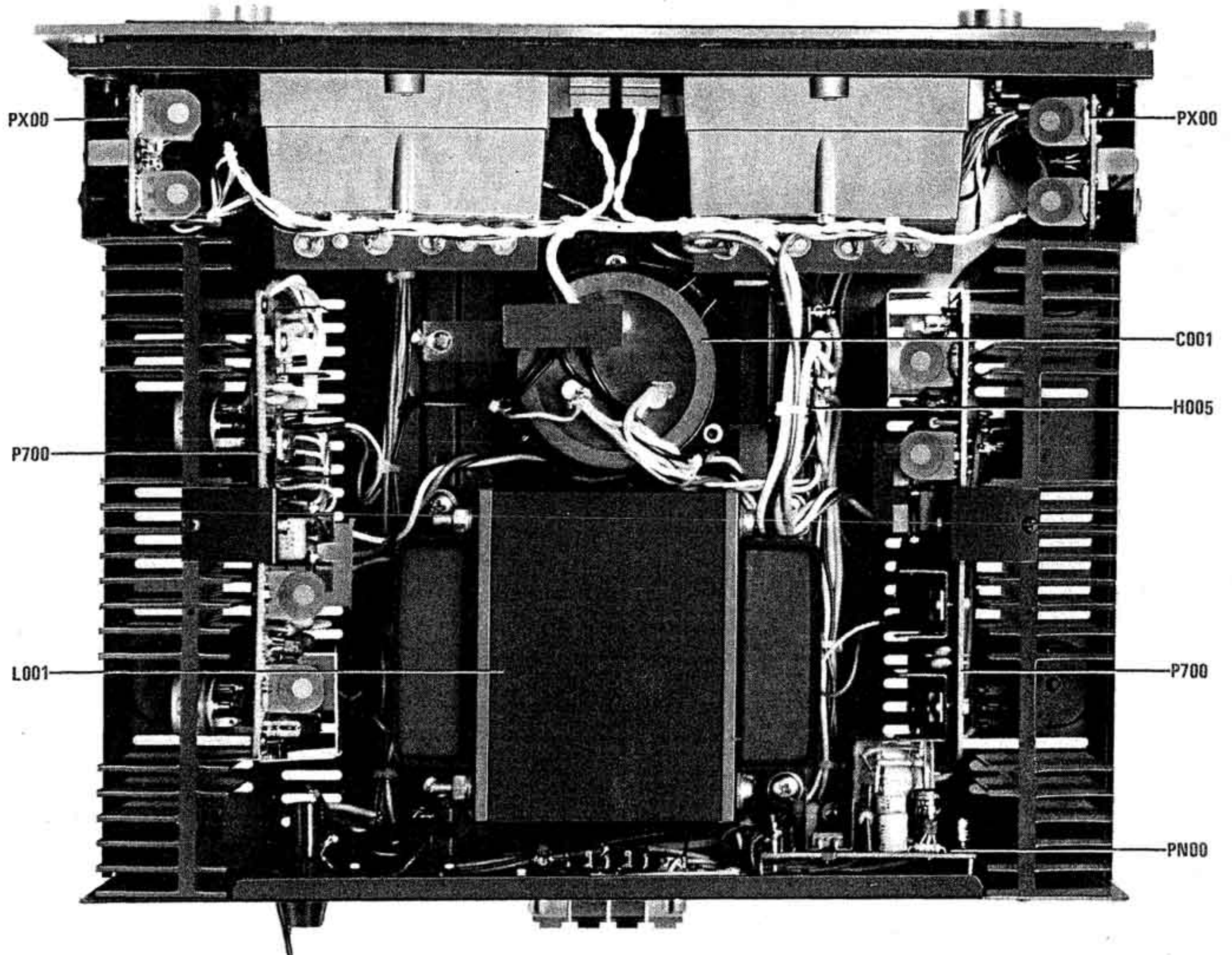
Figure 6. Main Chassis Component Locations (Top View)
