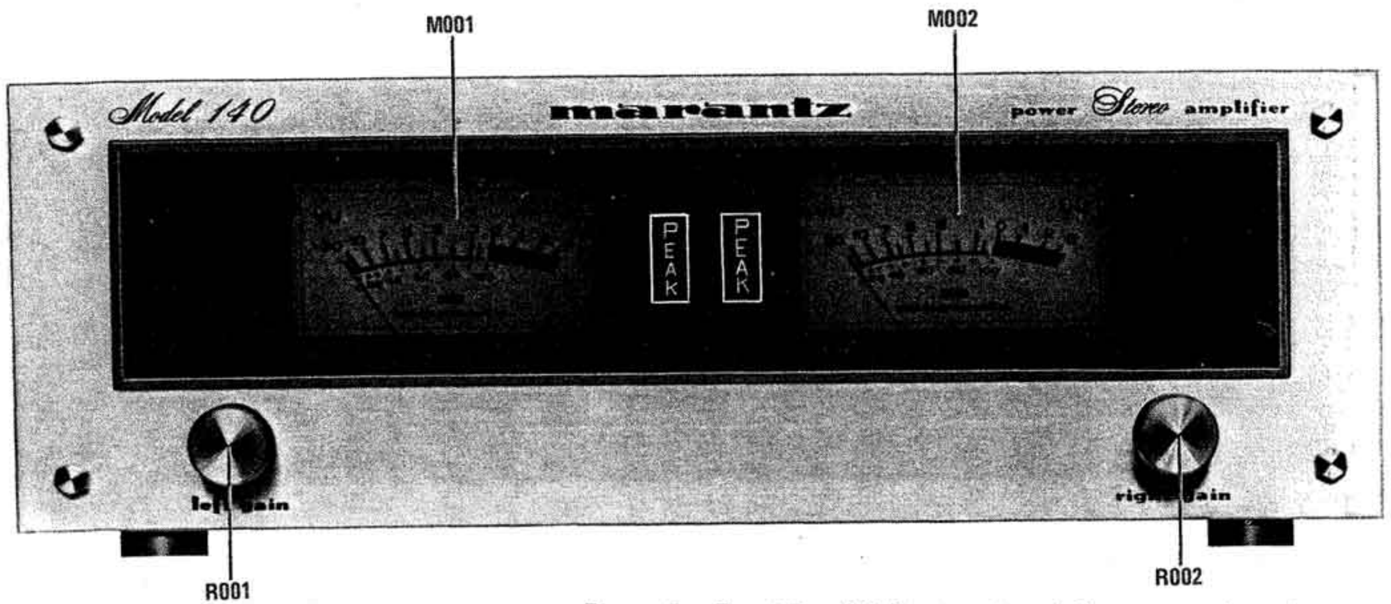
Figure 5. Front Panel Adjustment and Component Locations
