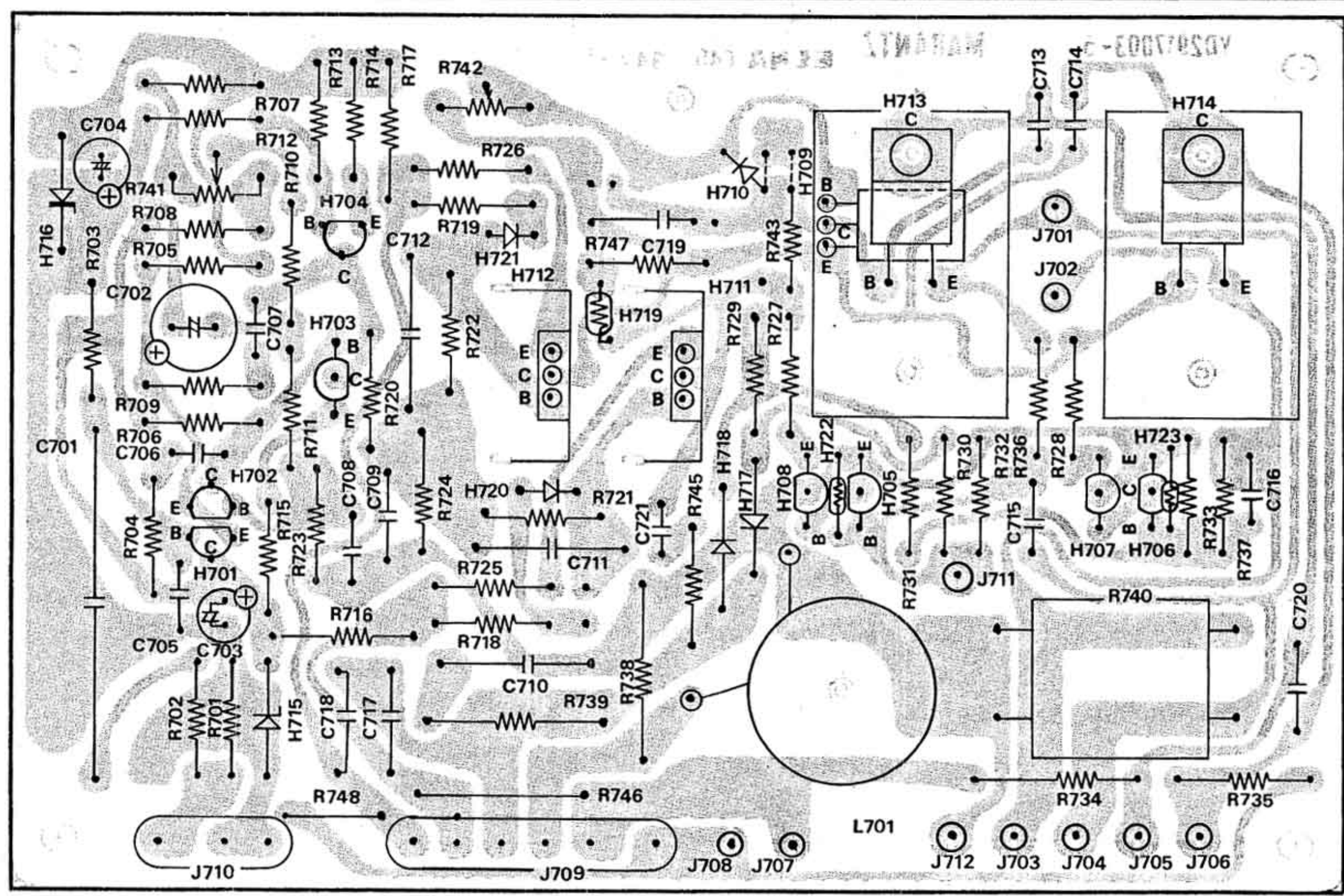
Figure 8. Main Amp. P700 Schematic Diagram and Component Locations
