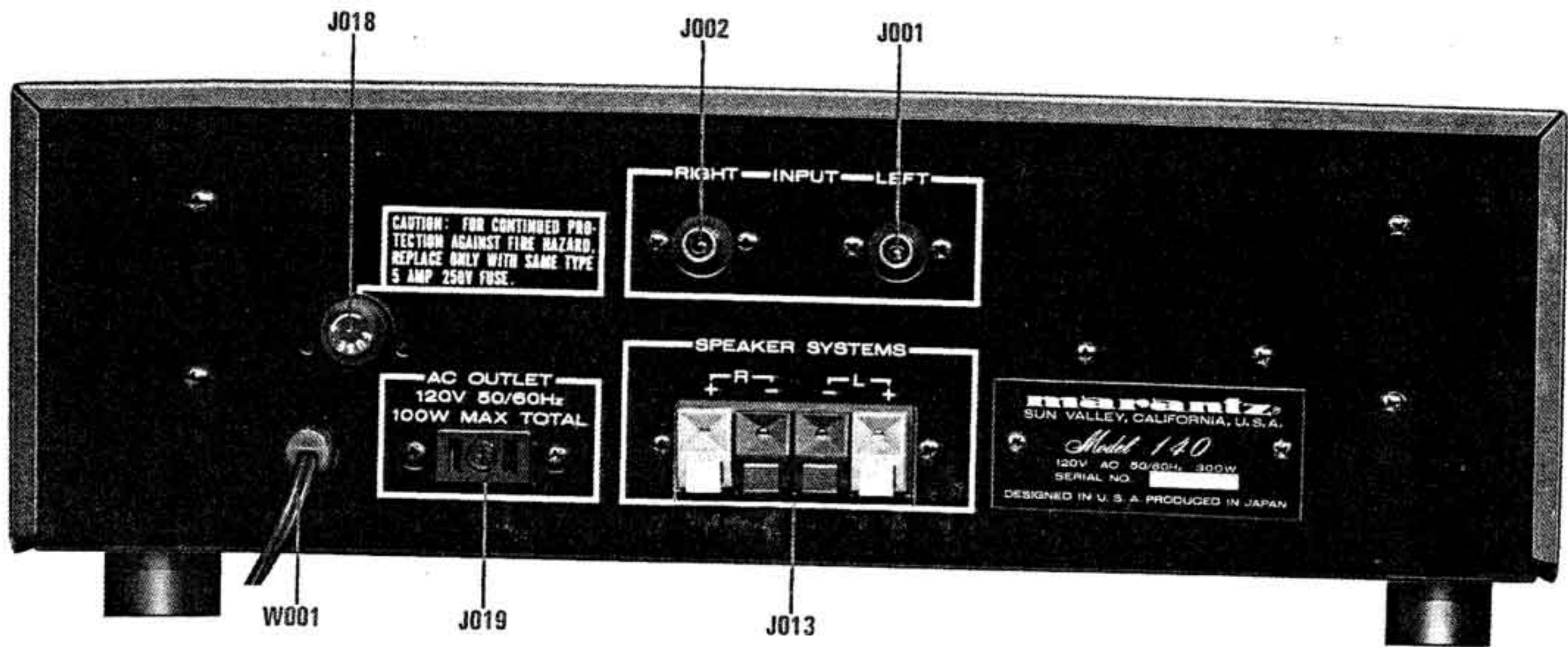
Figure 7. Rear Panel Jacks and Component Locations
