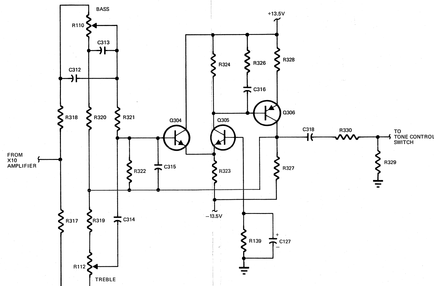
Figure 4. Tone Amplifier Simplified Schematic.
