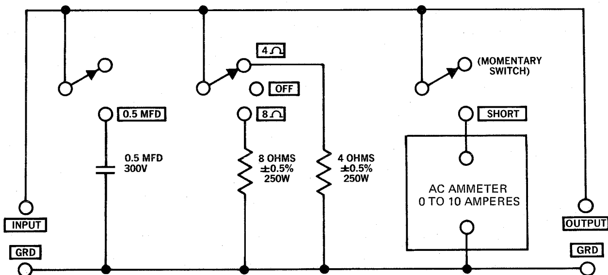
Figure 11. Amplifier Output Load Box Simplified Schematic
