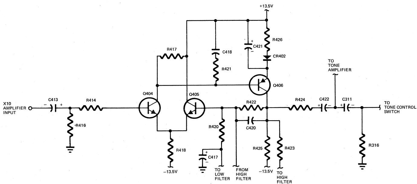
Figure 2. X10 Amplifier Simplified Schematic.
