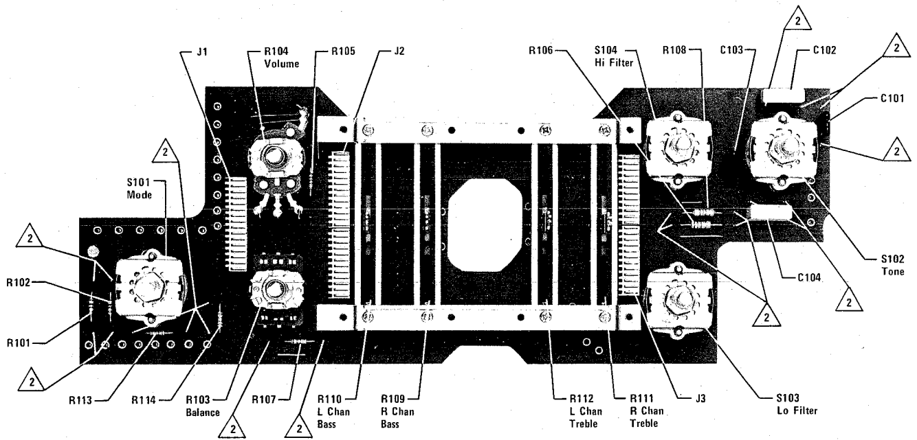
COMPONENT SIDE
