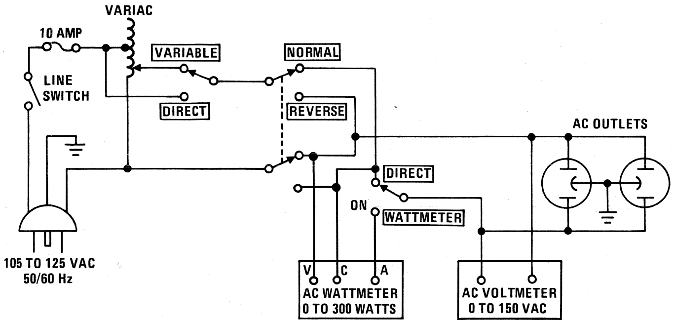
Figure 10. AC Power Control Box Simplified Schematic
