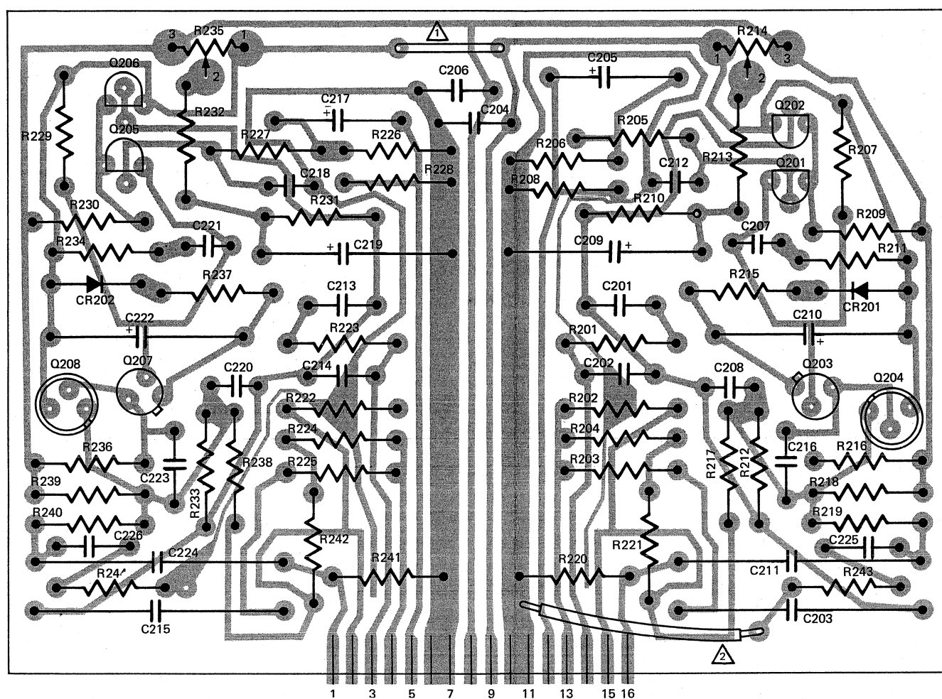
Figure 14. Phono Amplifier Board – A2 Component Assembly Diagram
