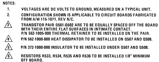
Figure 17. Power Amplifier Board – A5/A6 Component Assembly Diagram
