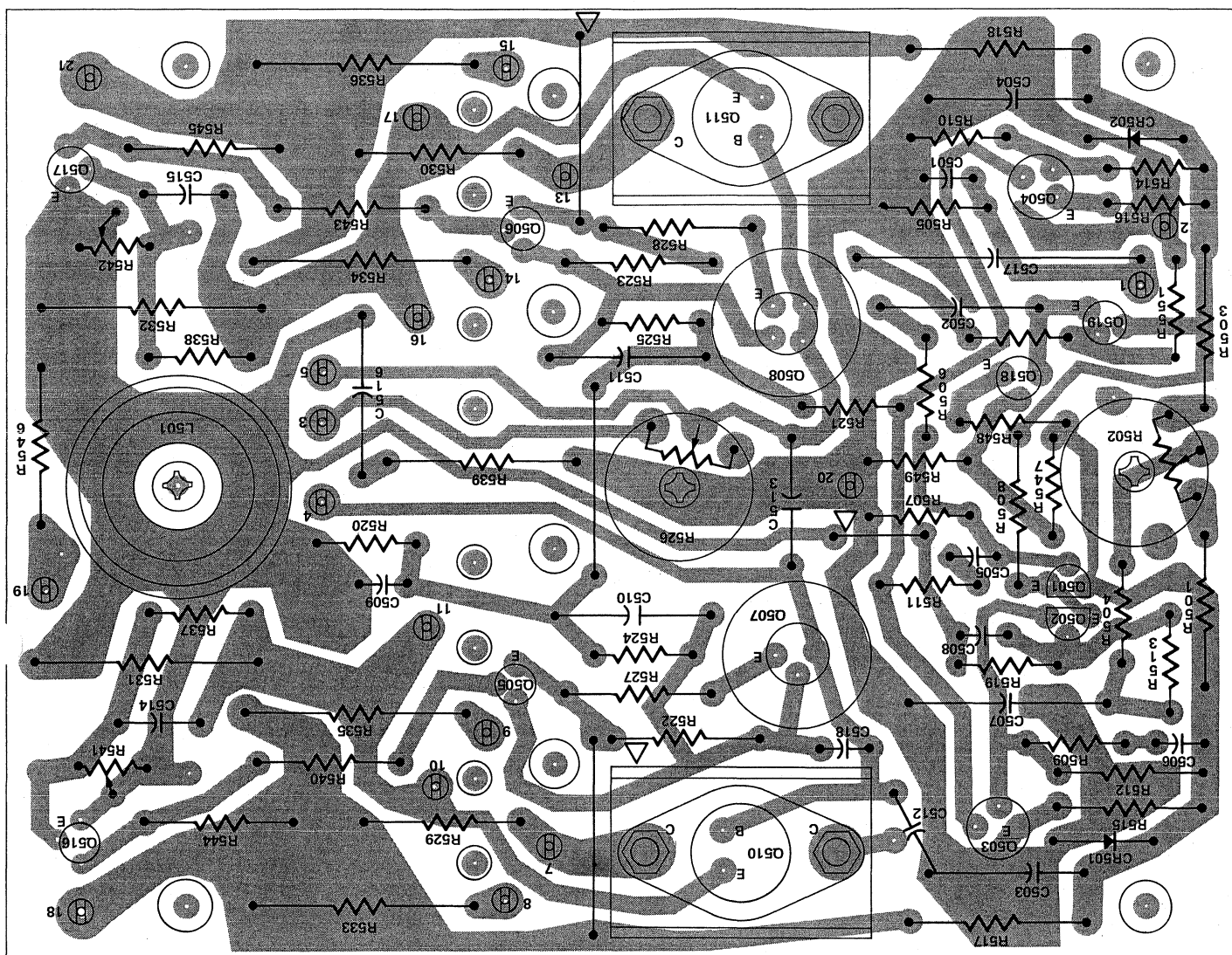
Figure 17. Power Amplifier Board – A5/A6 Component Assembly Diagram
