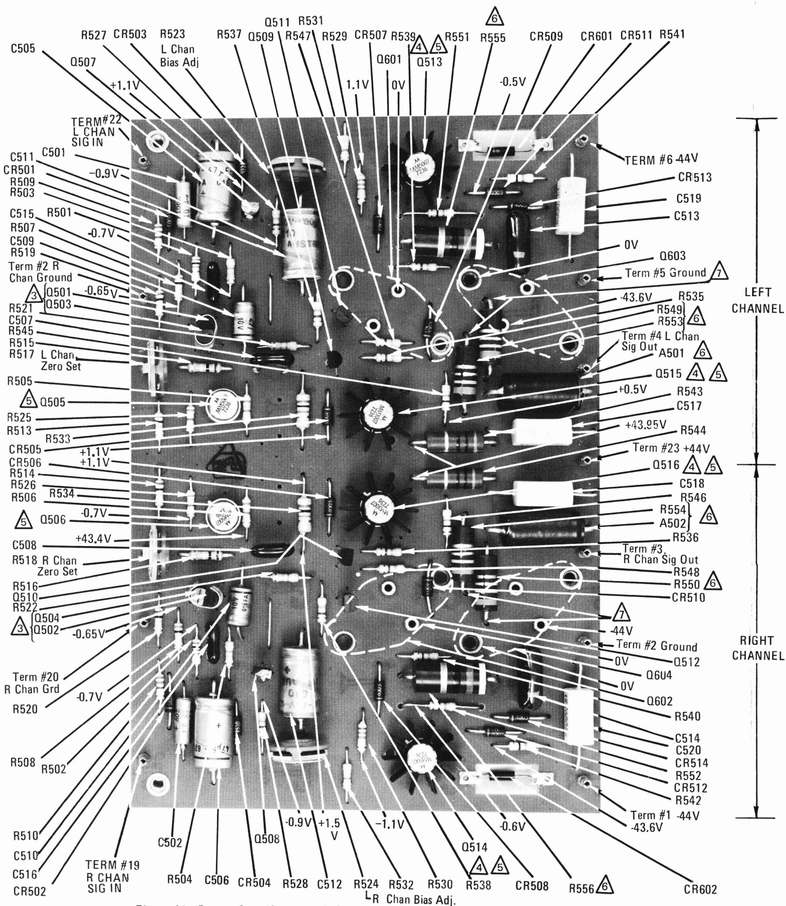
Figure 14. Power Amplifier Board Assembly
