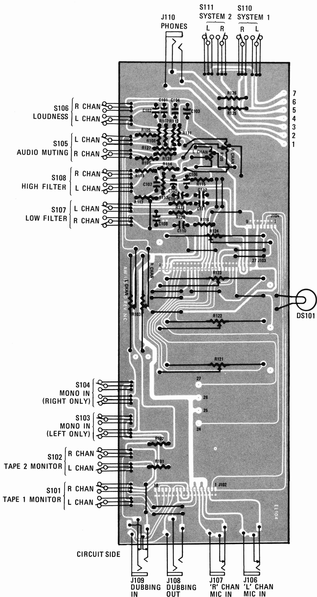
Figure 12. Interconnection Board Assembly (Cont.)
