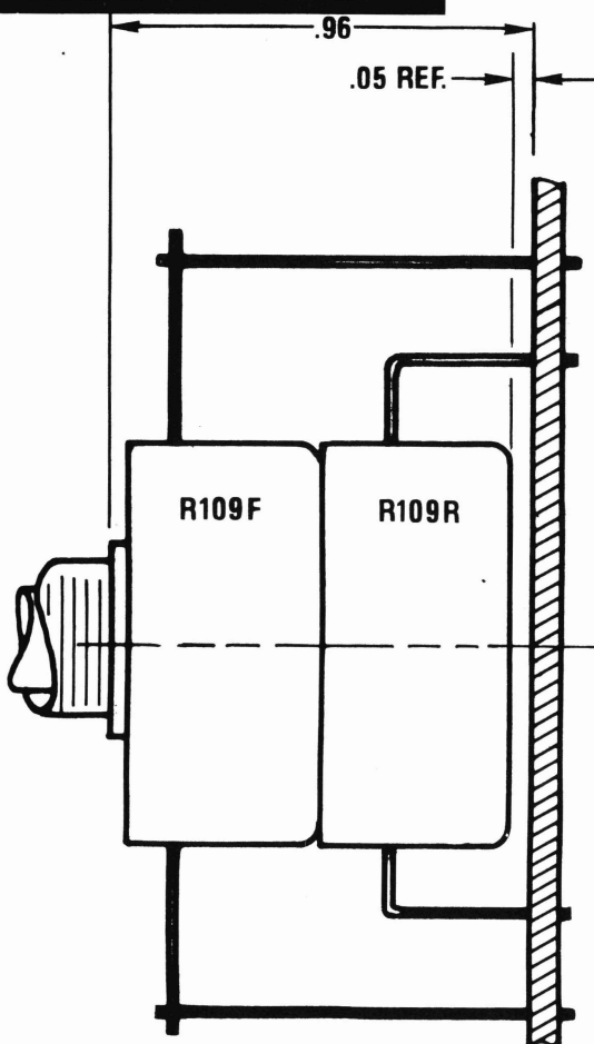
DETAIL B
