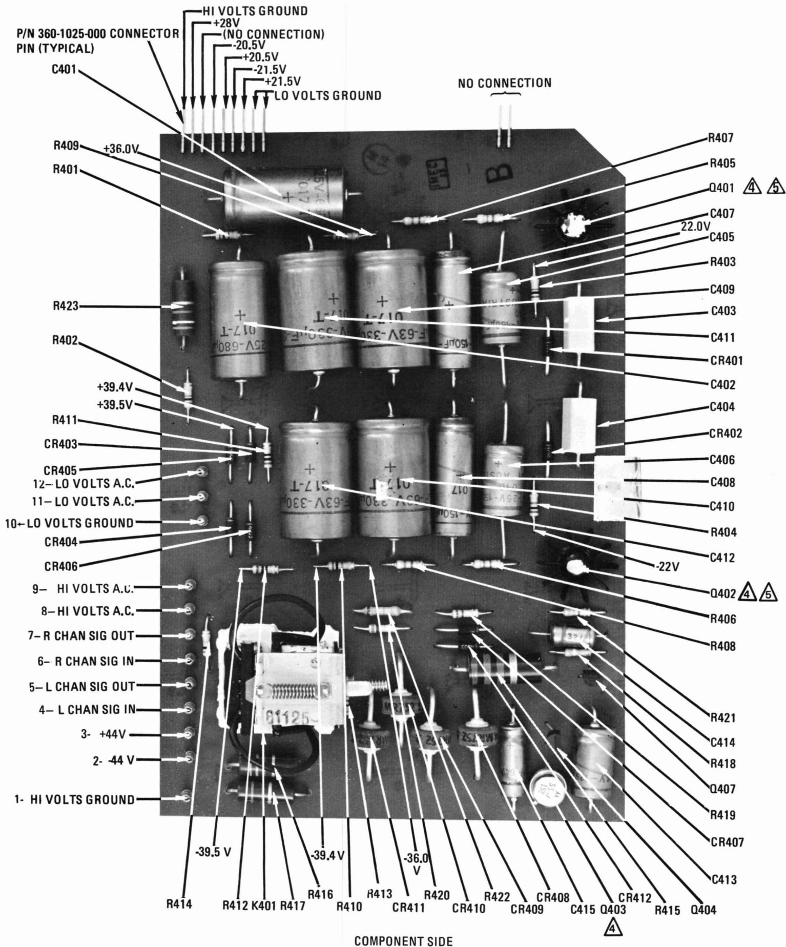
Figure 16. Power Supply Board Assembly
