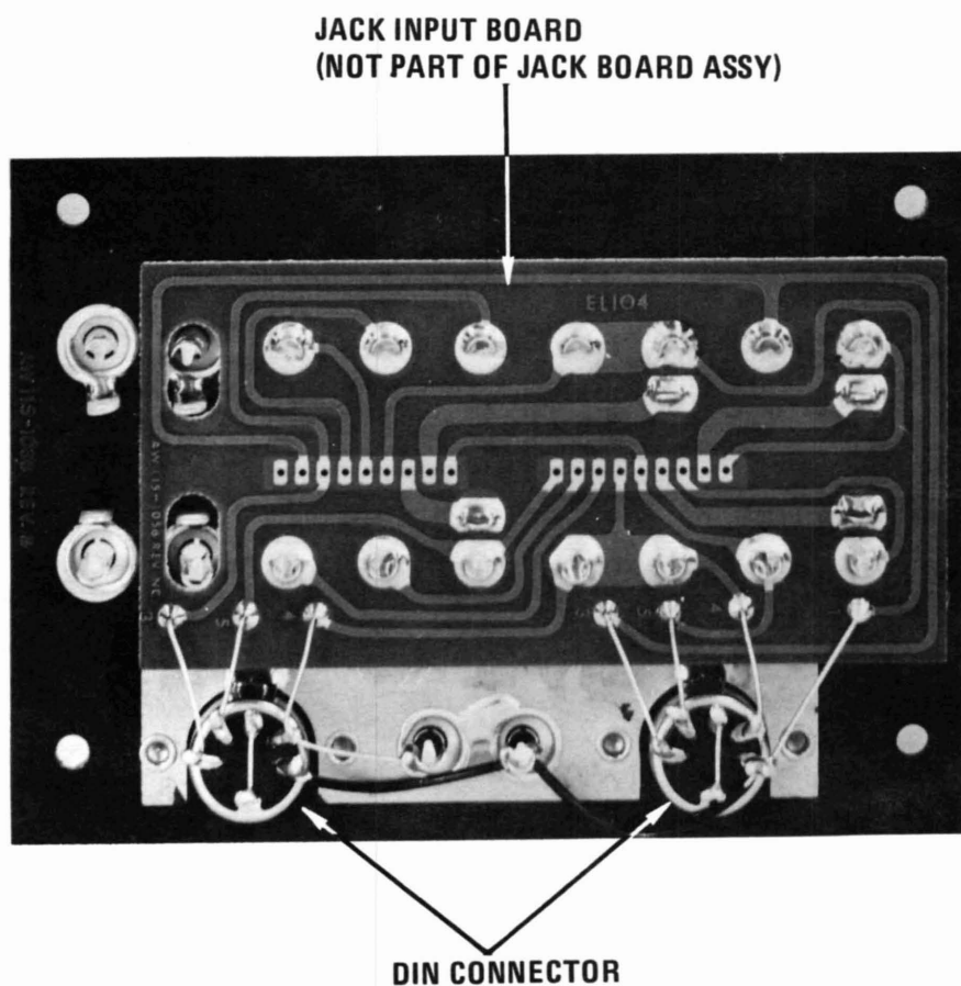
Figure 10. Jack Panel Board Assembly
