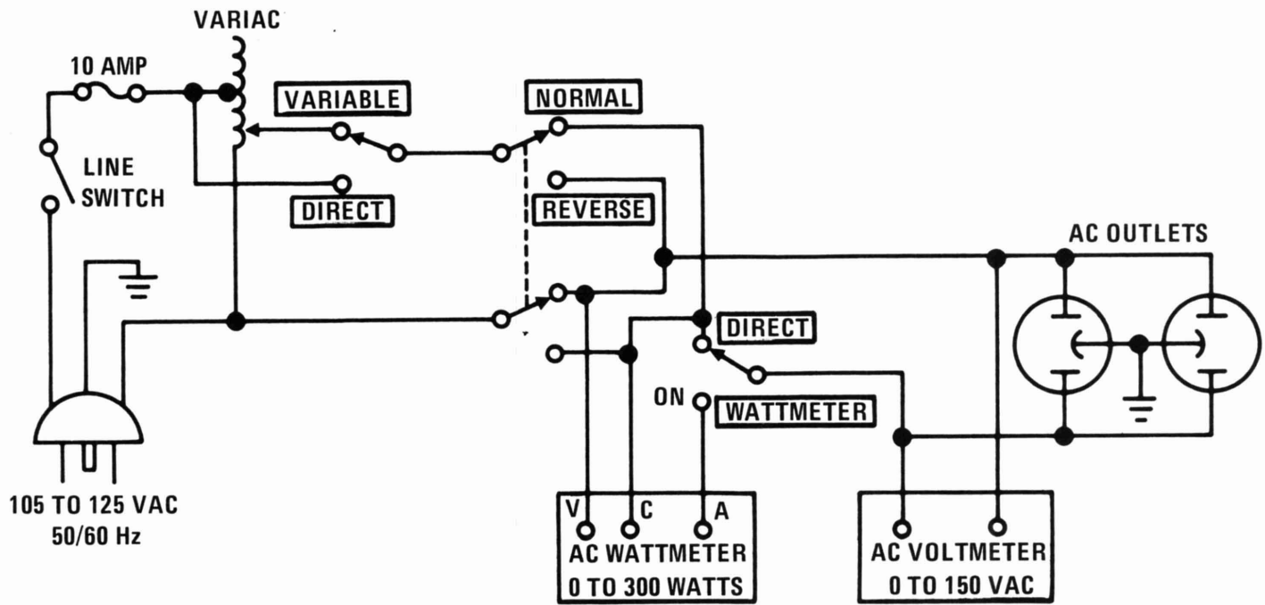
Figure 3. AC Power Control Box Schematic
