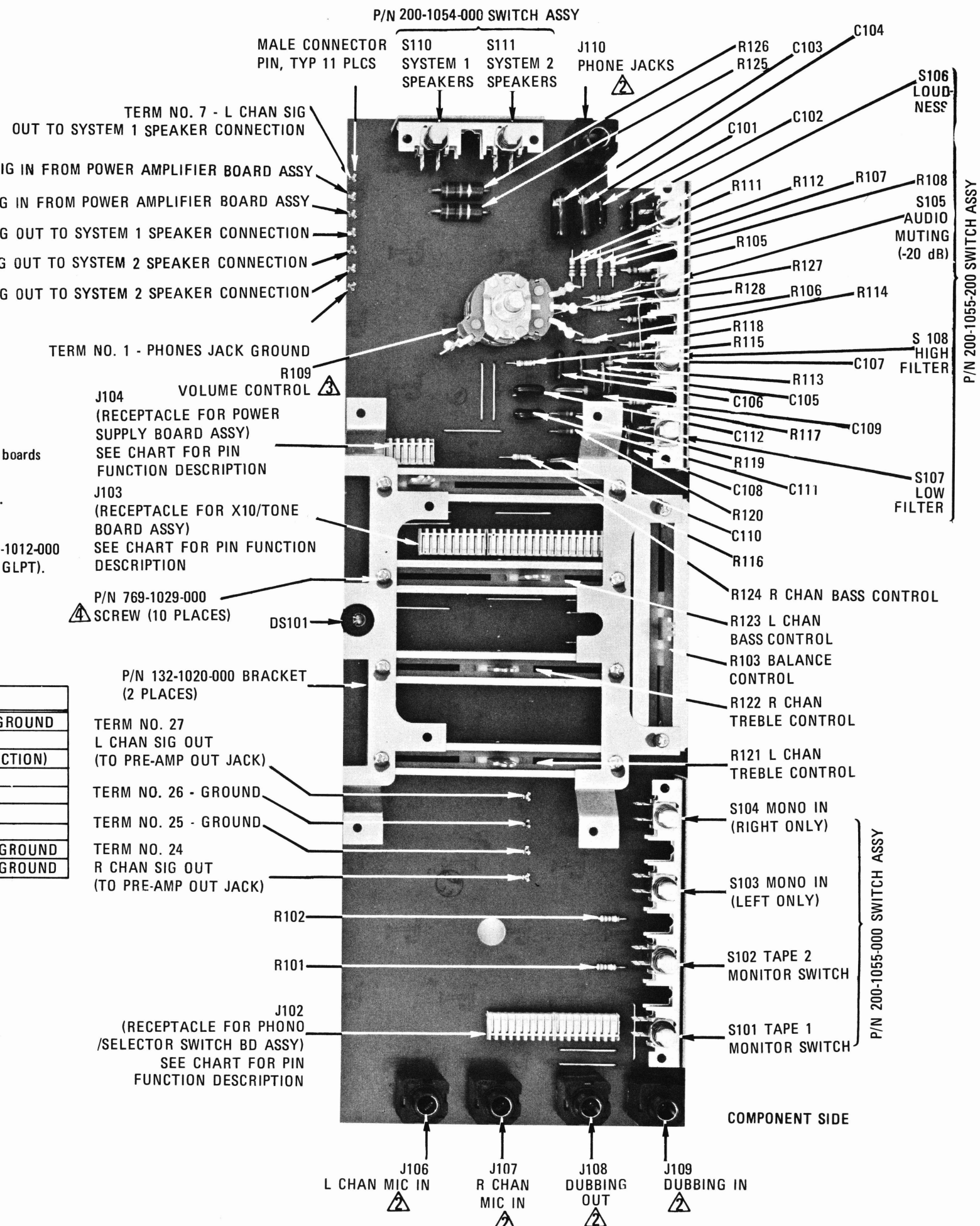
Figure 12. Interconnection Board Assembly
