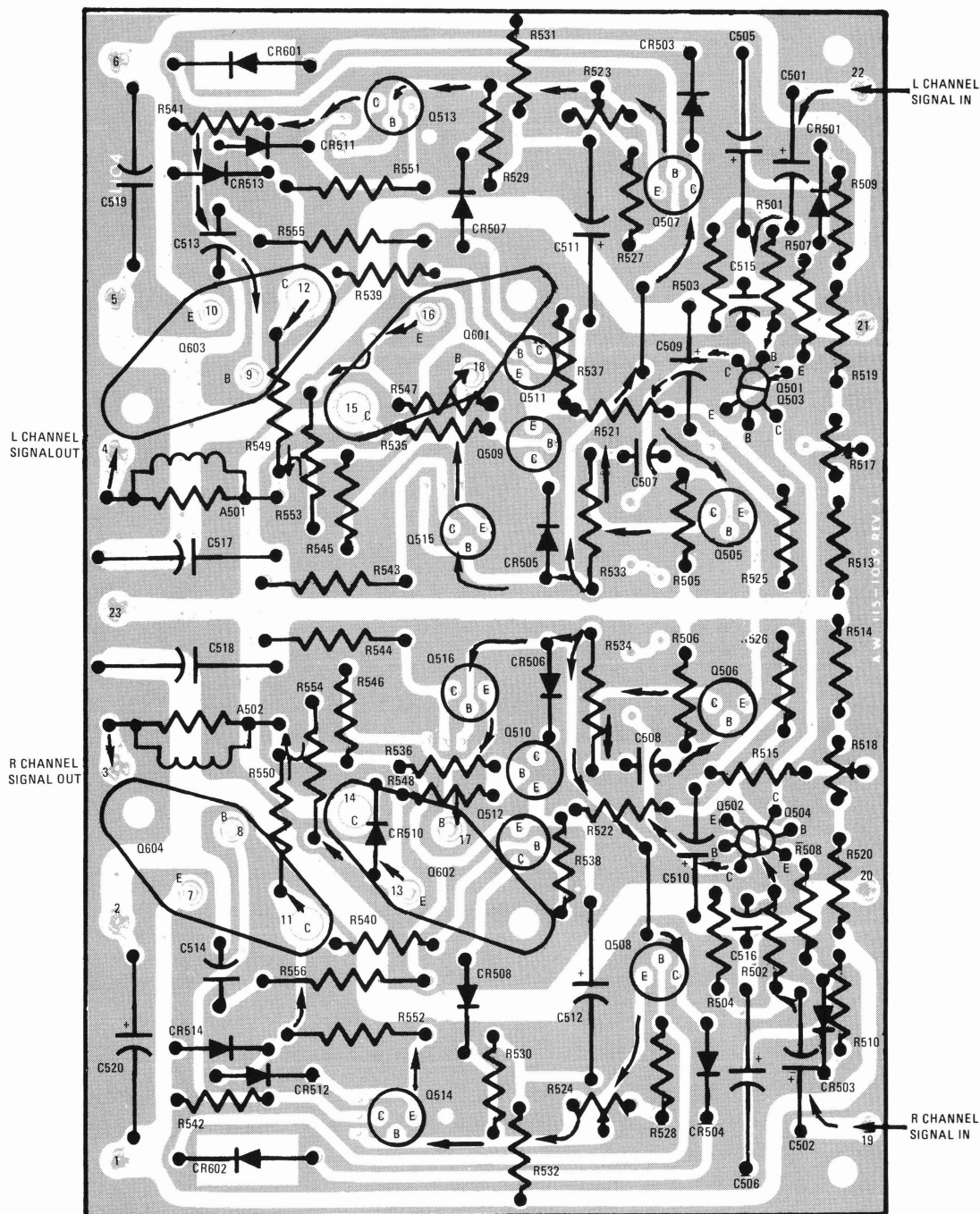
CIRCUIT SIDE
