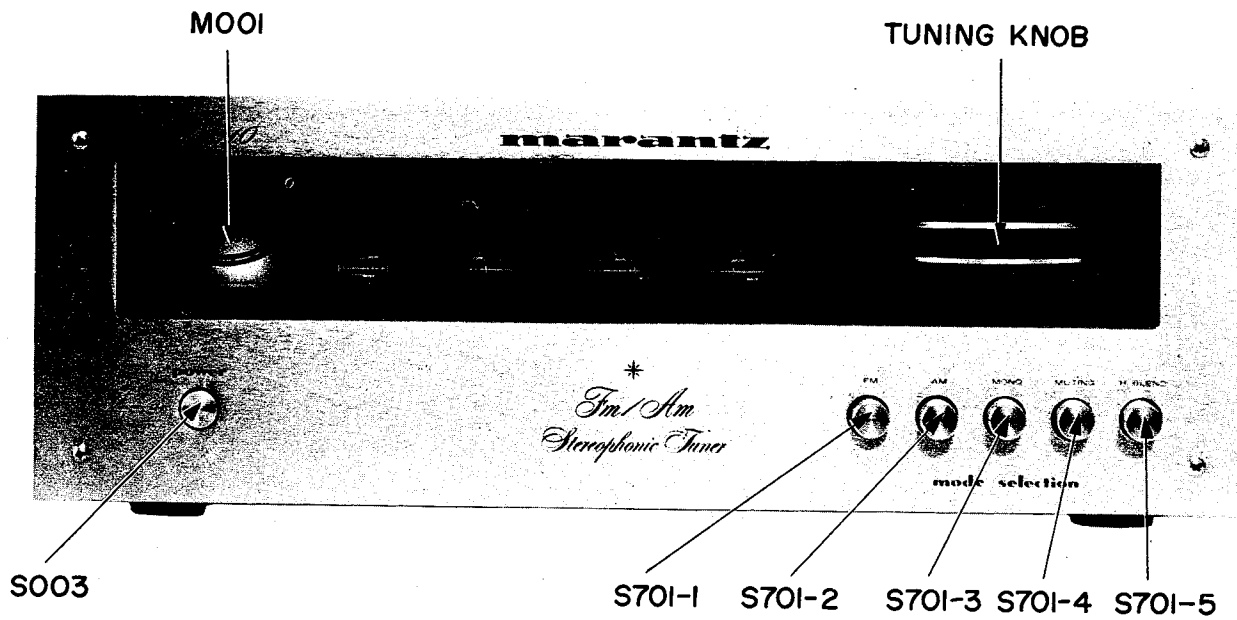
Figure 4. Front Panel Adjustment and Component Locations
