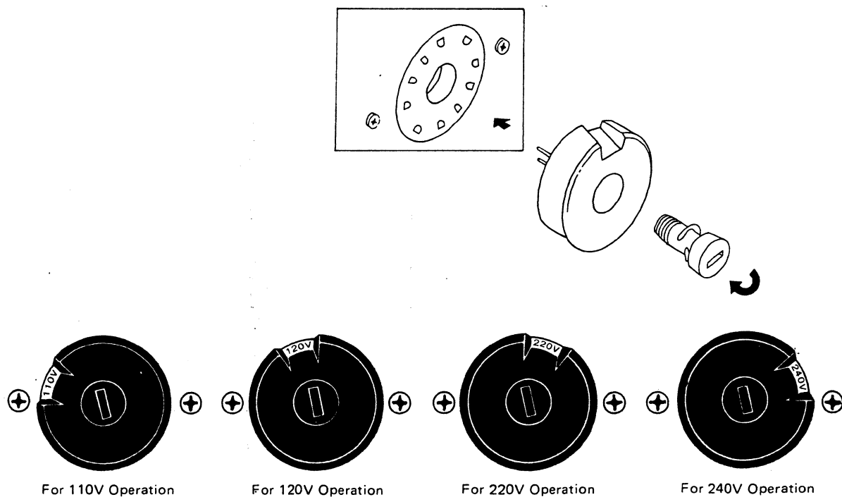
Figure 2. Voltage Conversion Chart
