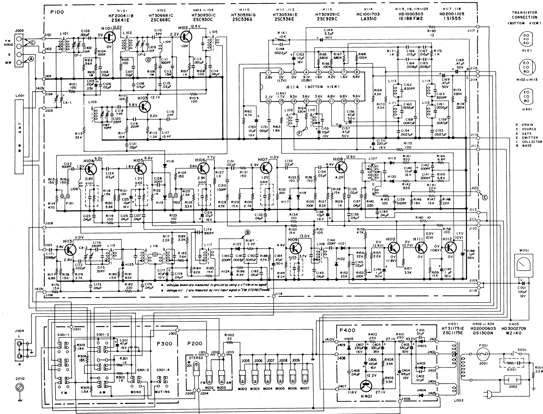
Figure 9. Schematic Diagram
