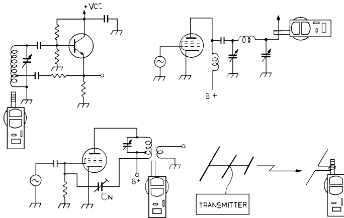
Fig. 2 Absorption wavemeter applications.
