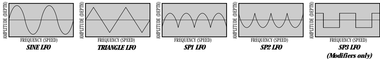
Figure 4-2 LFO Types
