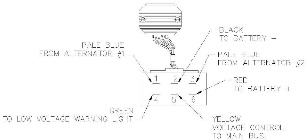
REGULATOR PLUG WIRING
