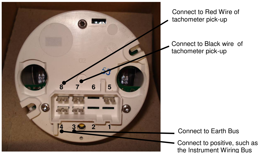
Figure 16. Tachometer Connections
