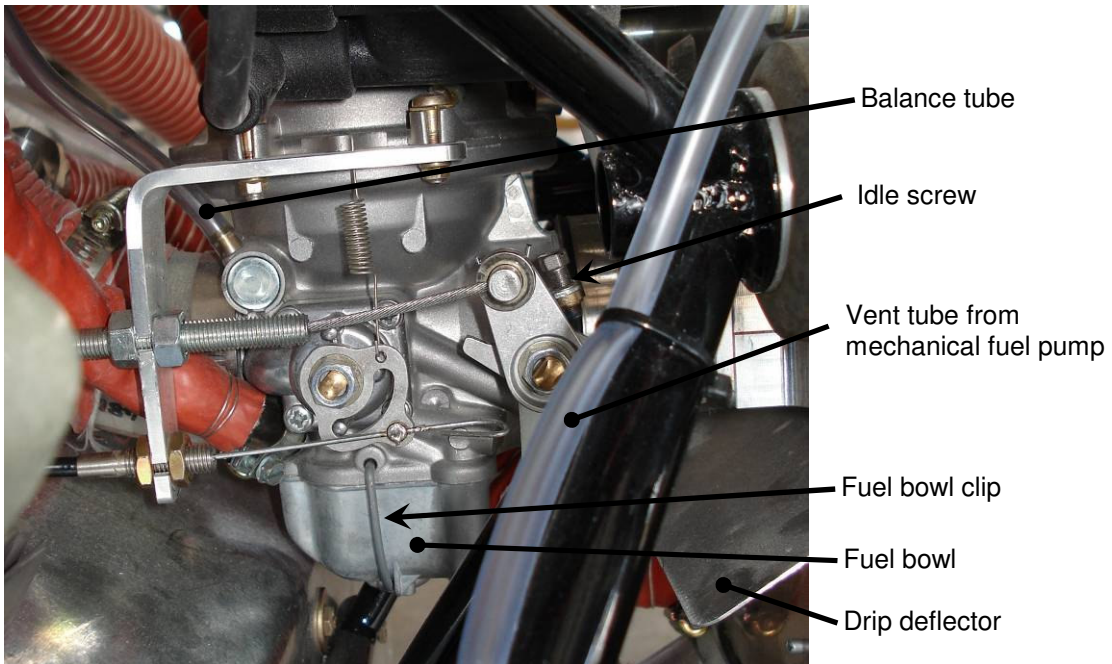
Figure 29. Carburettor Installation
