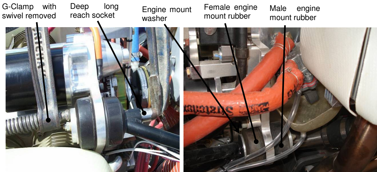
Figure 41 Upper & Lower Engine Mount Detail
