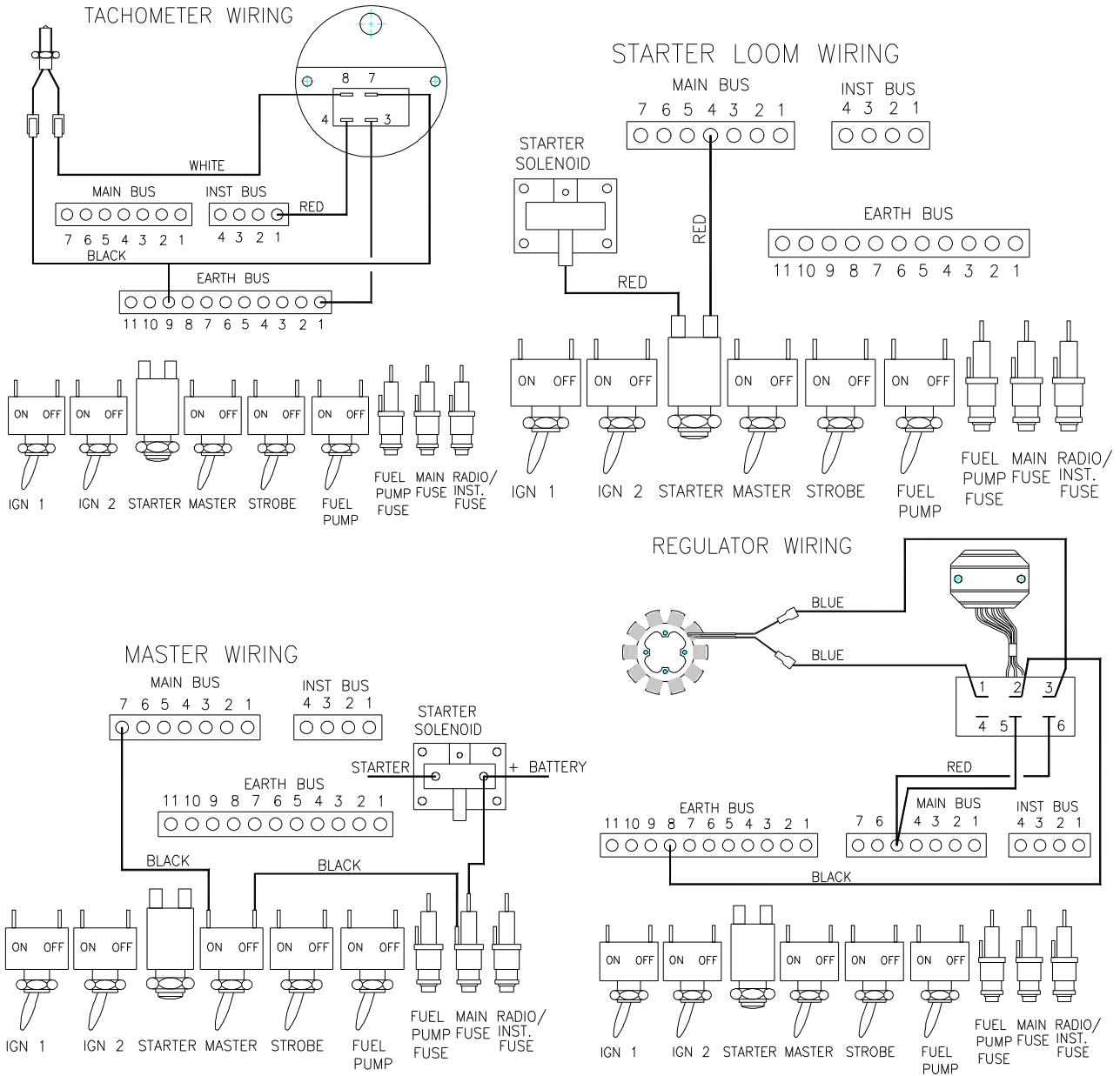
Figure 63. Wiring Details
