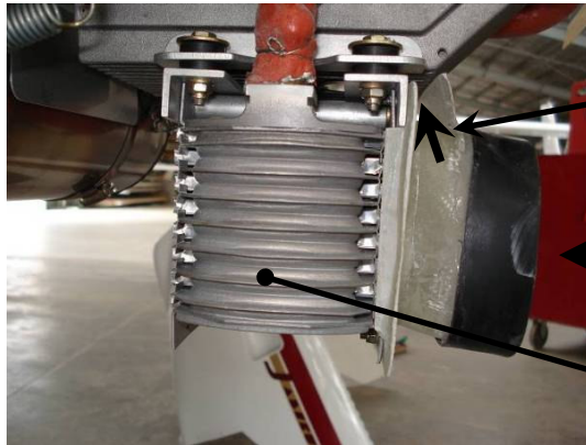
Figure 54. Oil Cooler Duct Design
