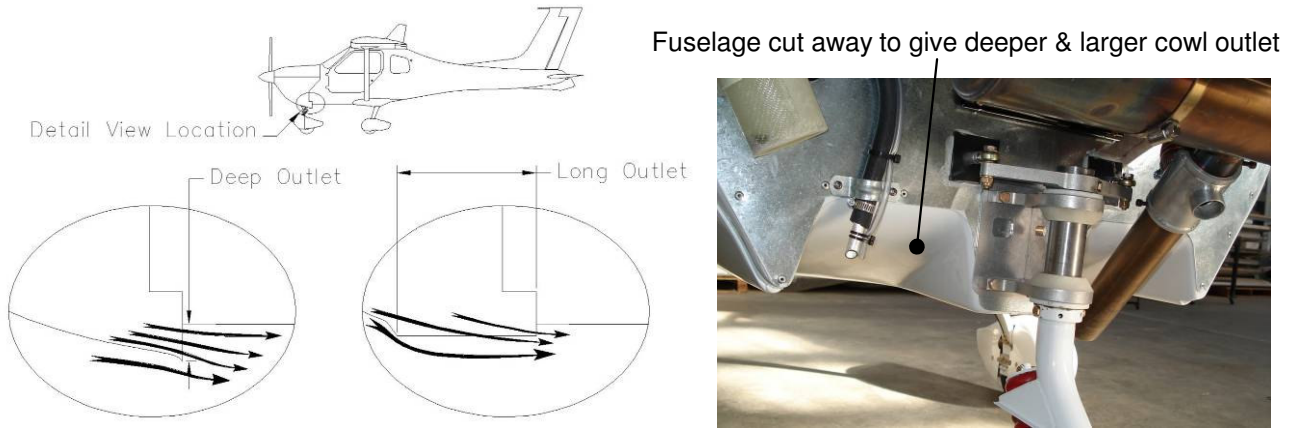
Figure 58. Cowl Outlet Geometry
