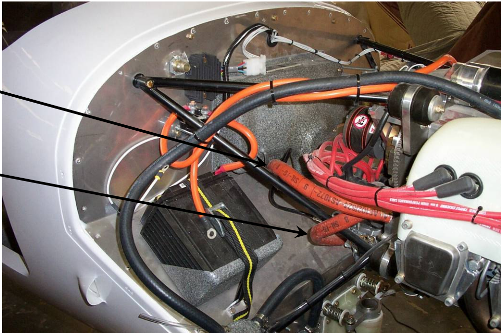
Figure 43. Fuel Connections General
