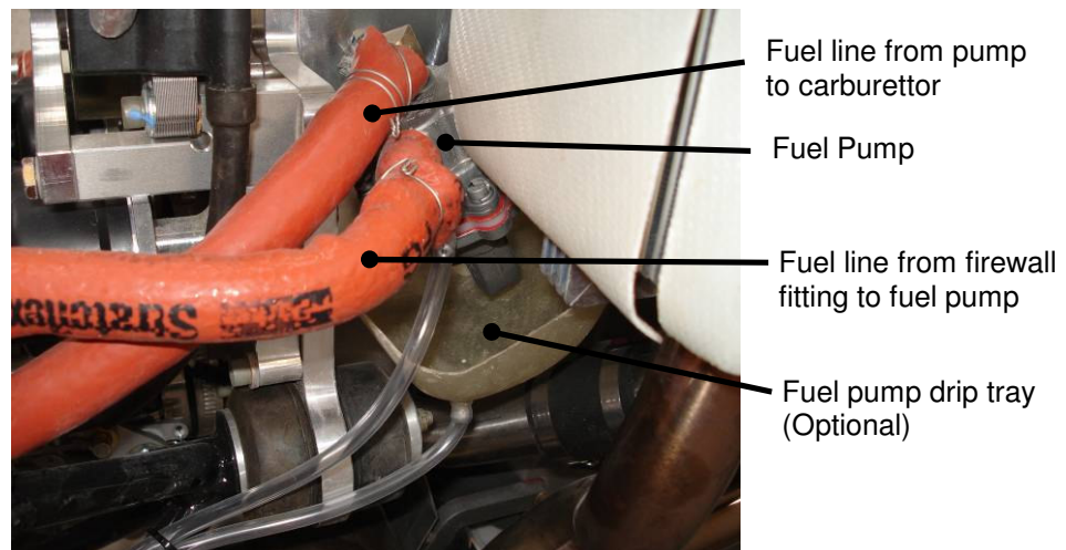
Figure 28. Mechanical Fuel Pump
