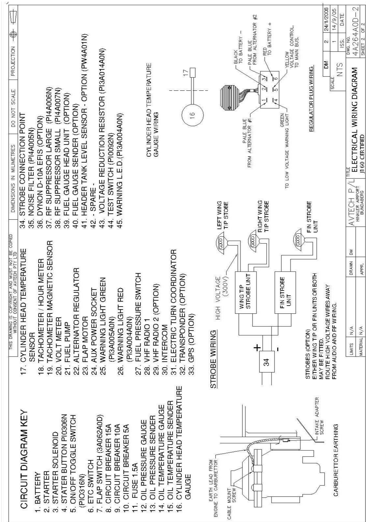
Figure 27. Wiring Diagram Key
