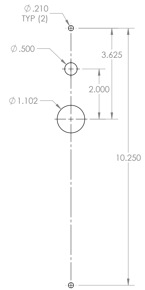
PANEL CUTOUT SCALE: 1:2
