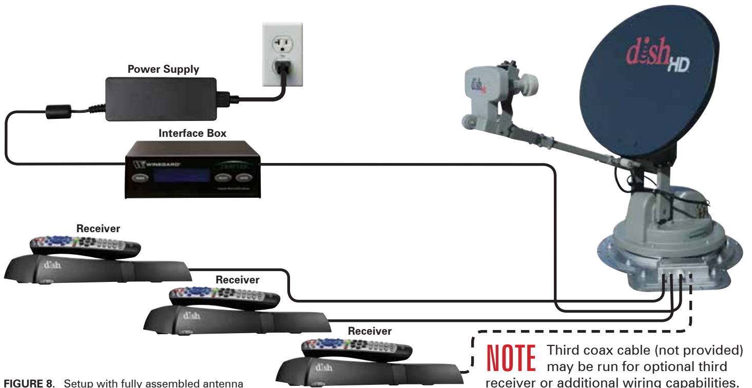
FIGURE 8. Setup with fully assembled antenna
