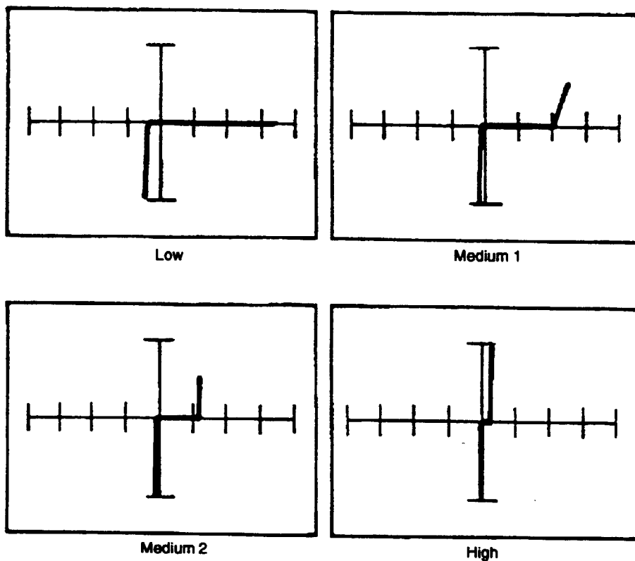
Figure 12-68. Signatures Between the E2 Pin and the Ground Pin of a 6301-1J at 60 Hz.
