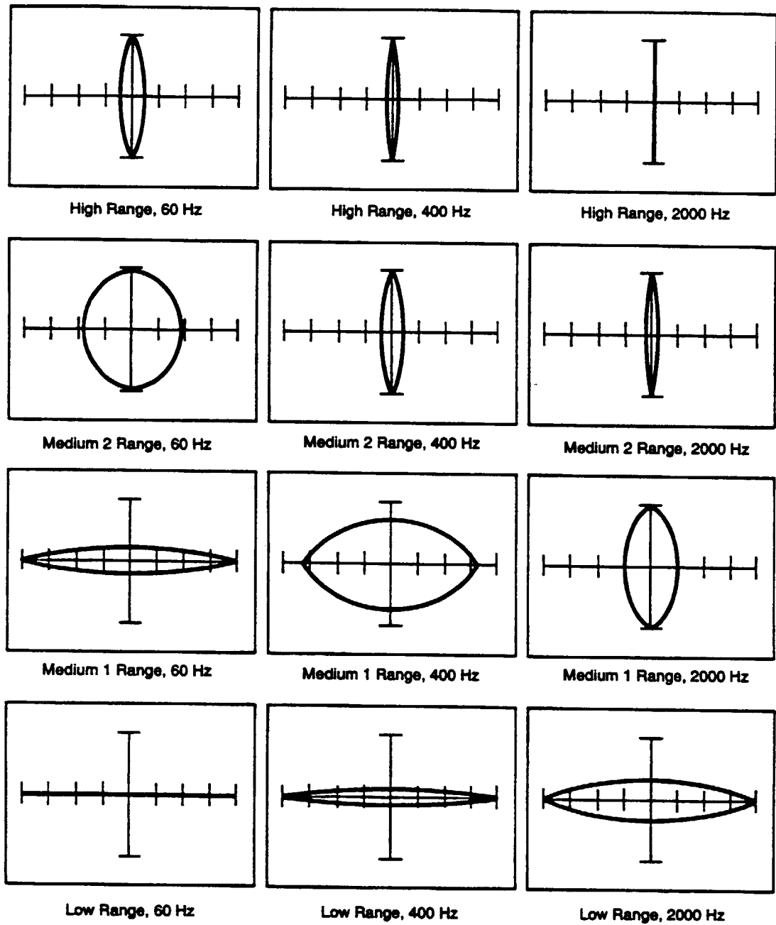
Figure 7-5. Signatures of a 0.22μF Capacitor.
