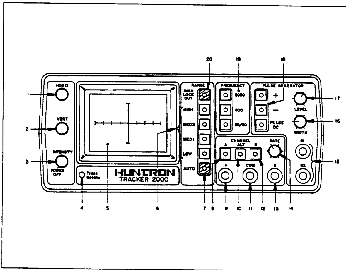
Figure 2-1. Front Panel.
