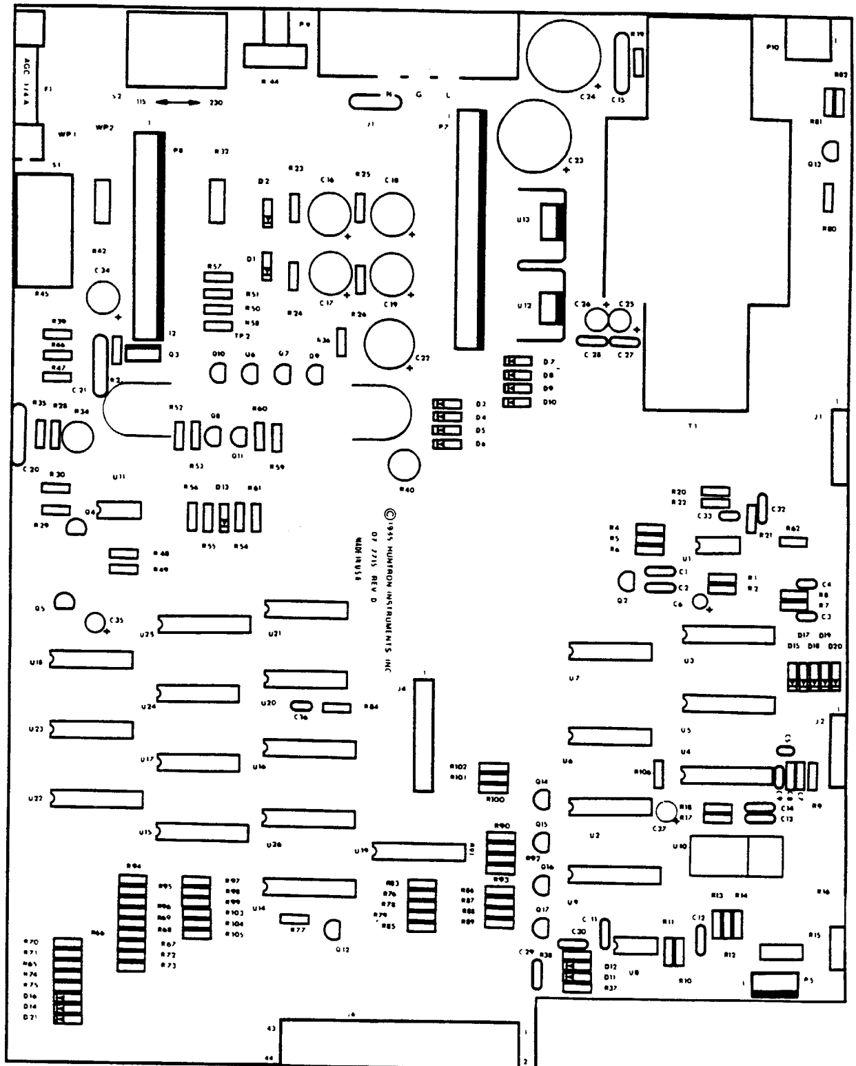
Figure 6-1. Main PCB Component Locations
