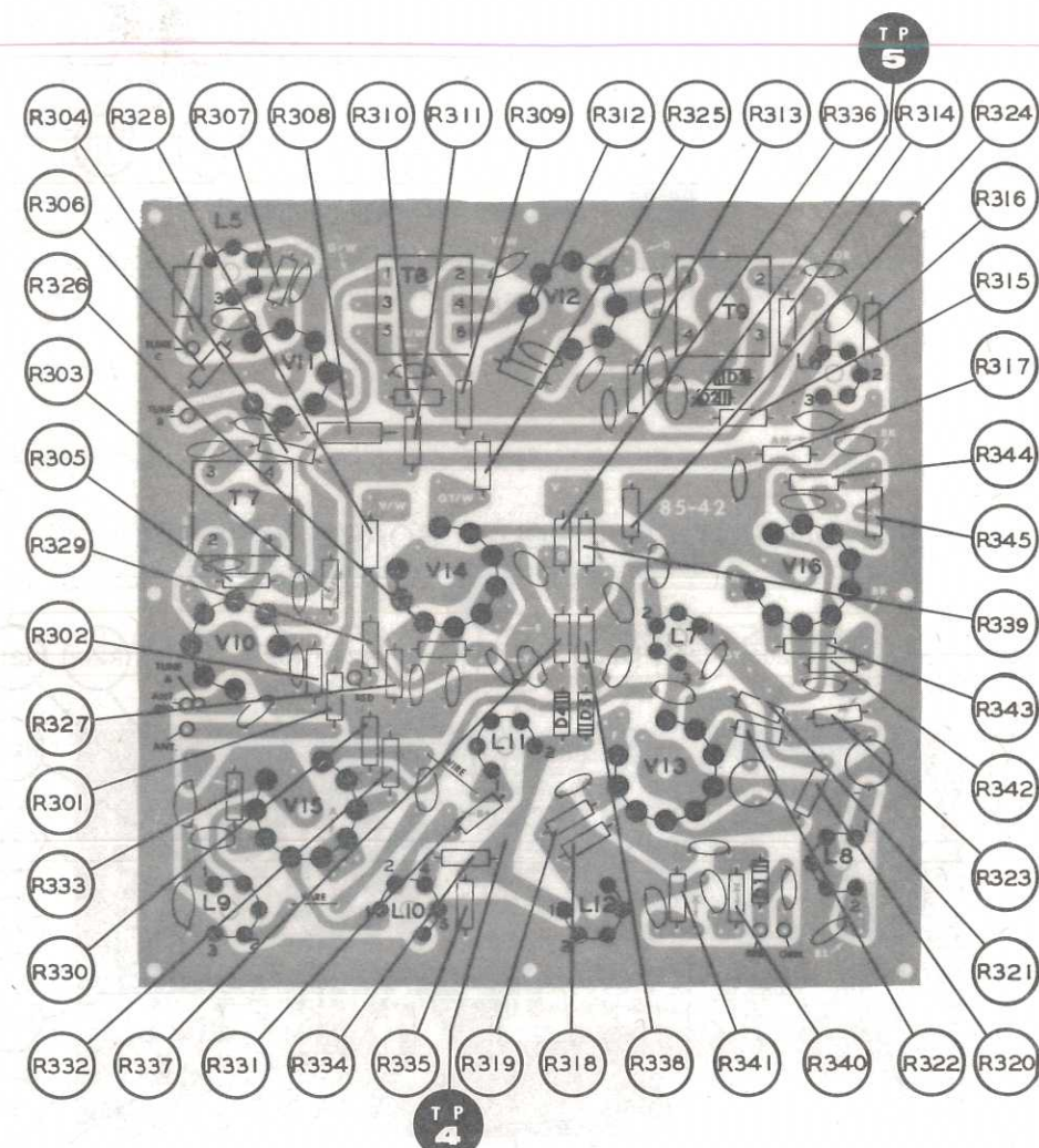
RESISTORS FOIL SIDE OF BOARD
