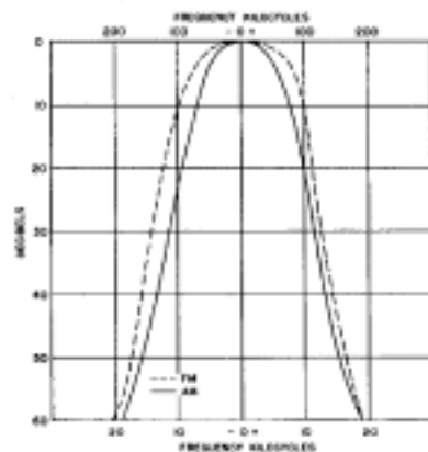
FM & AM selectivity characteristics
