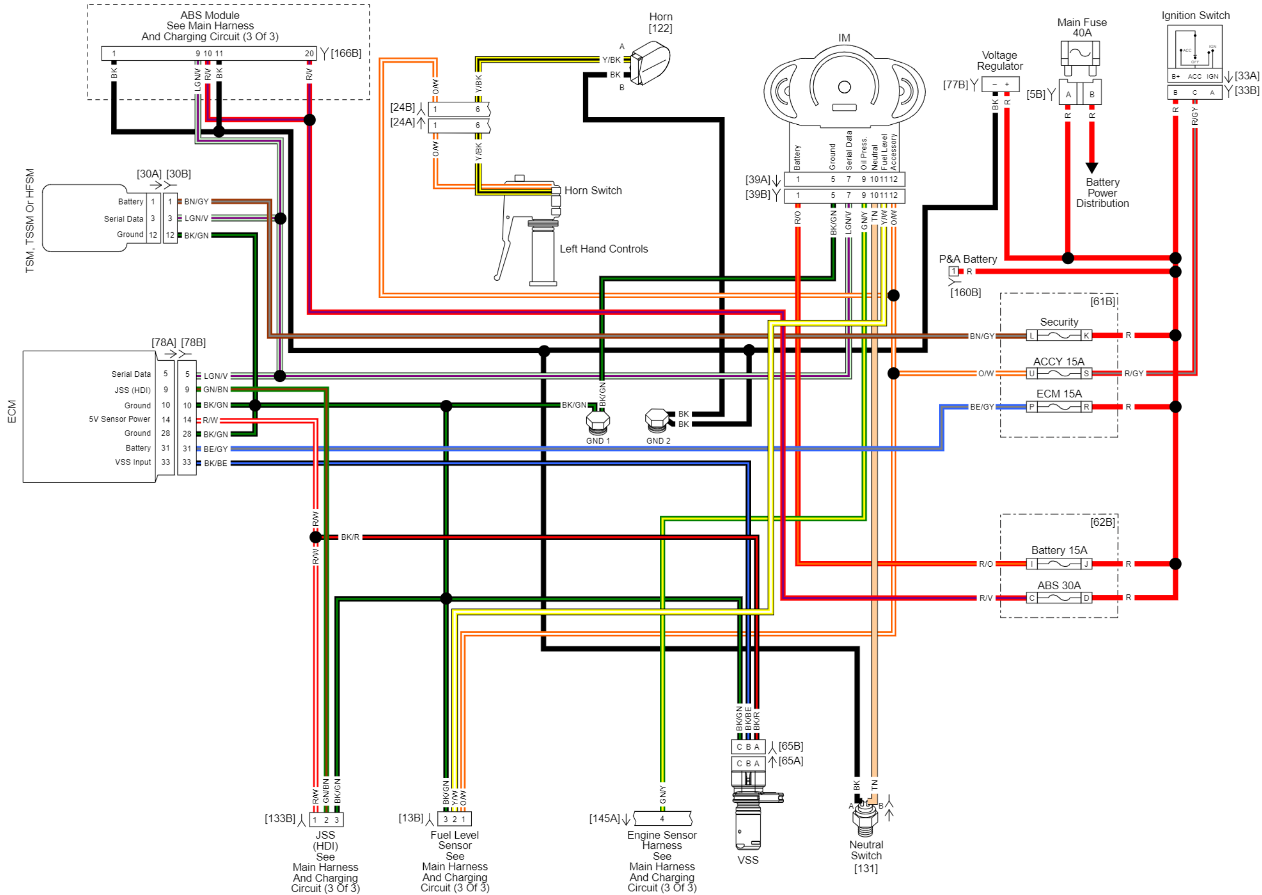
Horn and Instrument Circuit: 2012 VRSC
