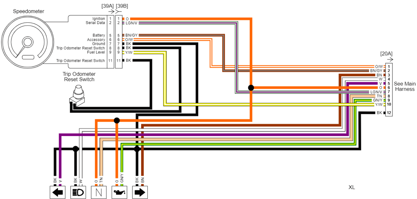
Instrument, Indicators, and Hand Controls: 2012 Sportster
