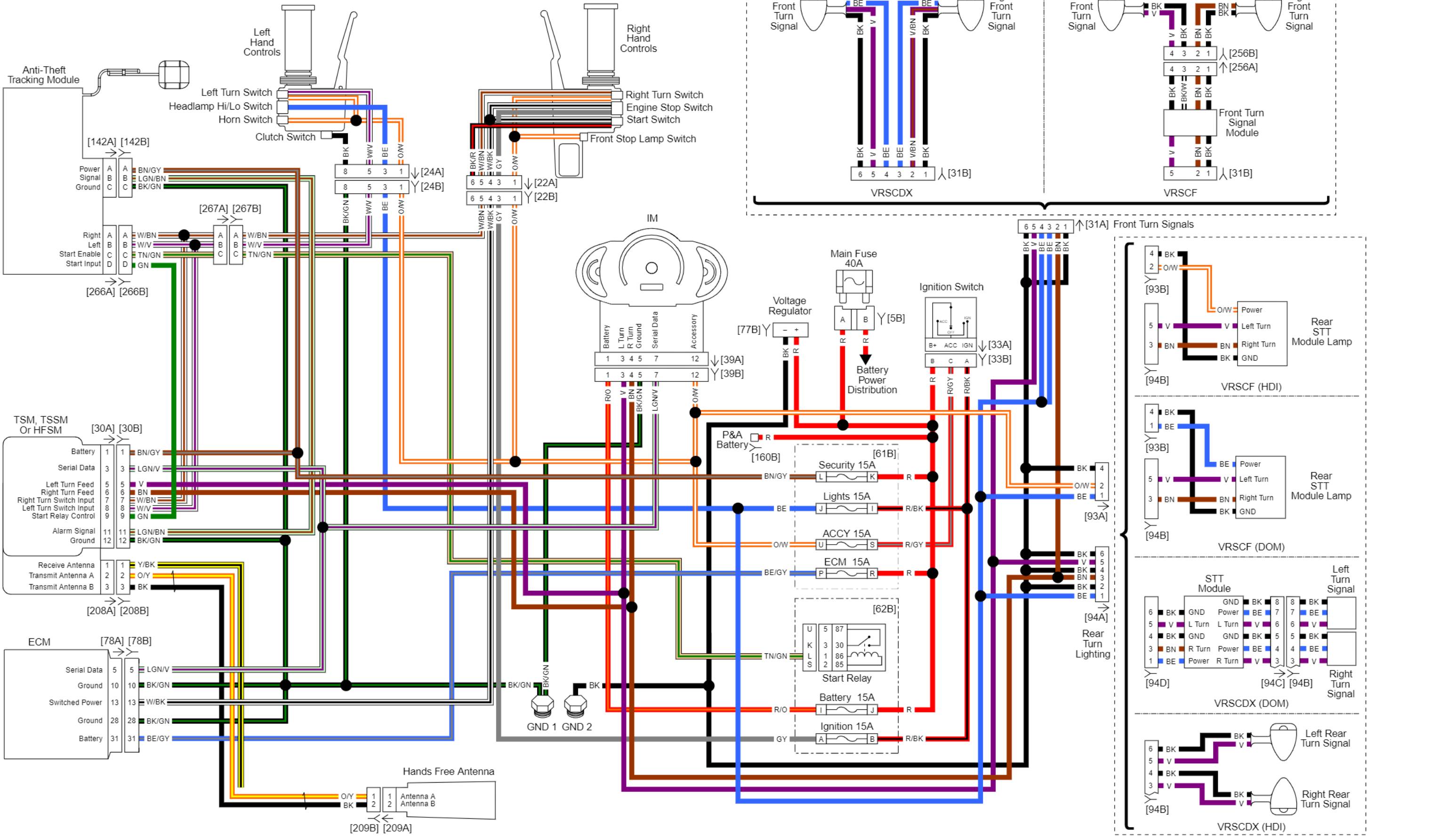
Security Circuit With Anti-Theft Tracking Module: 2012 VRSC
