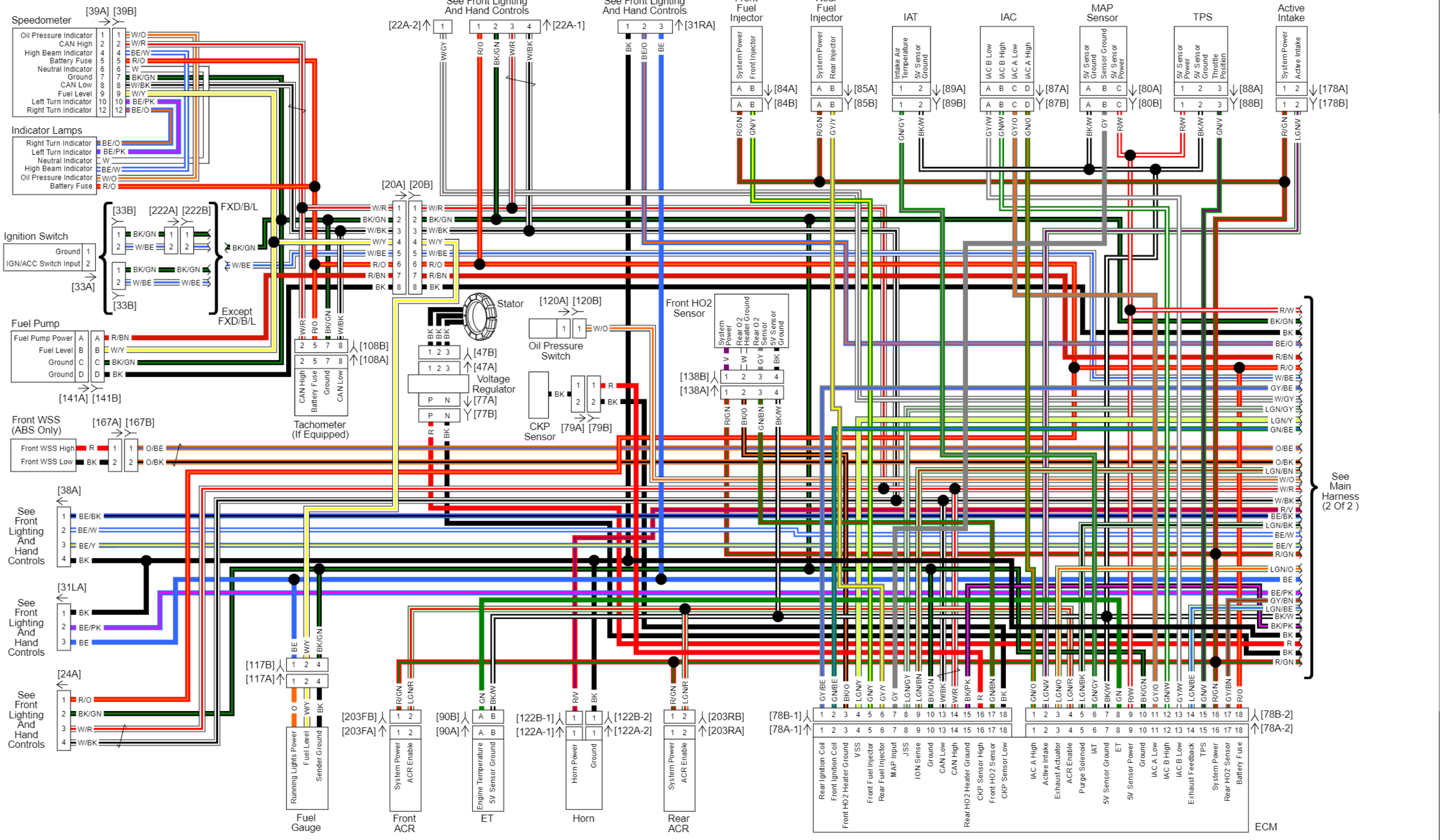
Main Harness 1 of 2: 2012 Dyna
