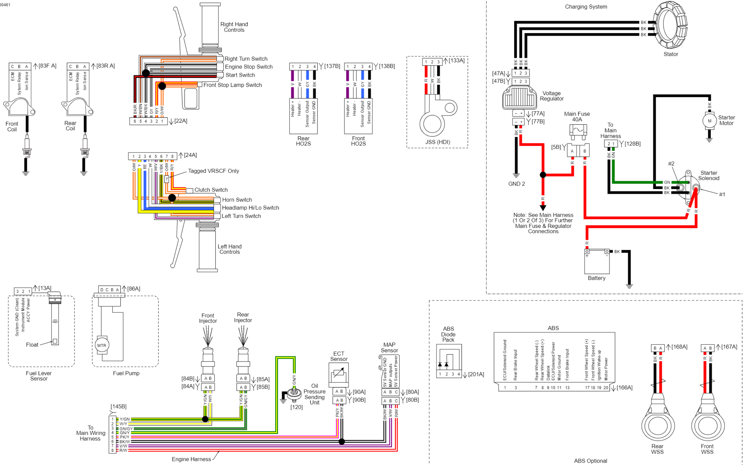
Main Harness and Charging Circuit (3 of 3): 2012 VRSC
