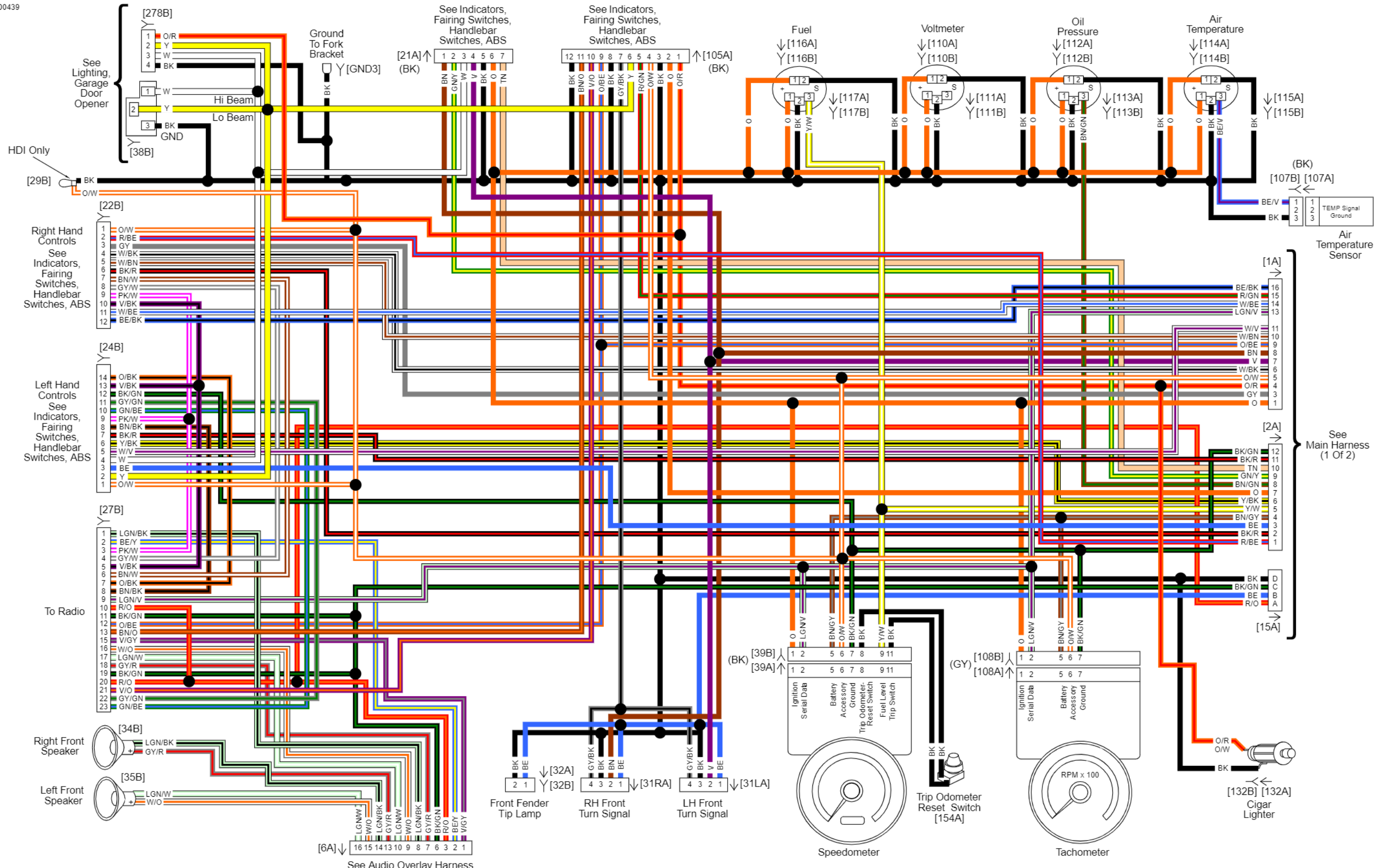
Fairing Harness: 2012 FLHTCUSE7
