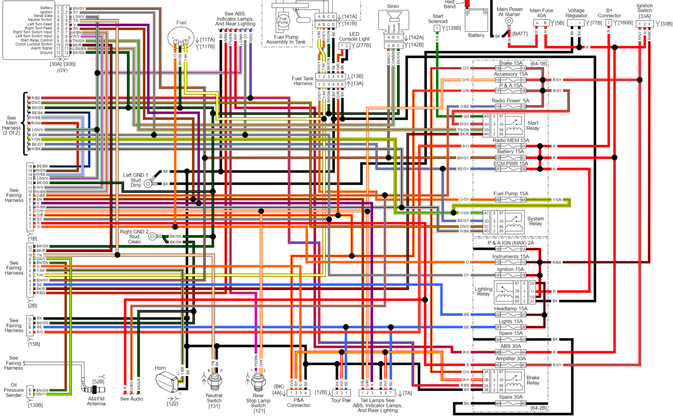
Main Wiring Harness (1 of 2): 2012 FLHXSE3
