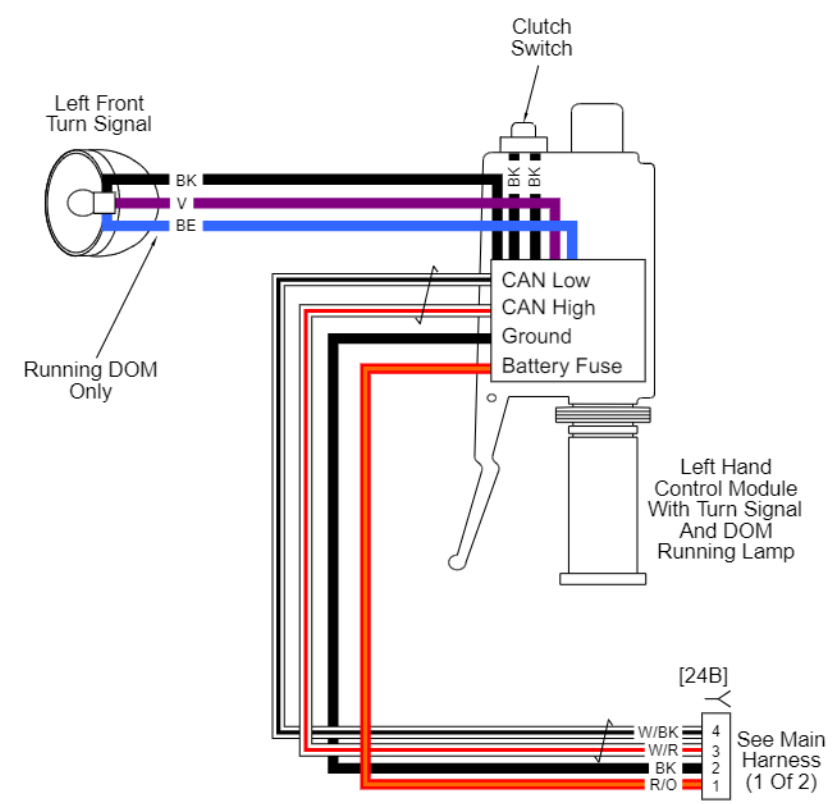
Front Lighting and Hand Controls: 2012 Softail
