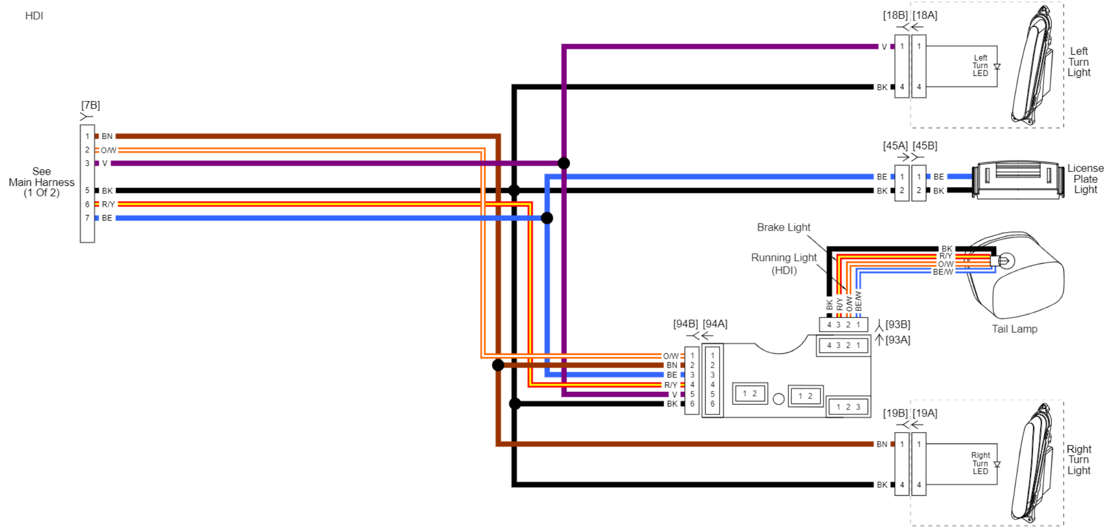
Rear Lighting: 2012 FLTRXSE
