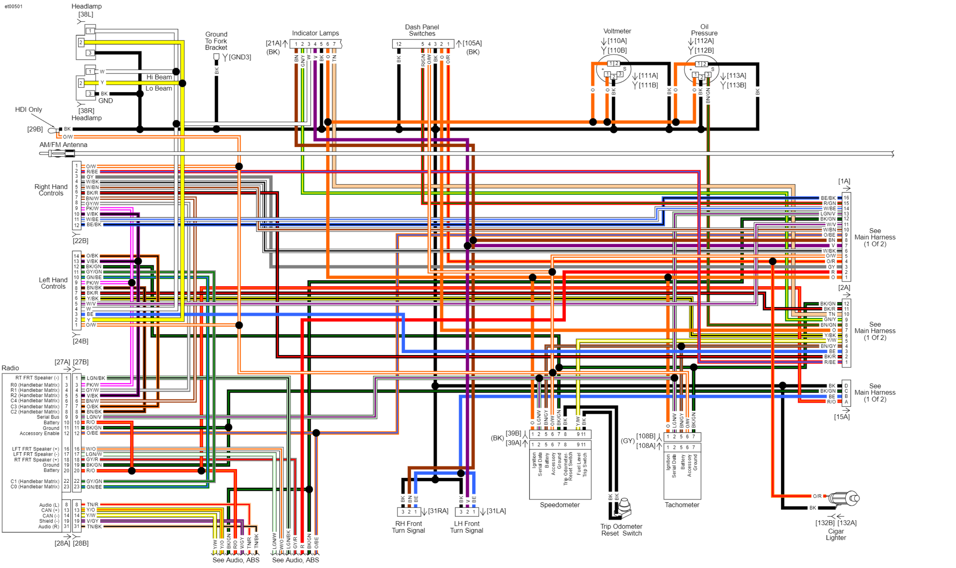
Fairing Harness: 2012 FLTRXSE
