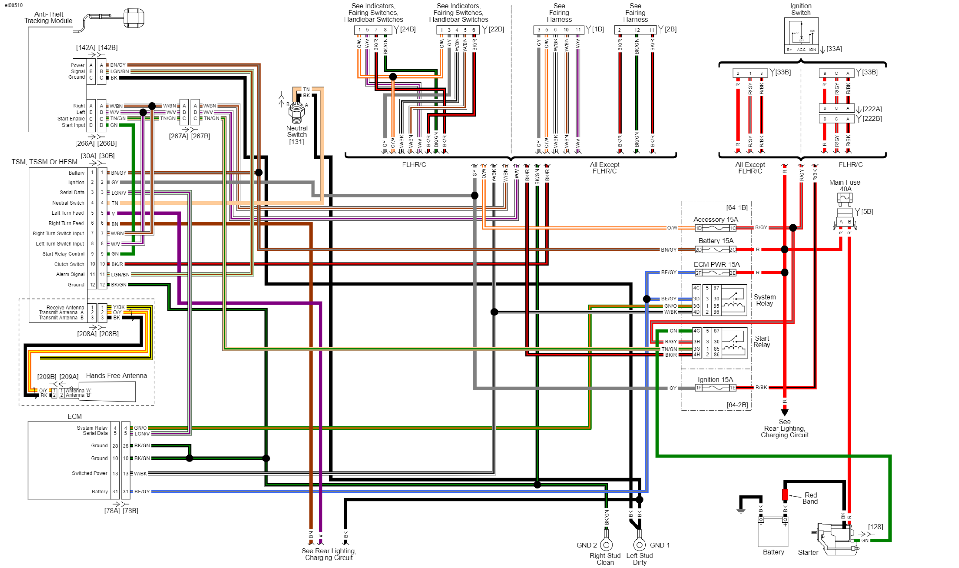
Security Circuit: 2012 Touring With Anti-Theft Tracking Module
