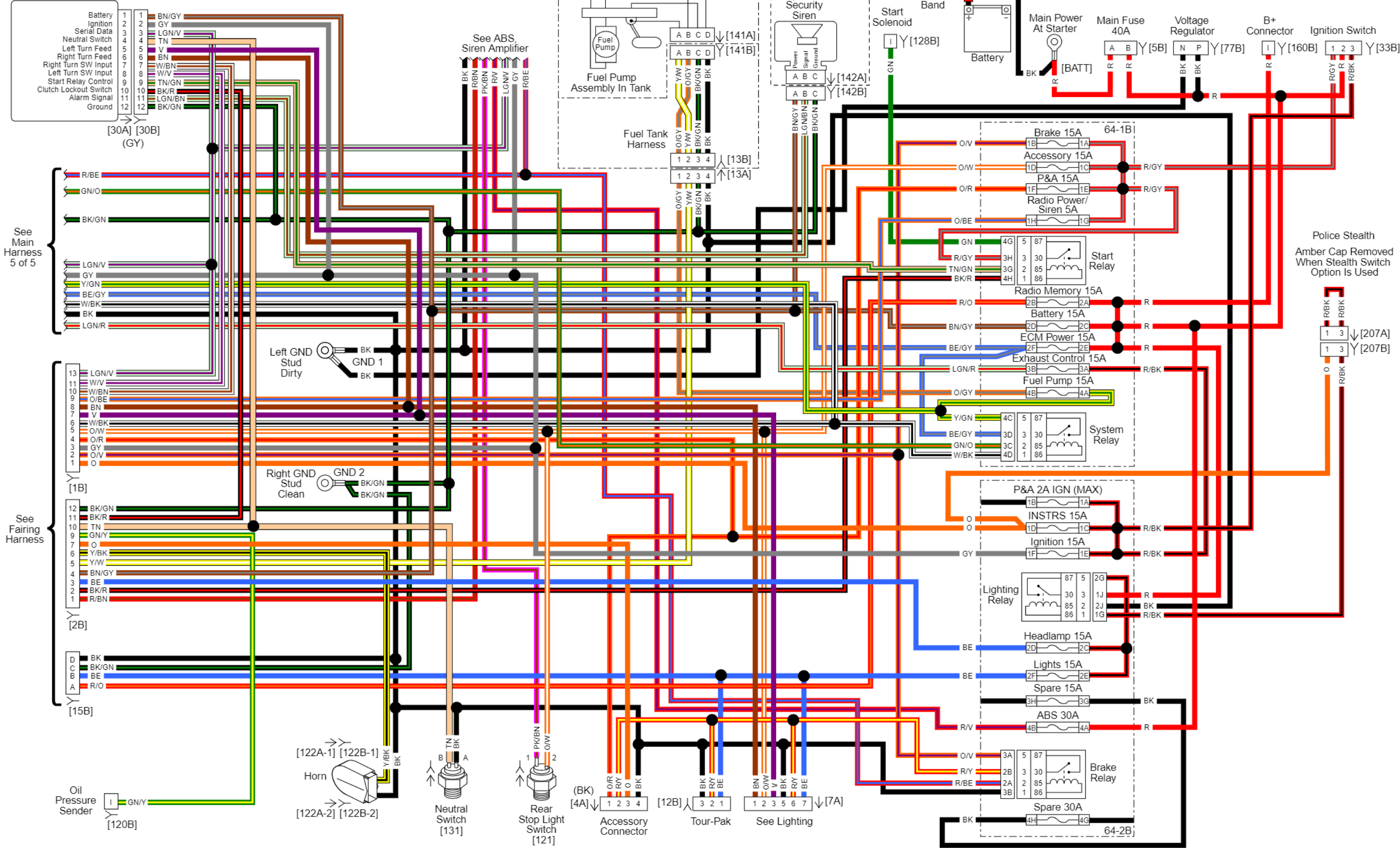
Main Harness (1 of 3): 2012 FLHTP
