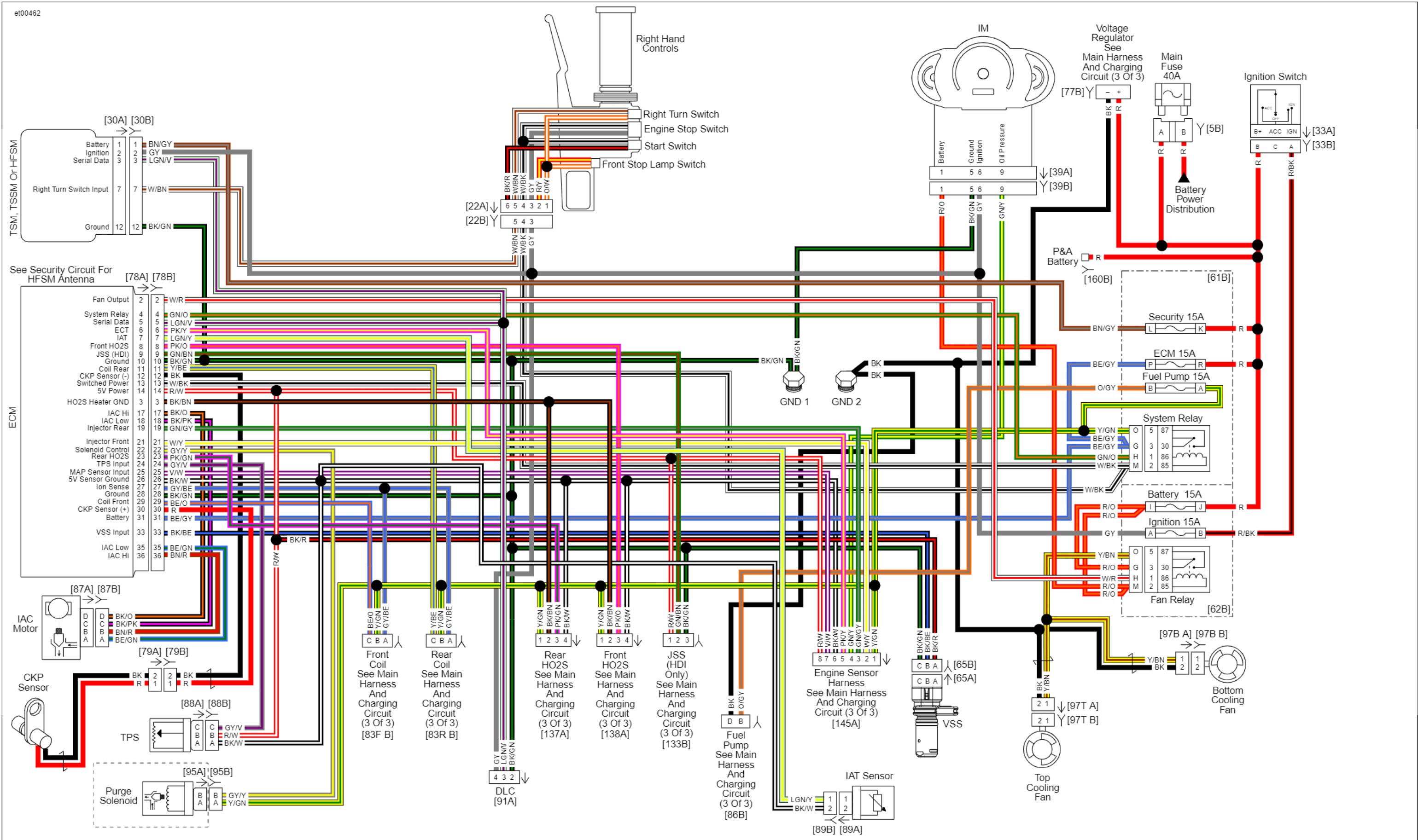
Ignition Circuit: 2012 VRSC
