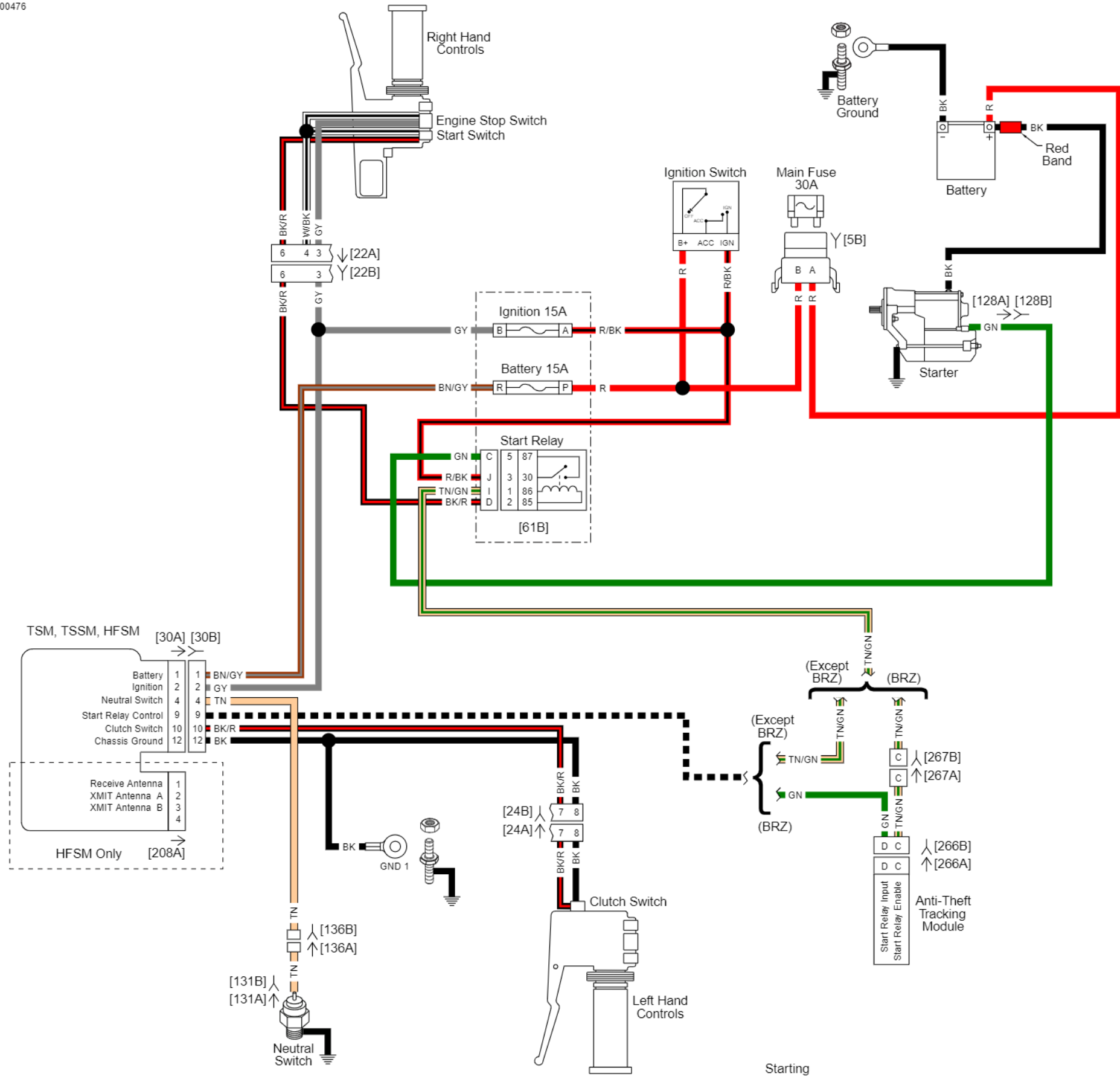
Starting and Charging Circuit: 2012 Sportster
