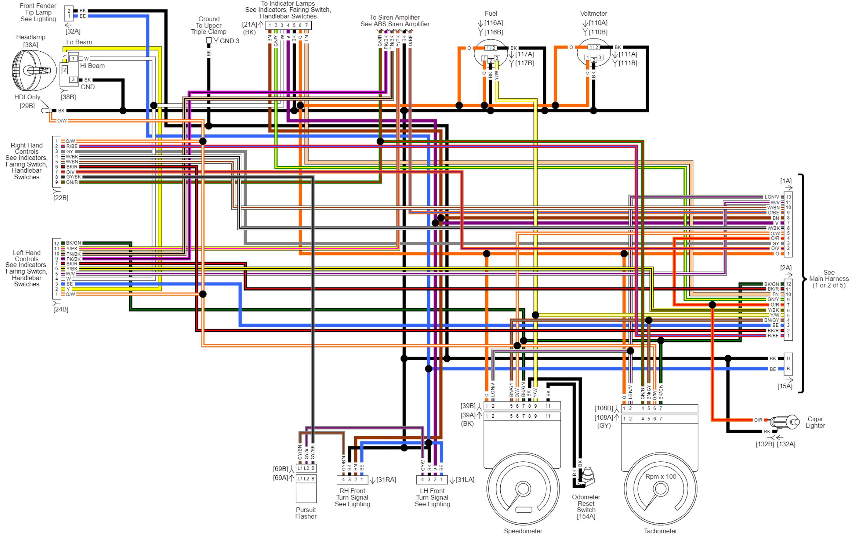
Fairing Harness: 2012 FLHTP
