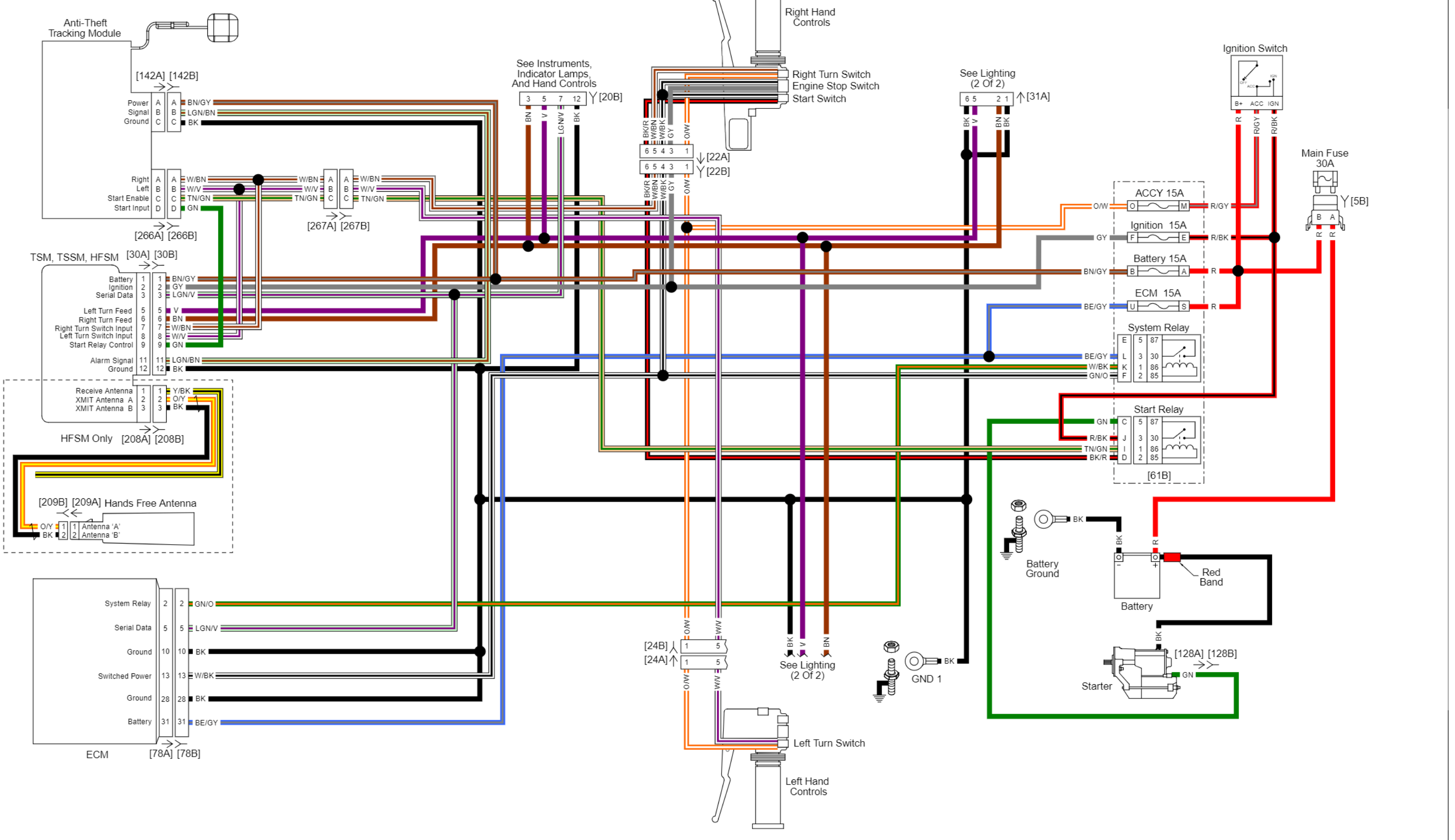
Security Circuit with Anti-Theft Tracking Module: 2012 Sportster
