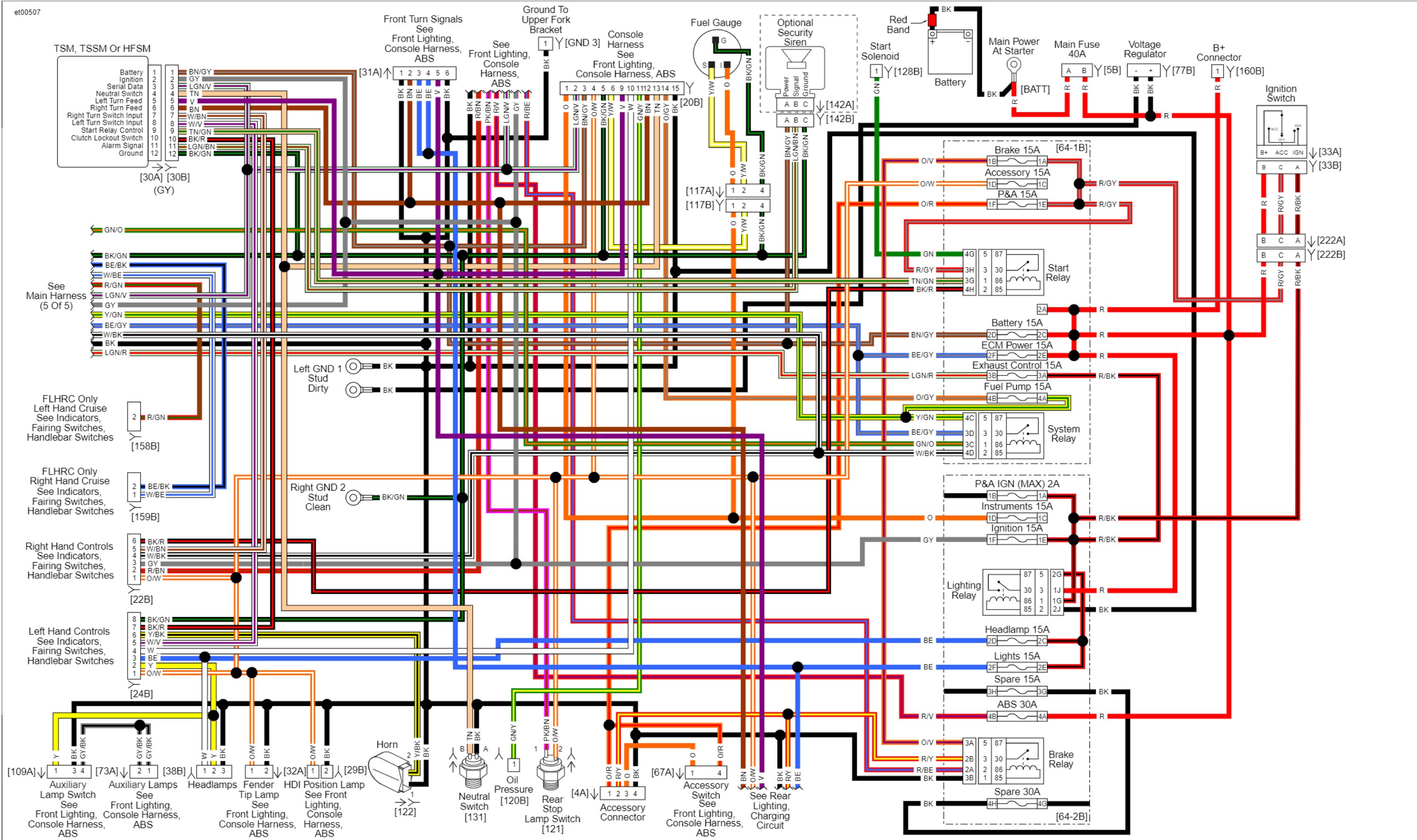
Main Harness (4 OF 5): 2012 Touring (FLHR/C) with ABS
