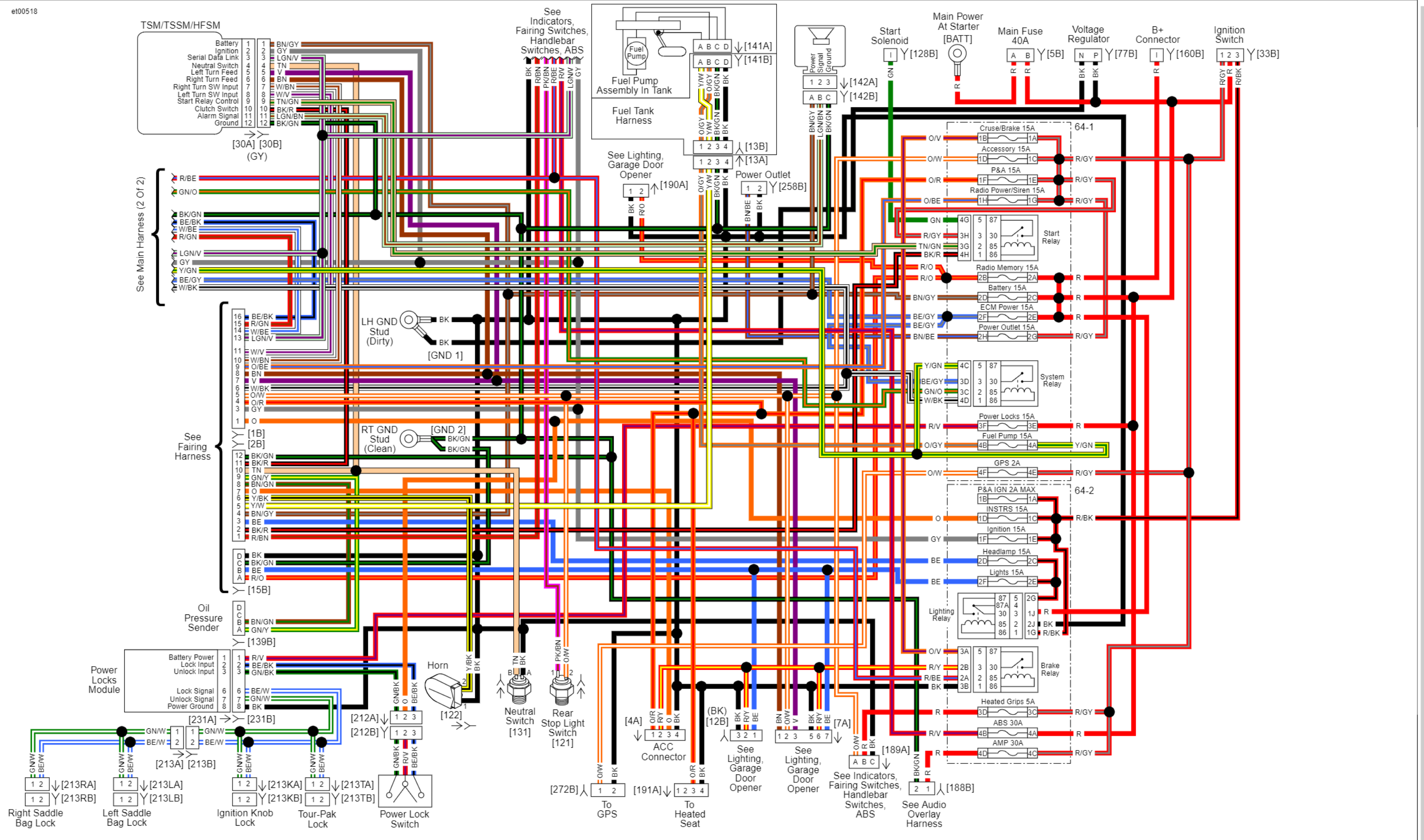
Main Harness (1 of 2): 2012 FLHTCUSE7
