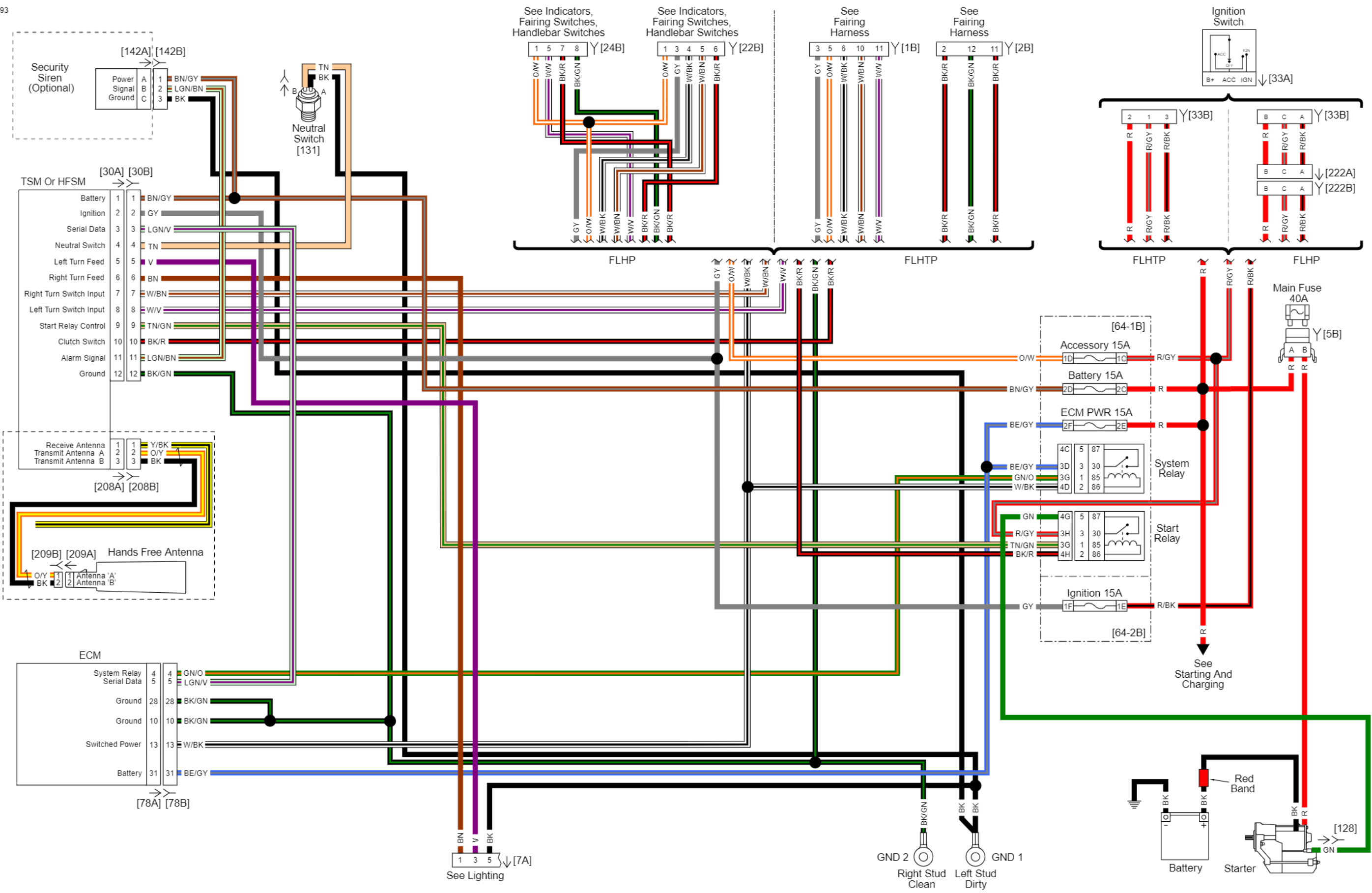
Security Circuit: 2012 FLHTP, FLHP
