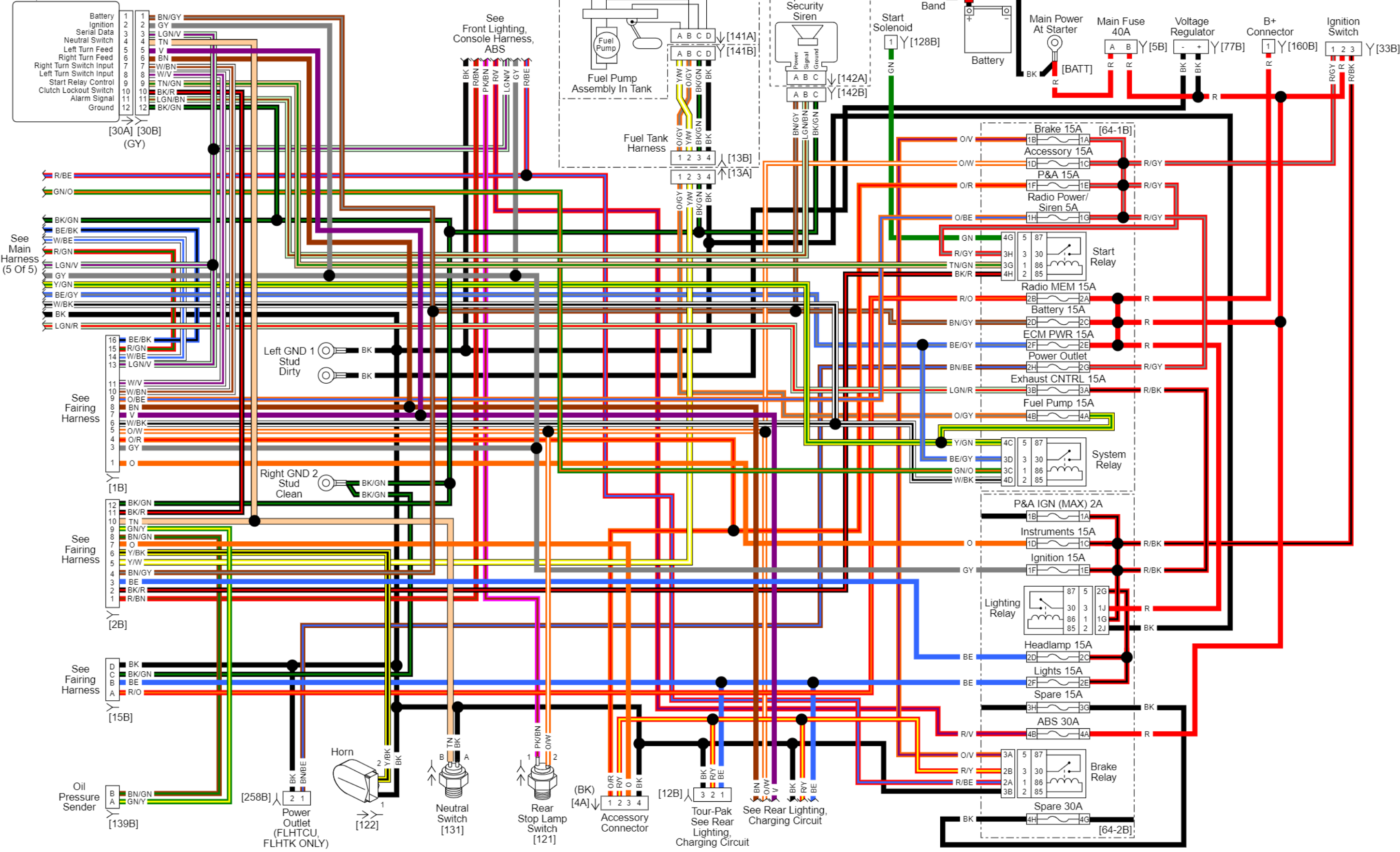
Main Harness (2 OF 5): 2012 Touring (Except FLHR/C) with ABS
