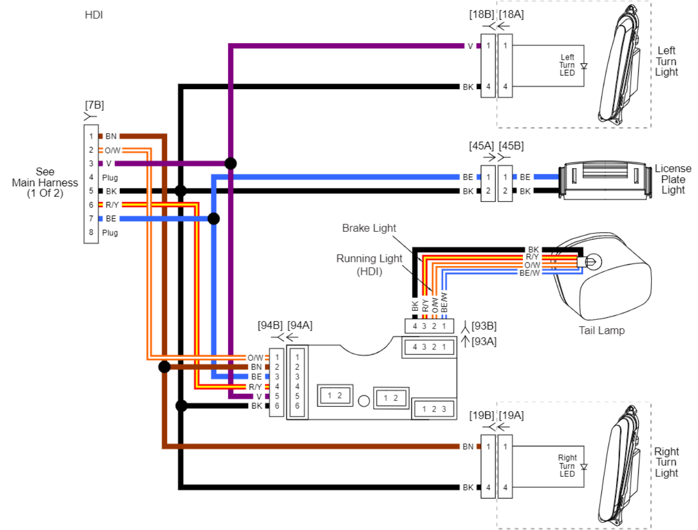
ABS, Indicator Lamps and Rear Lighting: 2012 FLHXSE3
