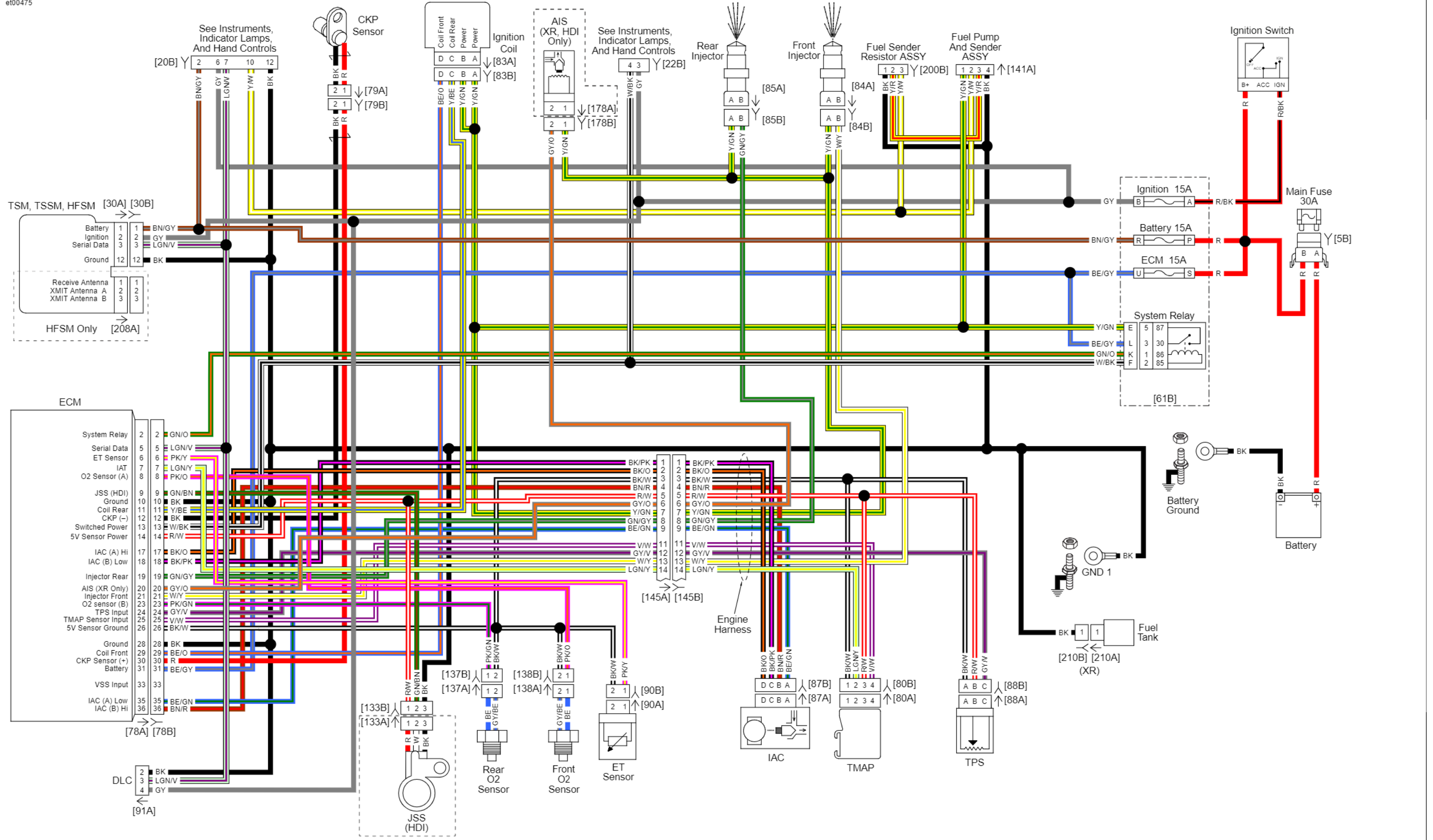
Engine Management: 2012 Sportster
