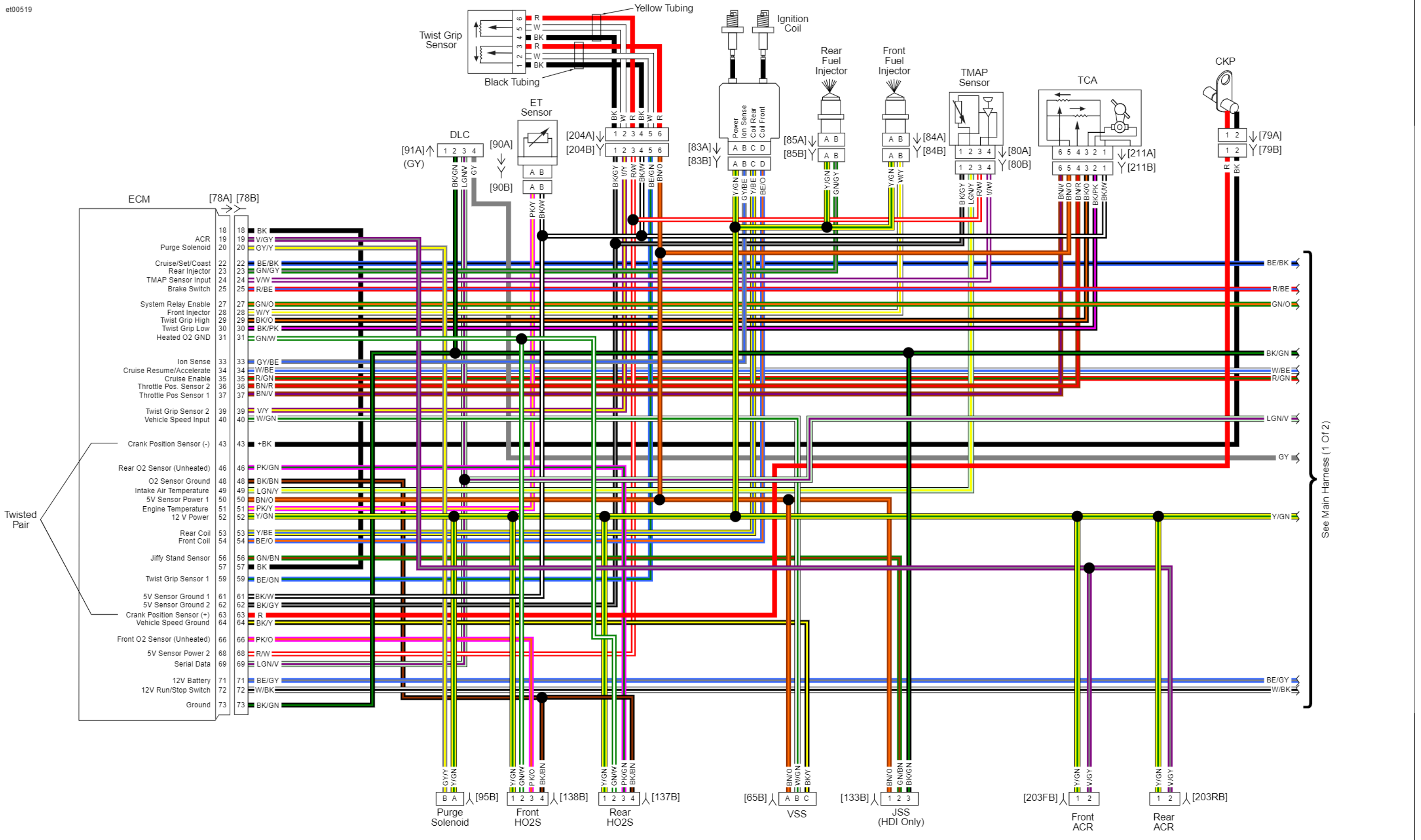
Main Harness (2 of 2): 2012 FLHTCUSE7
