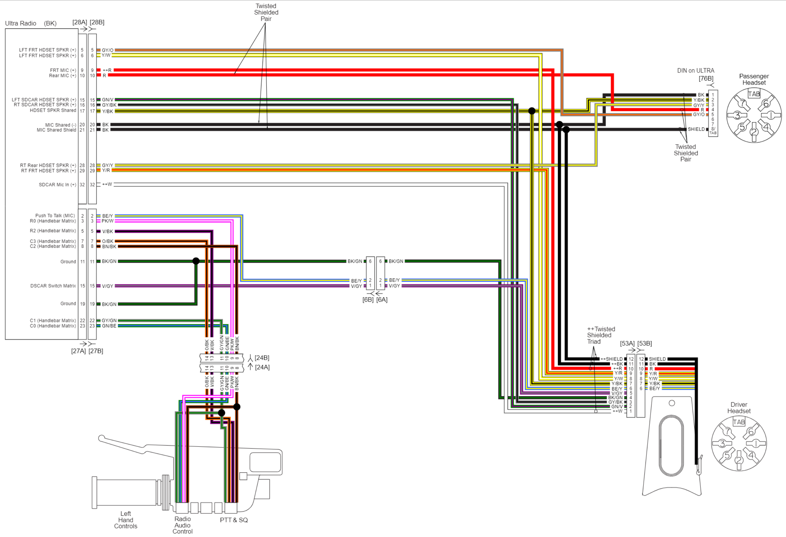
2-Place Intercom and Headset Audio: 2012 Touring
