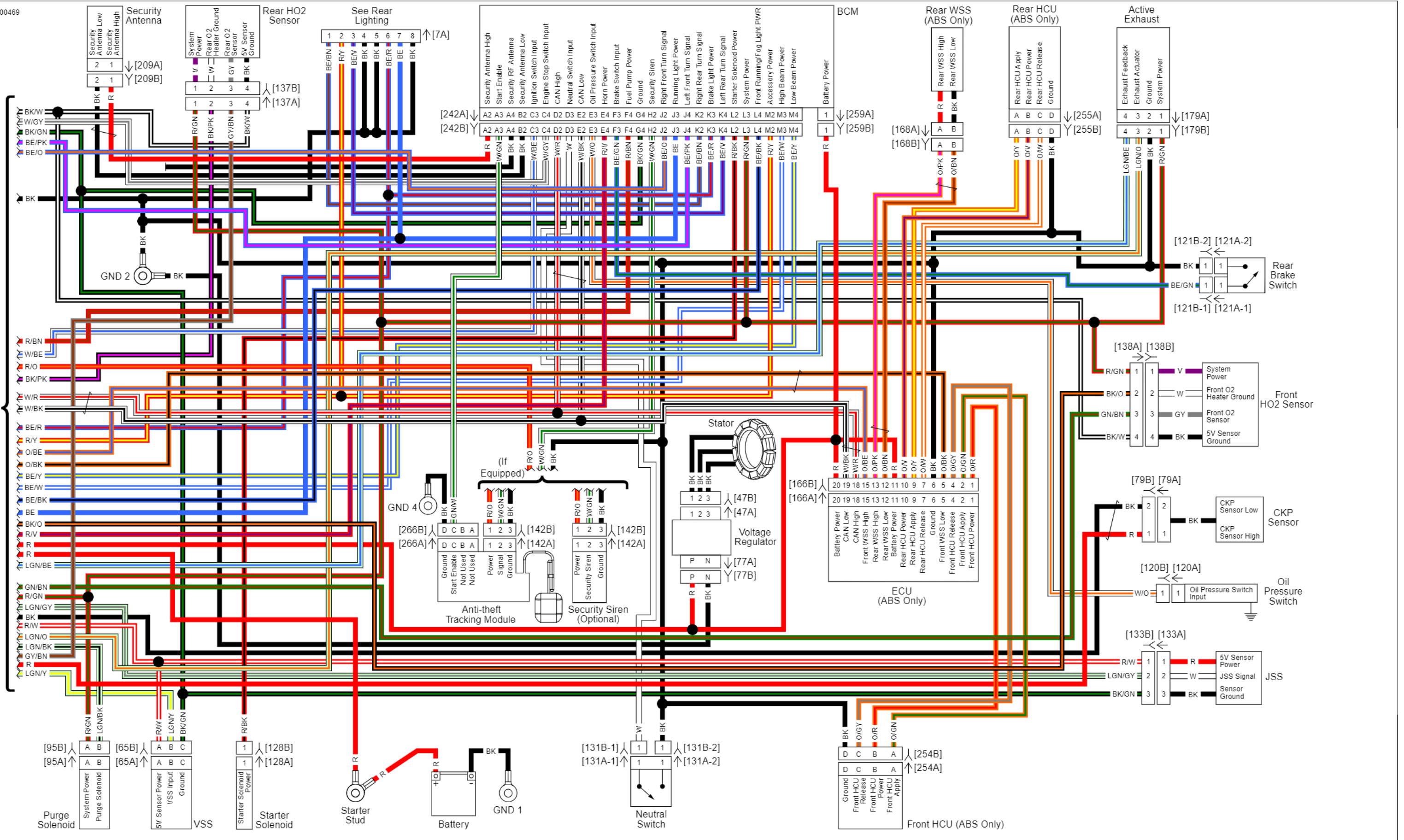
Main Harness 2 of 2: 2012 Softail (Except FXS)
