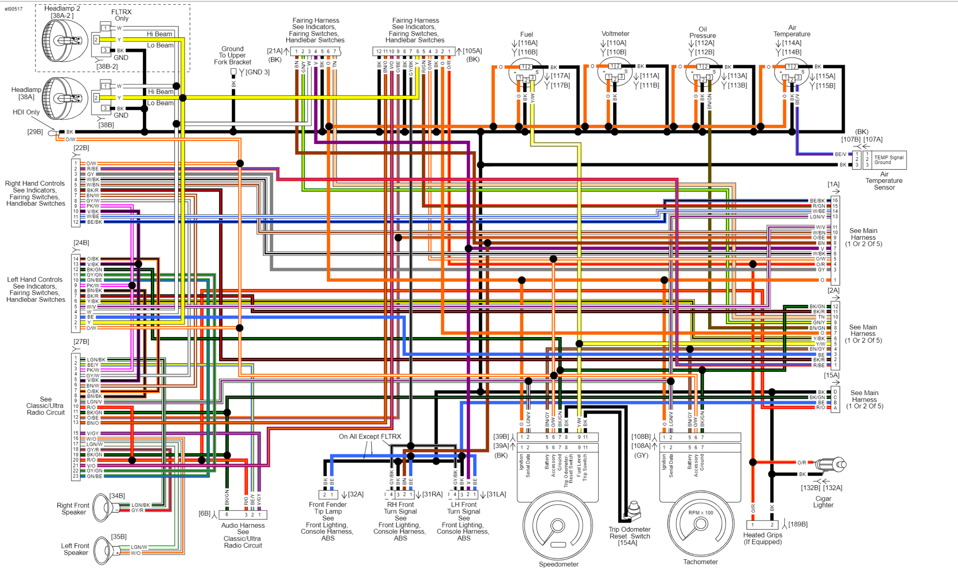
Fairing Harness: 2012 Touring
