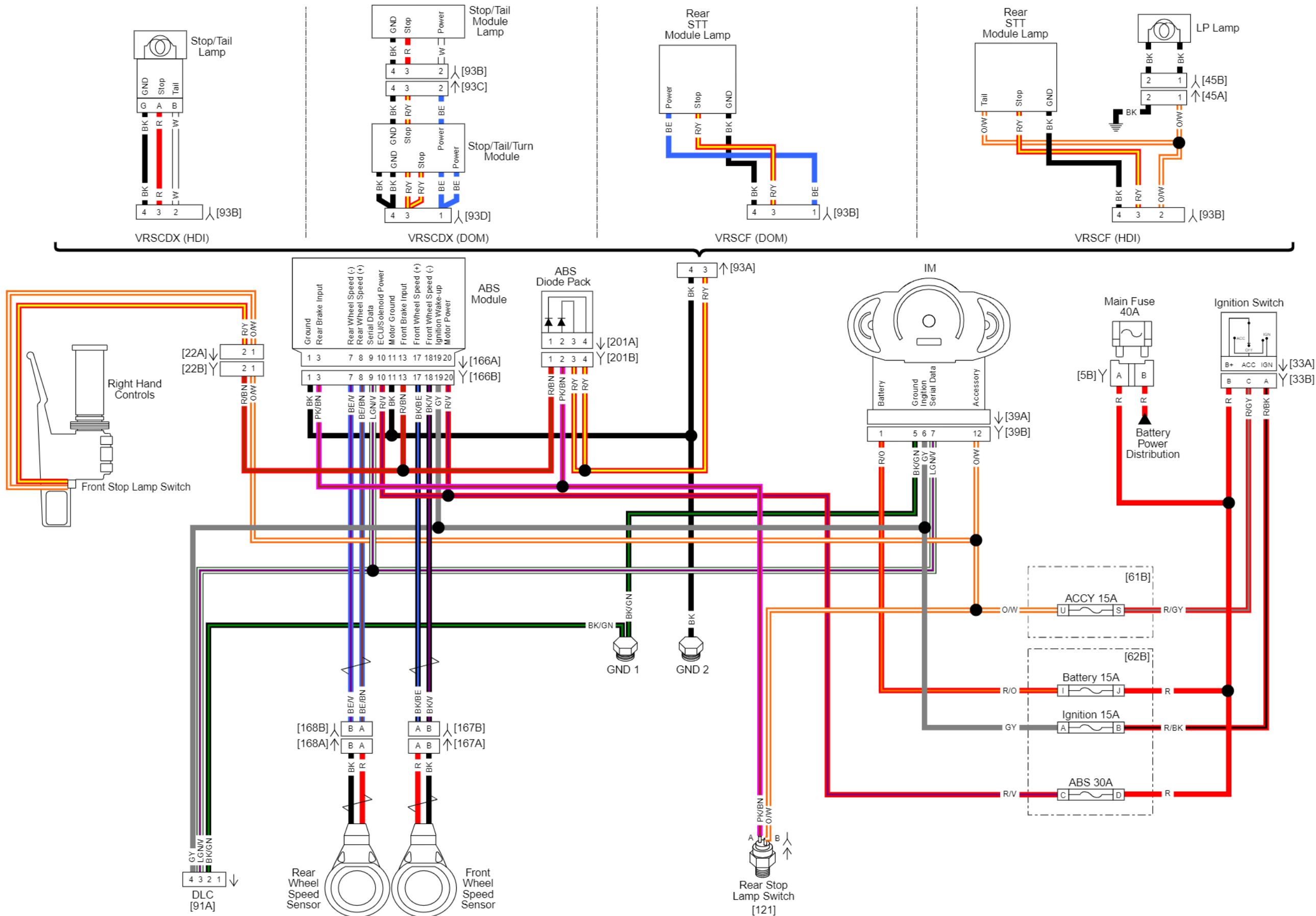
ABS Circuit: 2012 VRSC
