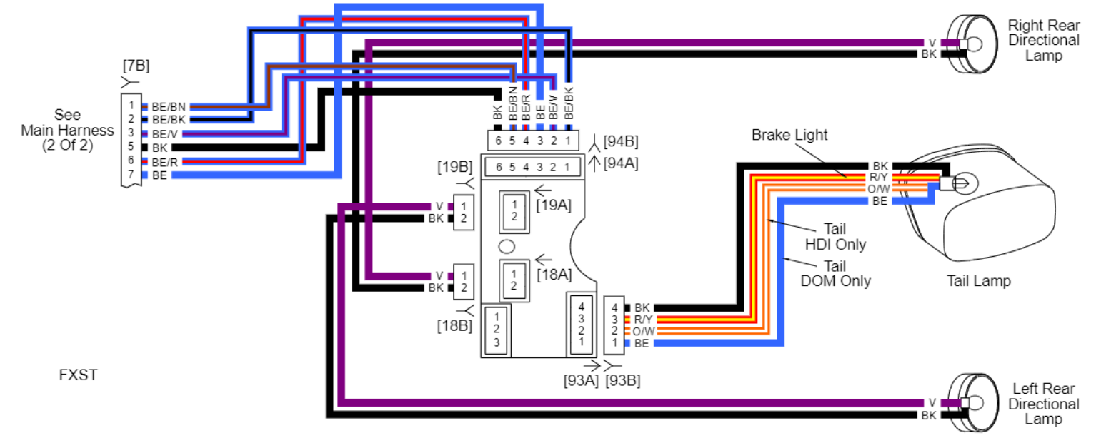
Rear Lighting: 2012 Softail
