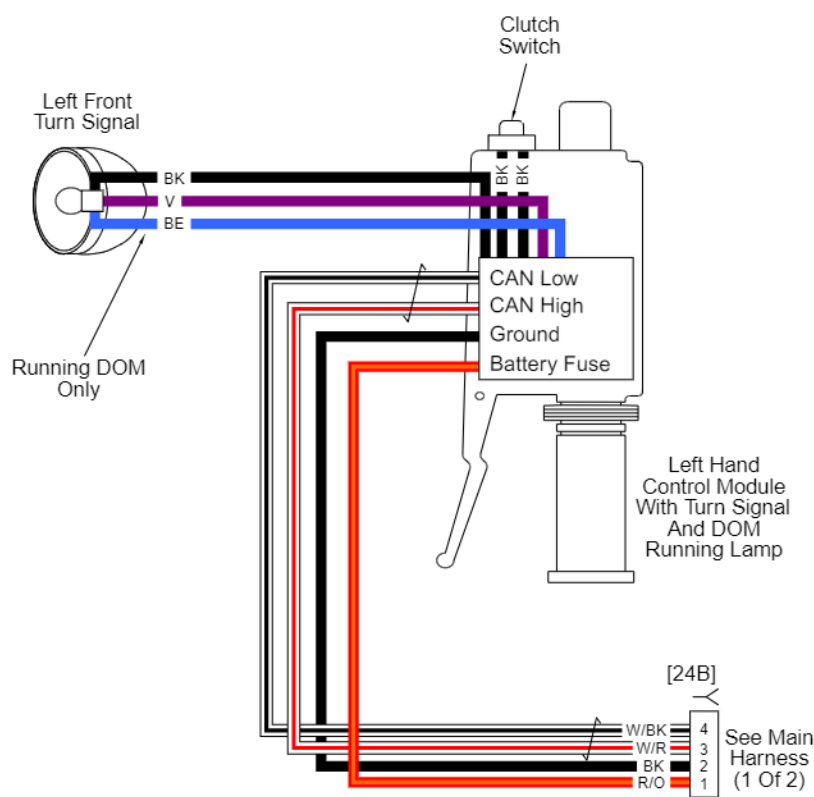
Front Lighting and Hand Controls: 2012 Dyna
