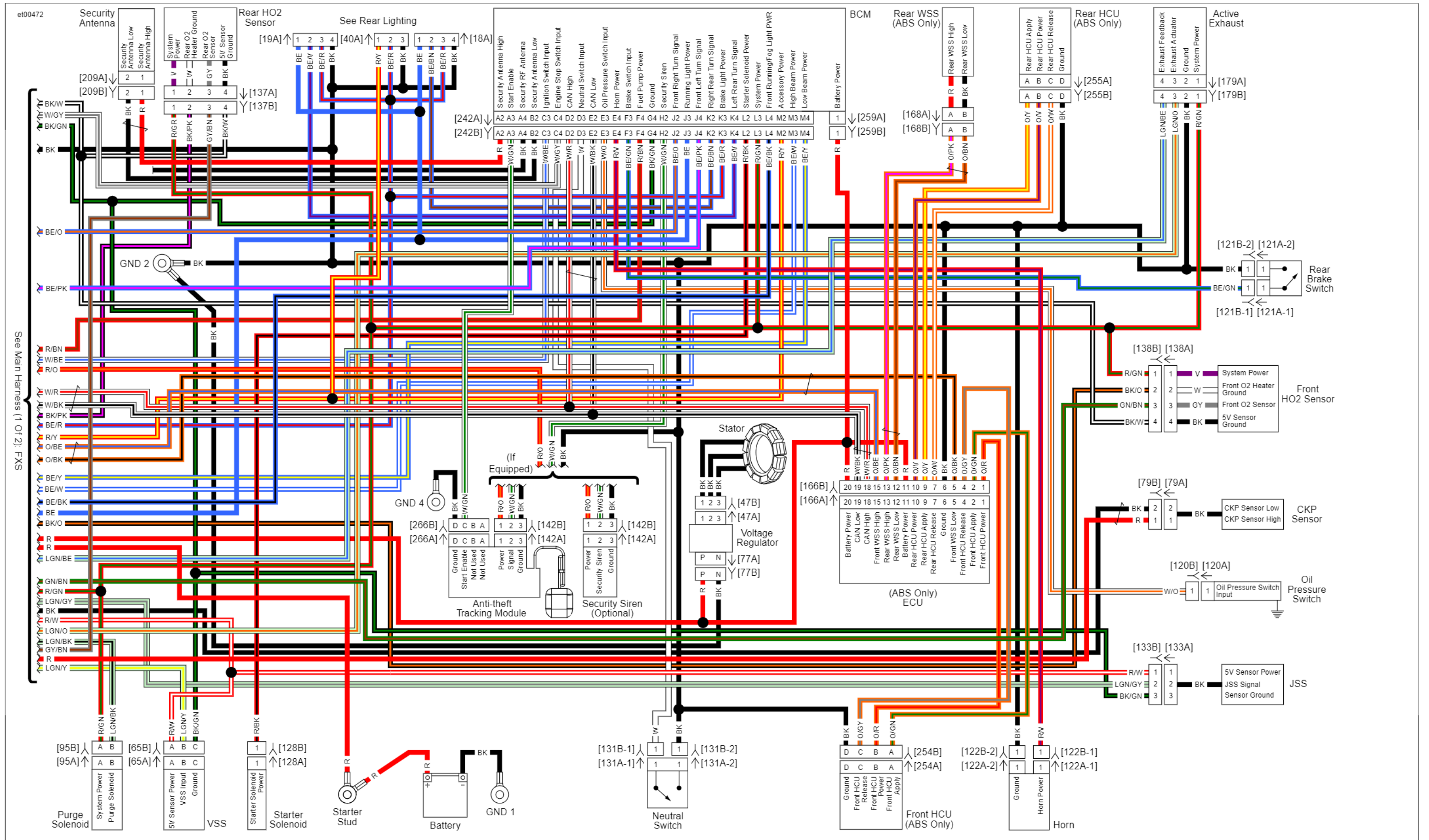
Main Harness 2 of 2: 2012 Softail (FXS)
