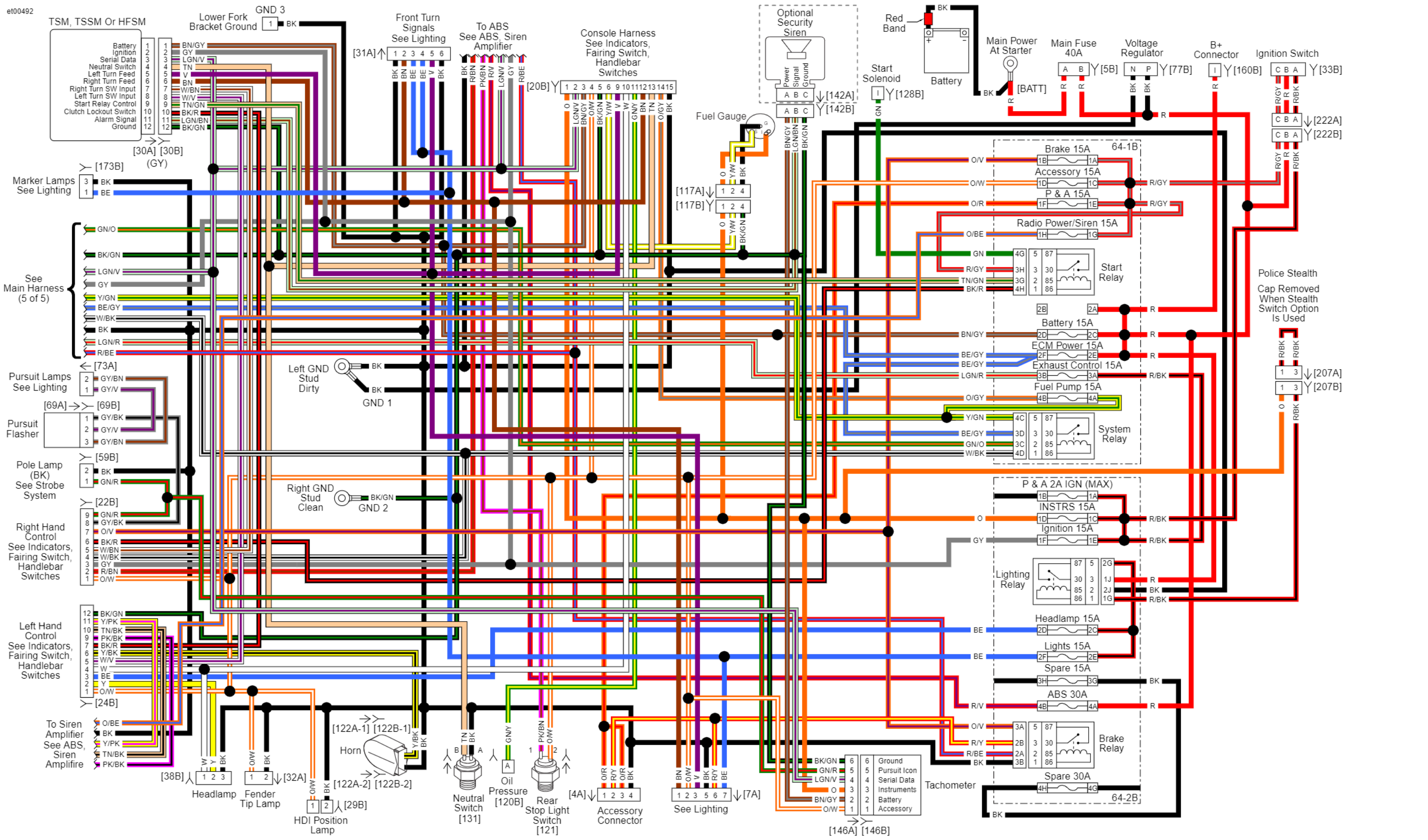
Main Harness (2 of 3): 2012 FLHP
