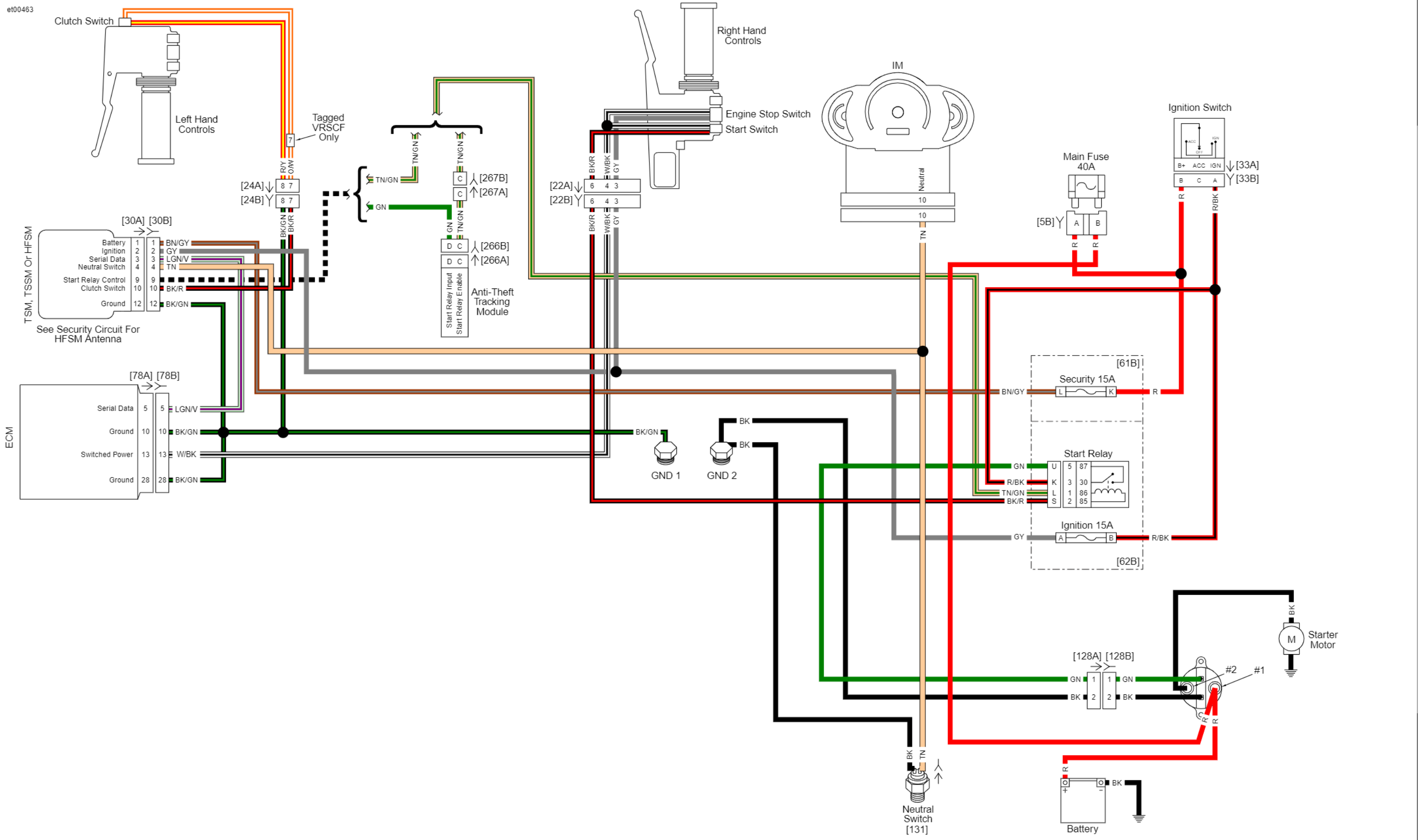
Starting Circuit: 2012 VRSC
