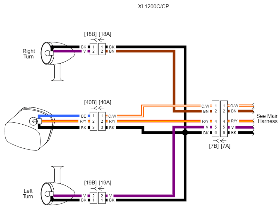
Dual Stop Lamp (Except DOM)
