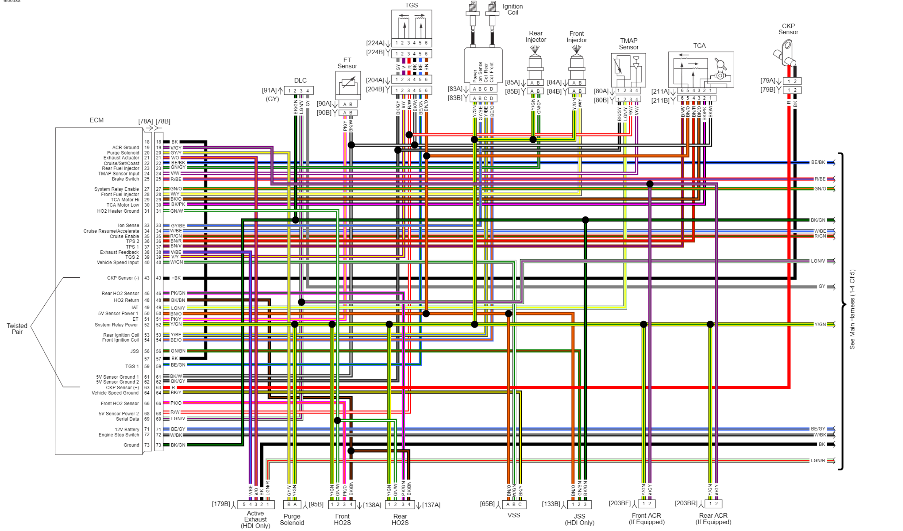
Main Harness (5 OF 5): 2012 Touring
