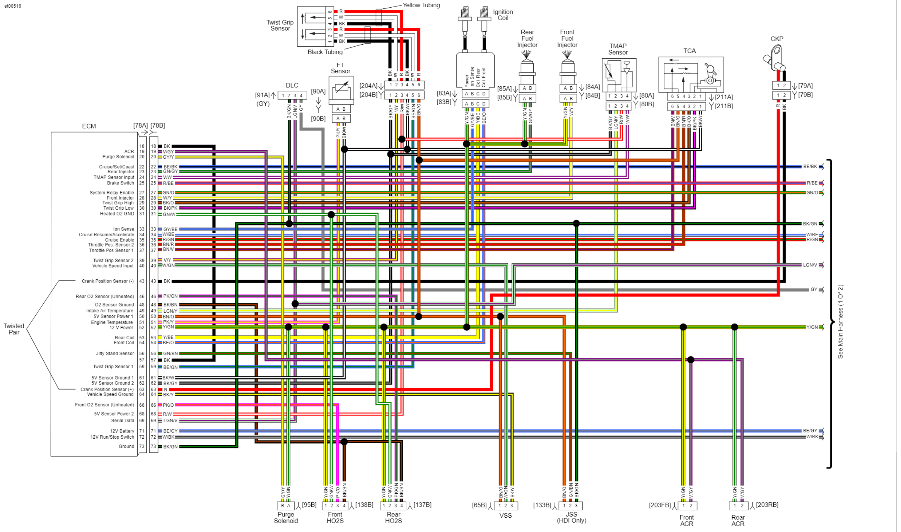
Main Harness (2 of 2): 2012 FLTRXSE
