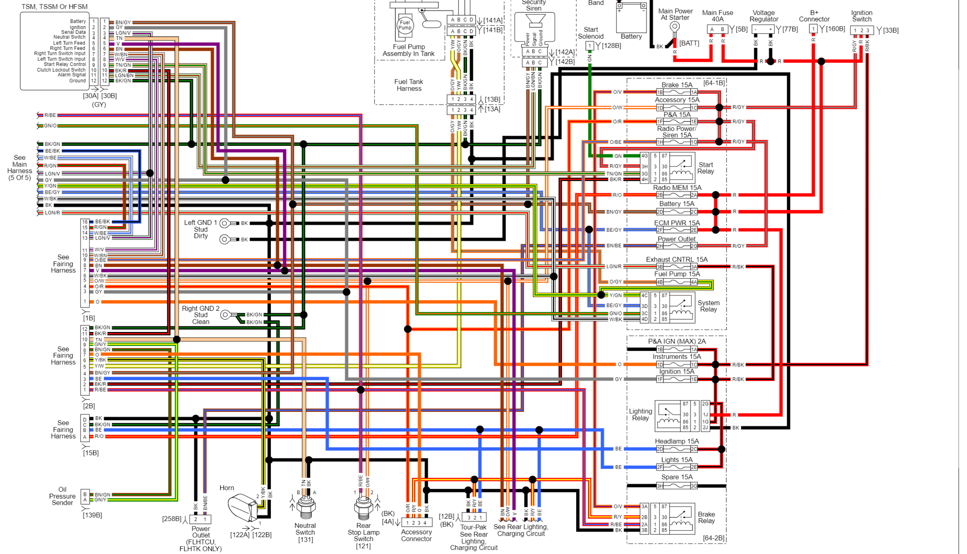
Main Harness (1 OF 5): 2012 Touring (Except FLHR/C) without ABS
