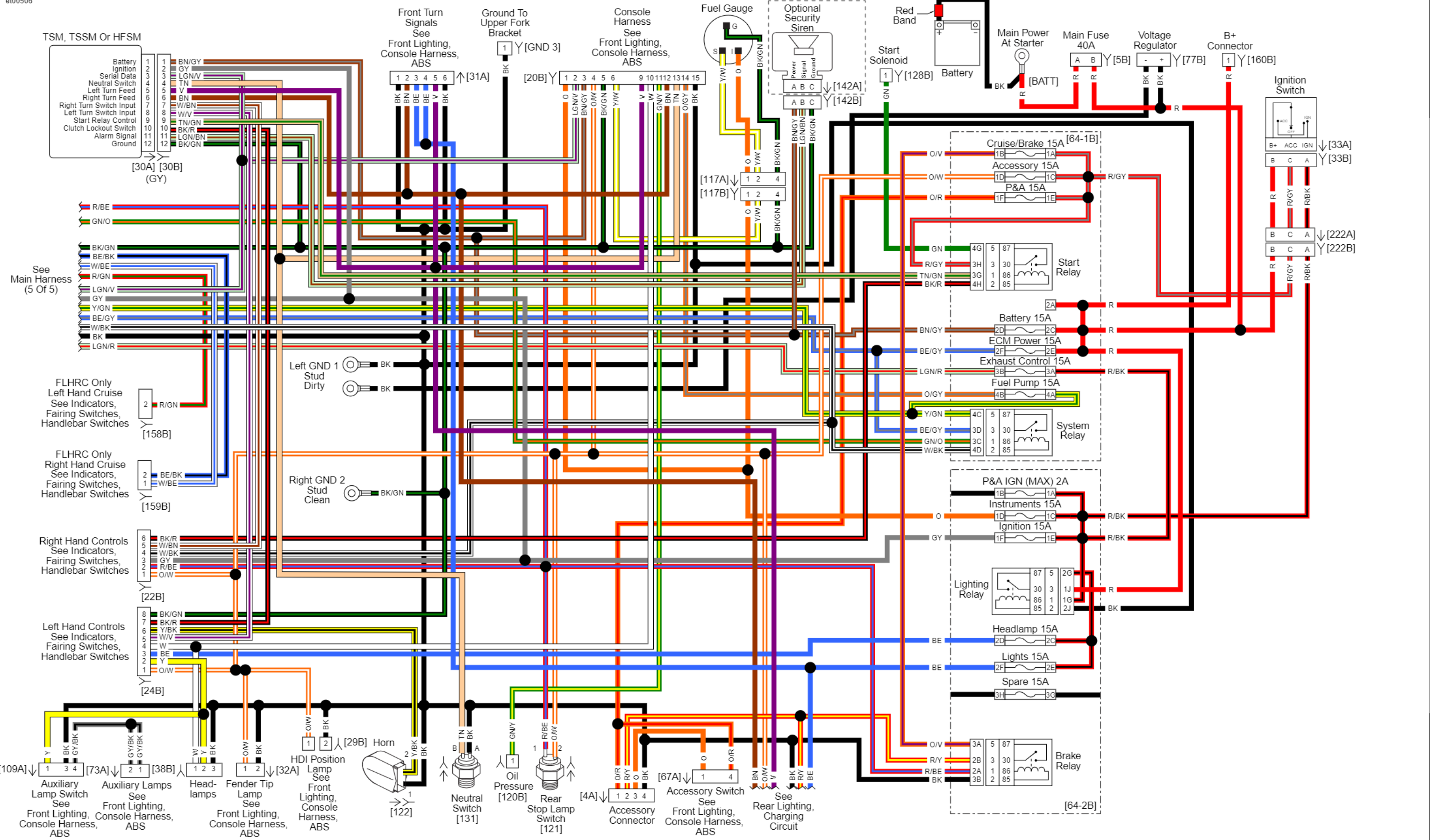
Main Harness (3 OF 5): 2012 Touring (FLHR/C) without ABS
