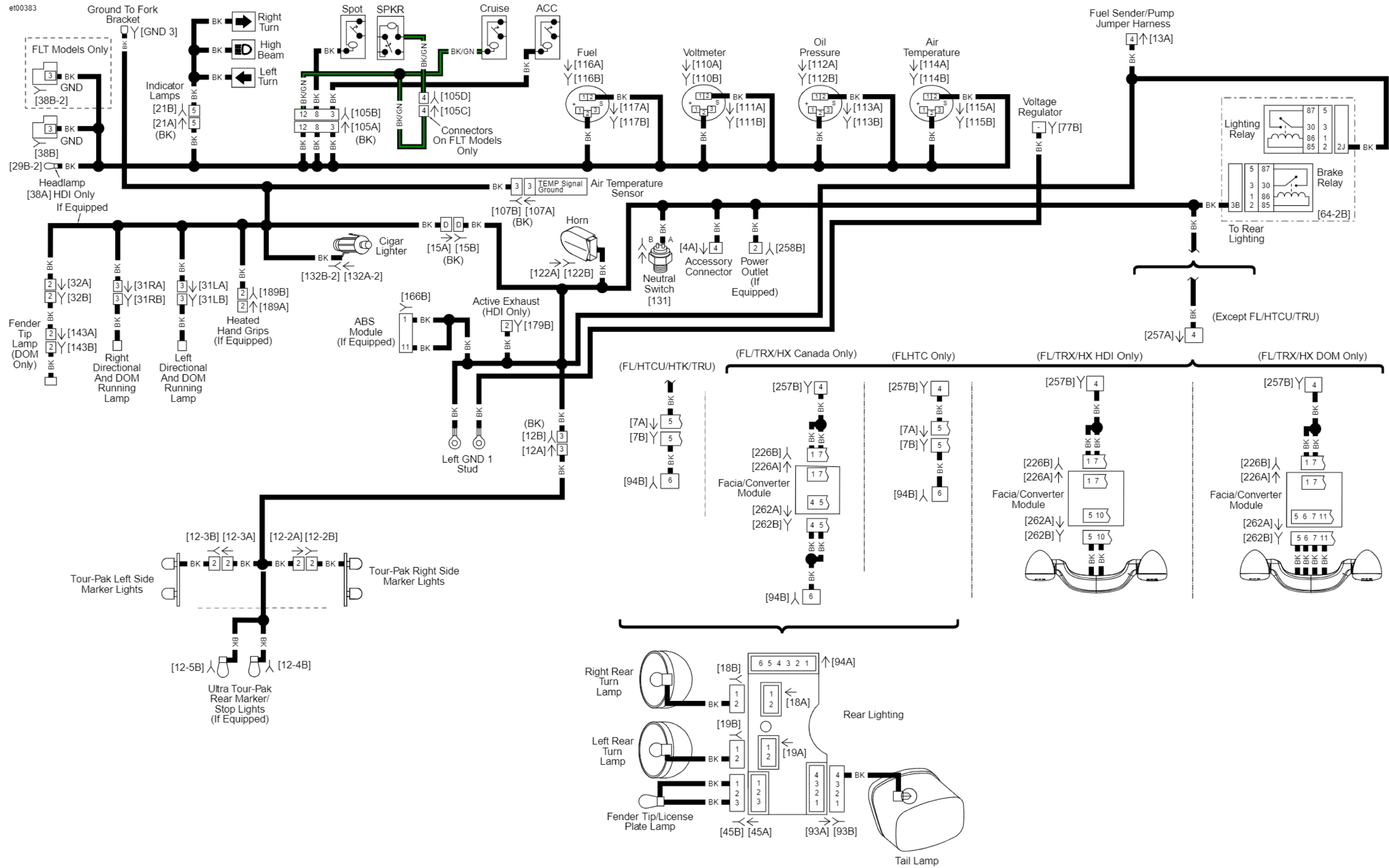
Left GND1: 2012 Touring (Except FLHR/C)
