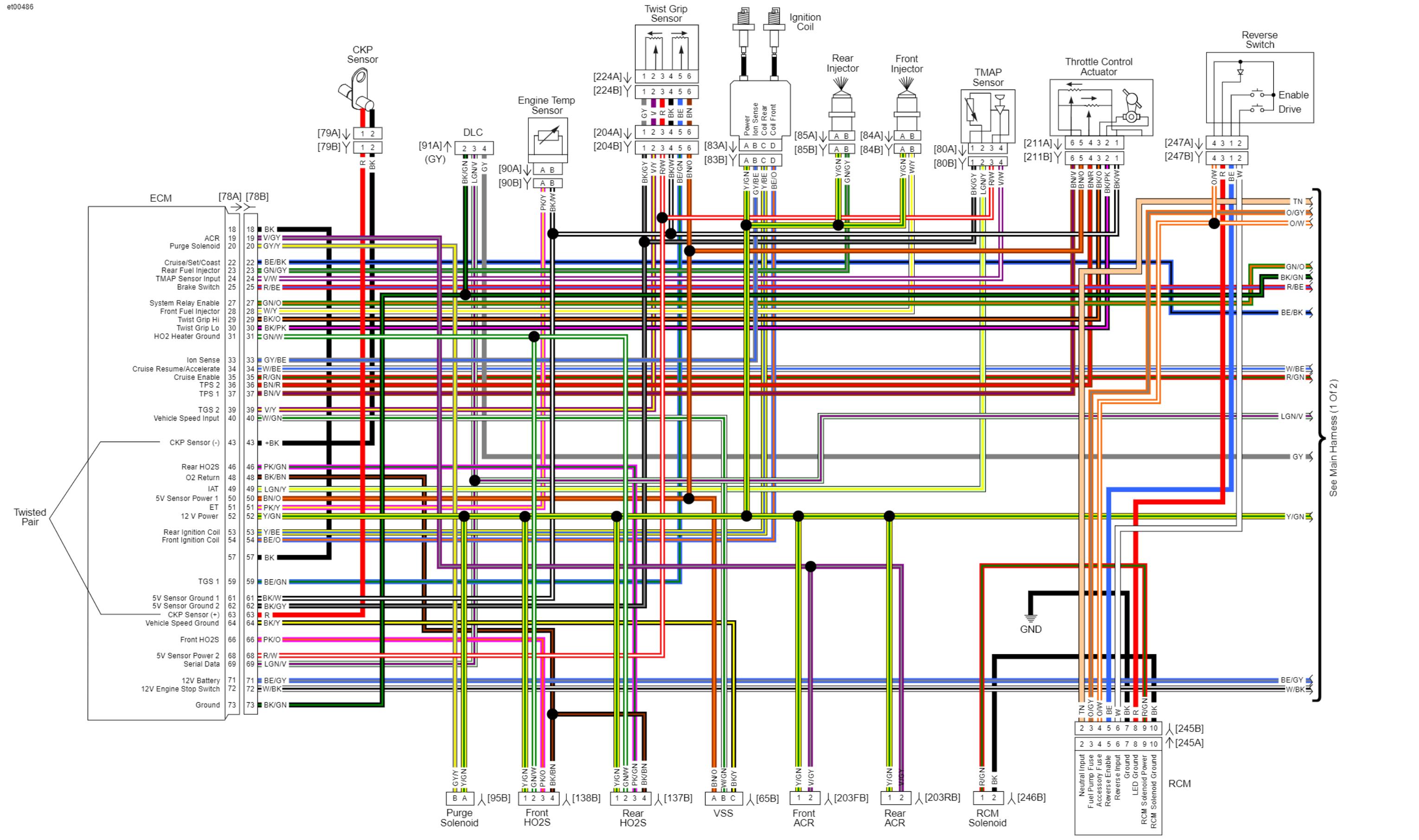
Main Harness (2 of 2): 2012 Trike Models
