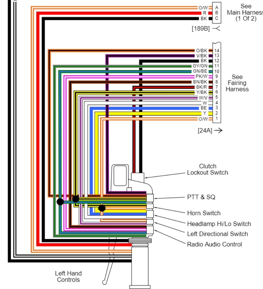
Indicators, Fairing Switches, Handlebar Switches, ABS: 2012 FLHTCUSE7
