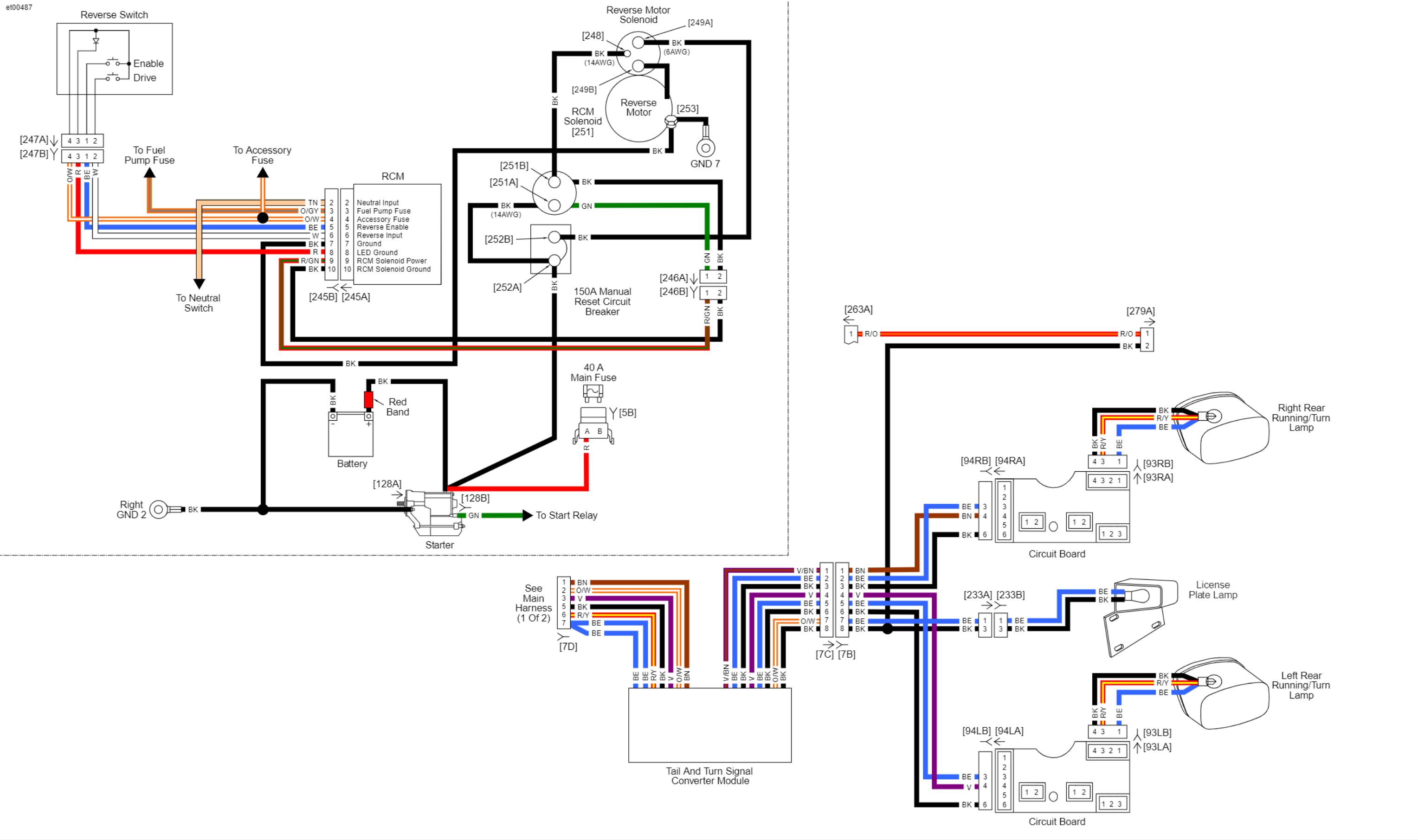
Reverse, Rear Lighting: 2012 Trike Models
