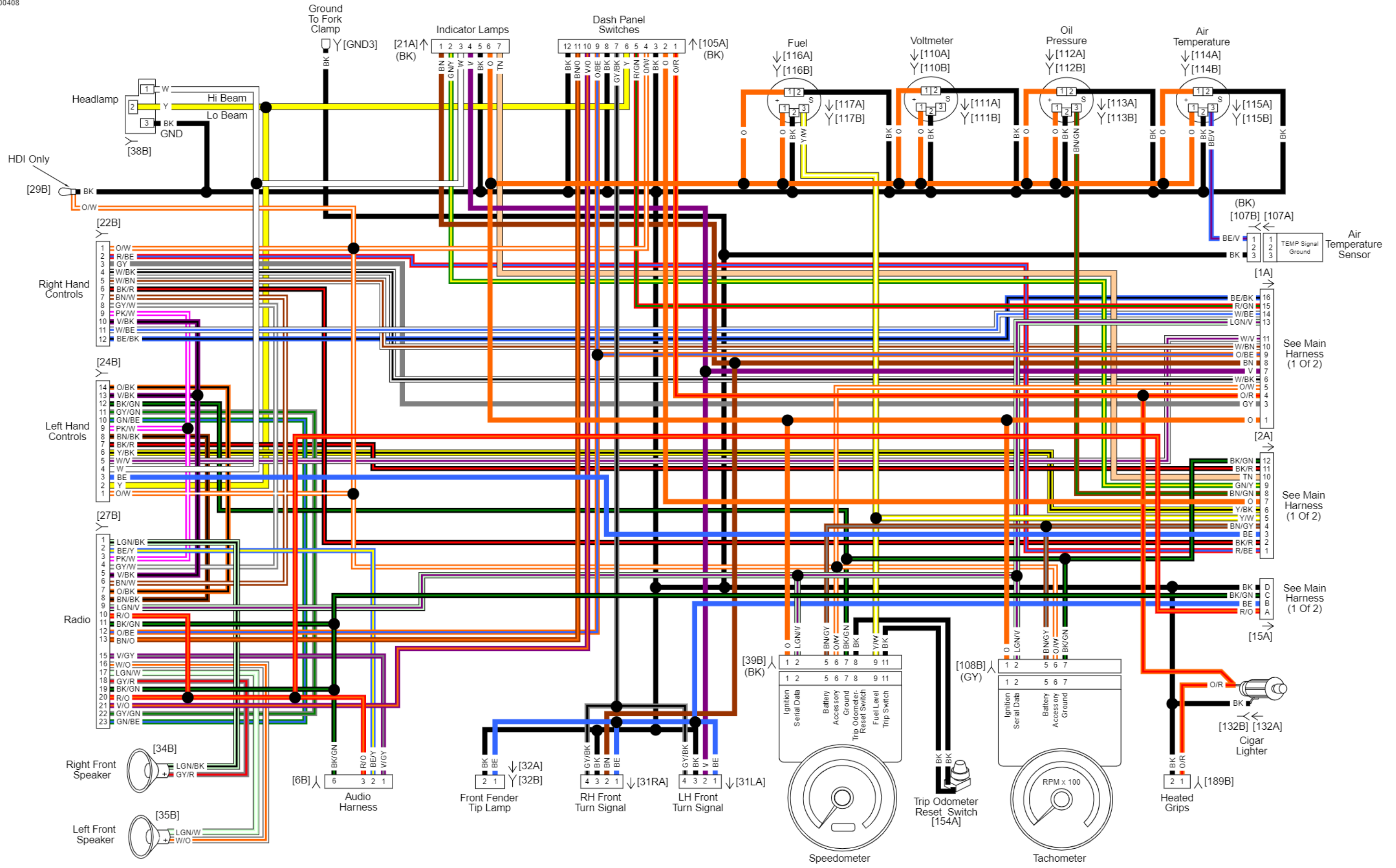
Fairing Harness: 2012 Trike Models
