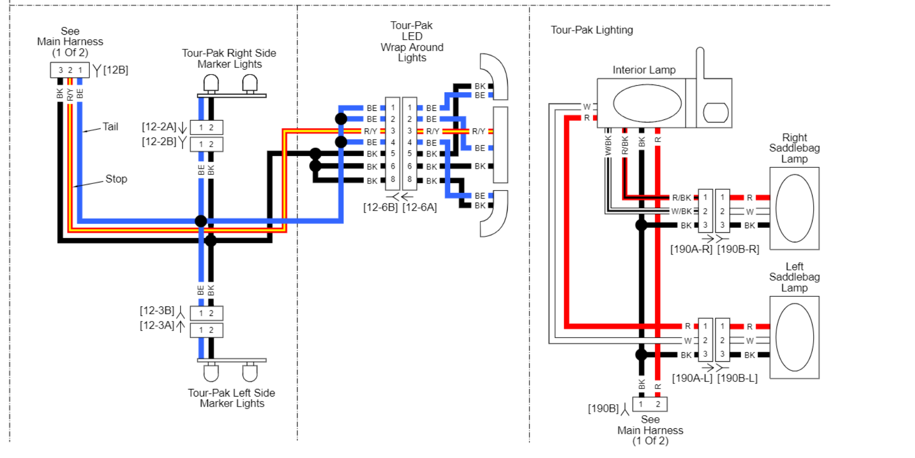
Lighting, Garage Door Opener: 2012 FLHTCUSE7
