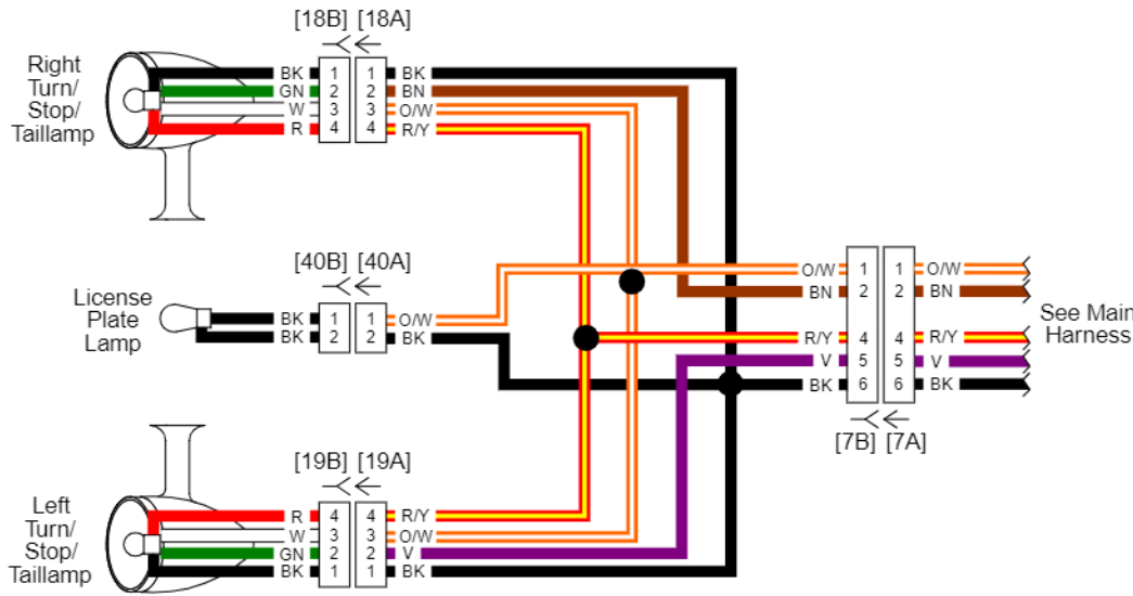
Dual Stop Lamp (Except DOM)
