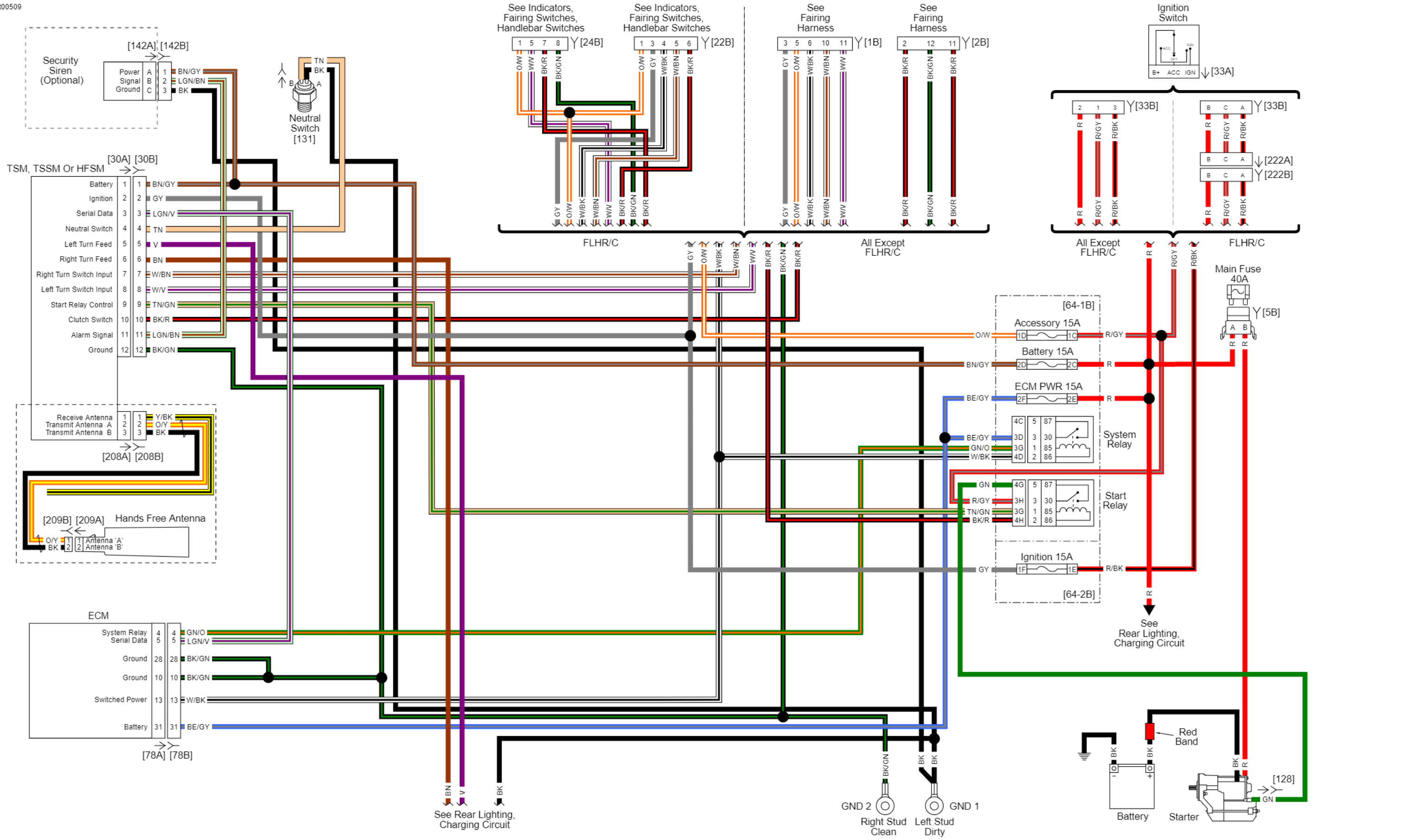
Security Circuit: 2012 Touring
