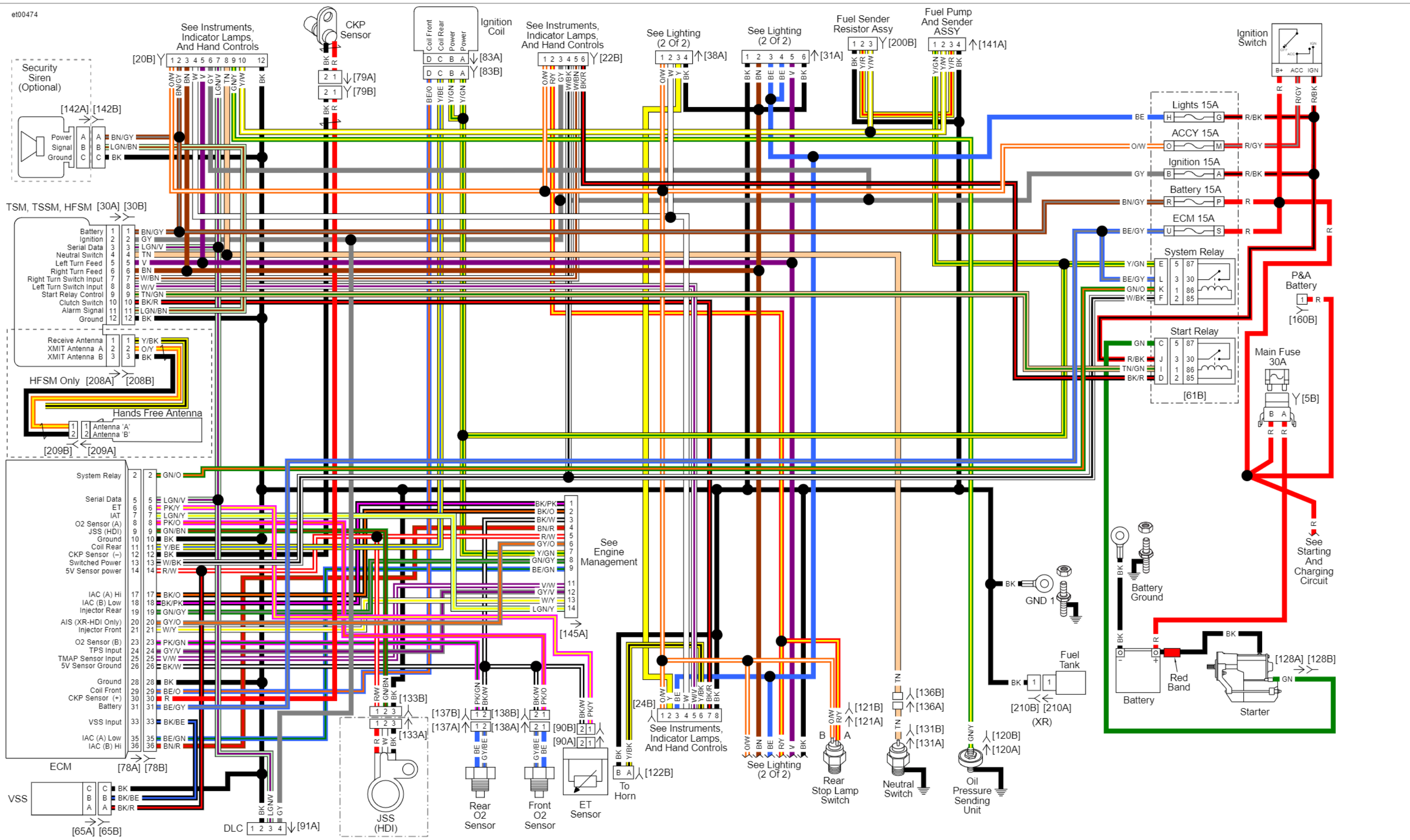
Main Harness: 2012 Sportster
