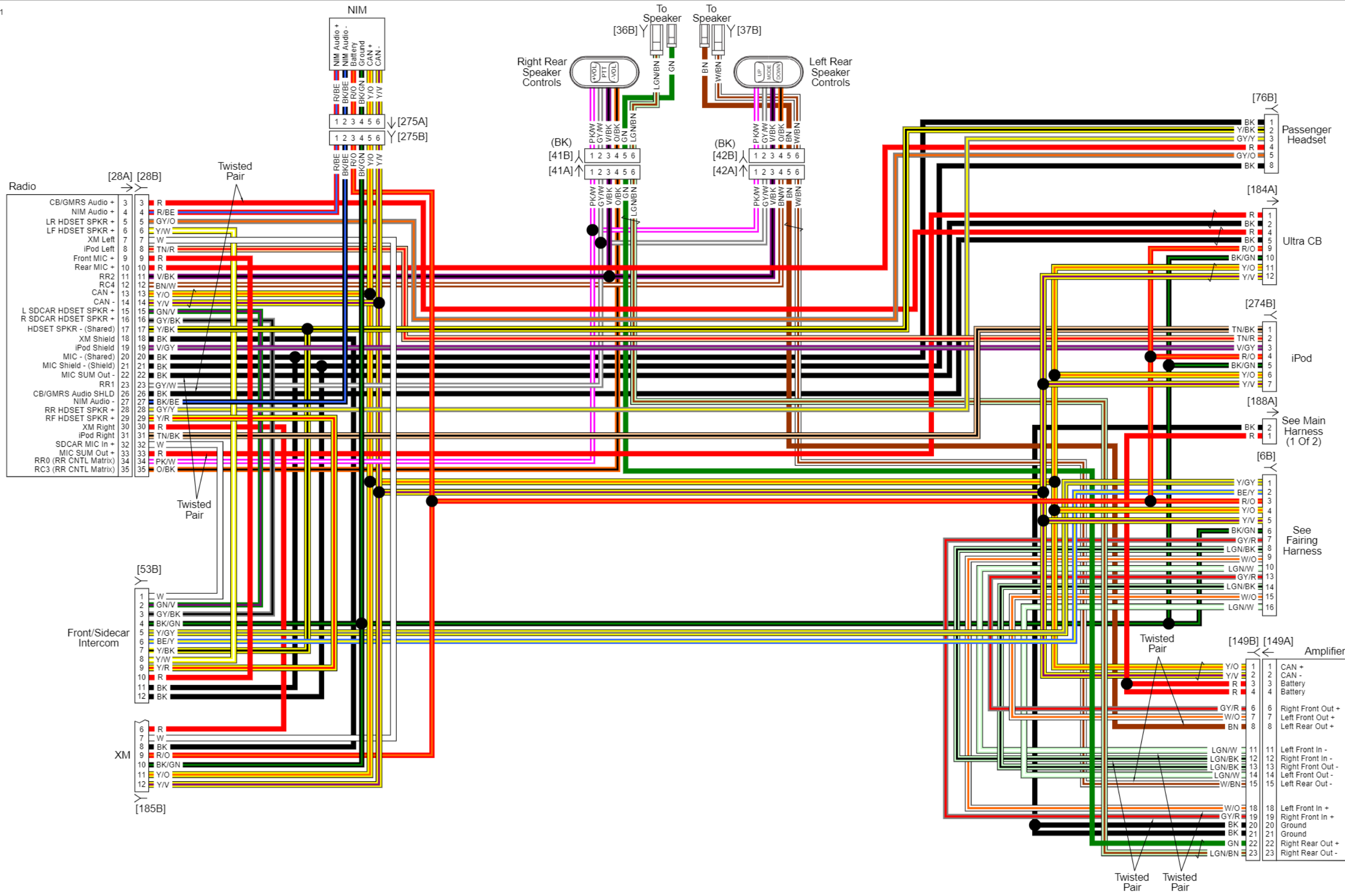
Audio Overlay Harness: 2012 FLHTCUSE7
