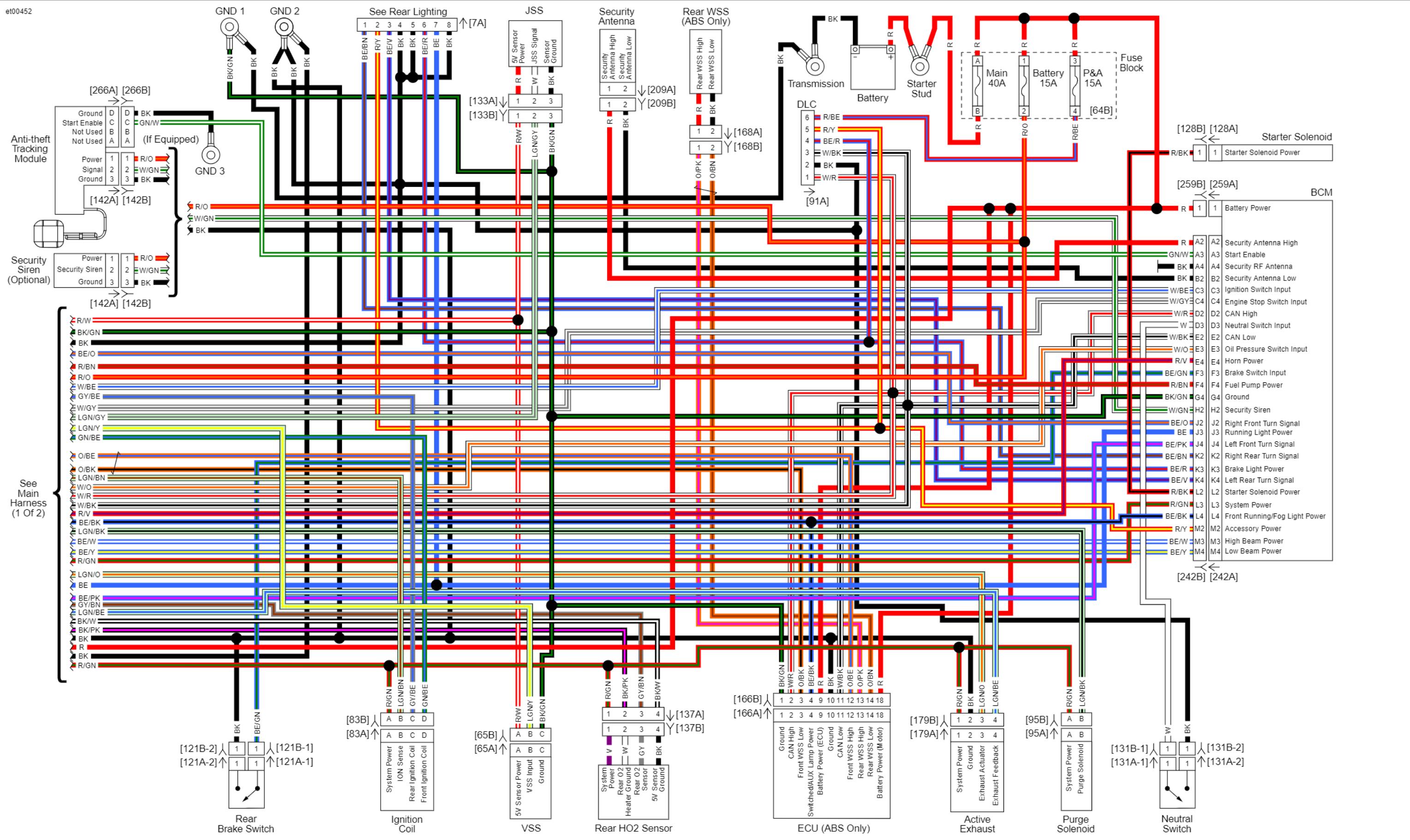
Main Harness 2 of 2: 2012 Dyna
