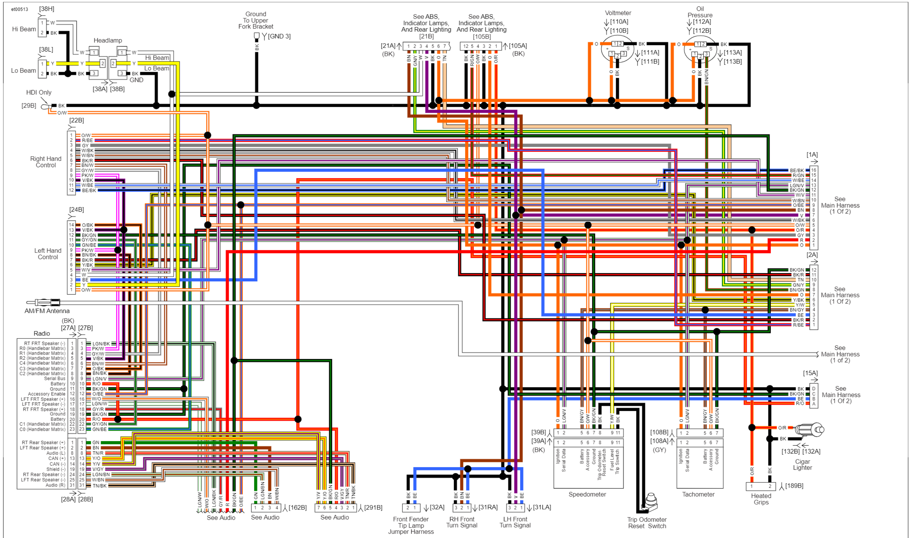
Fairing Harness: 2012 FLHXSE3
