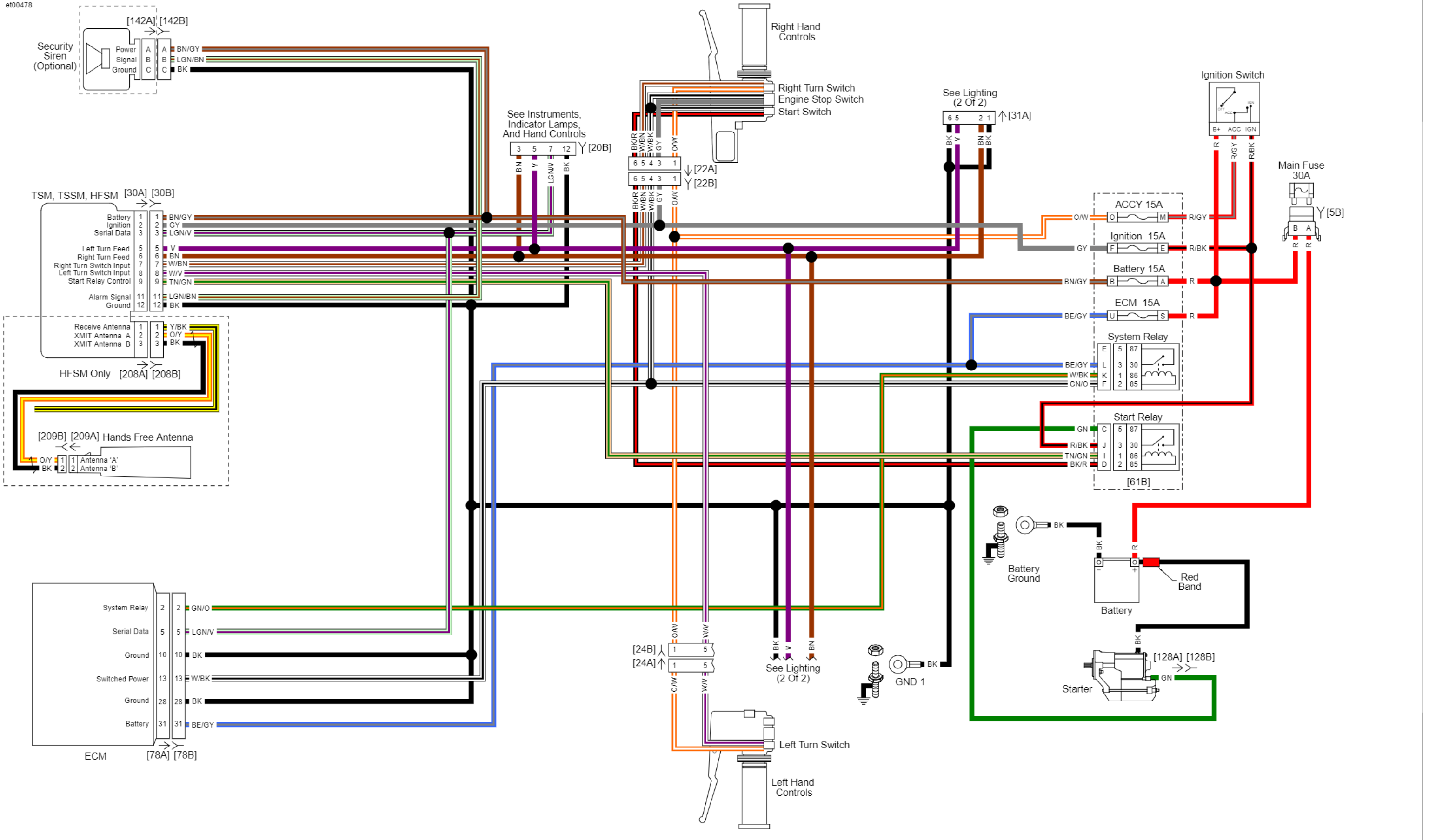
Security Circuit: 2012 Sportster
