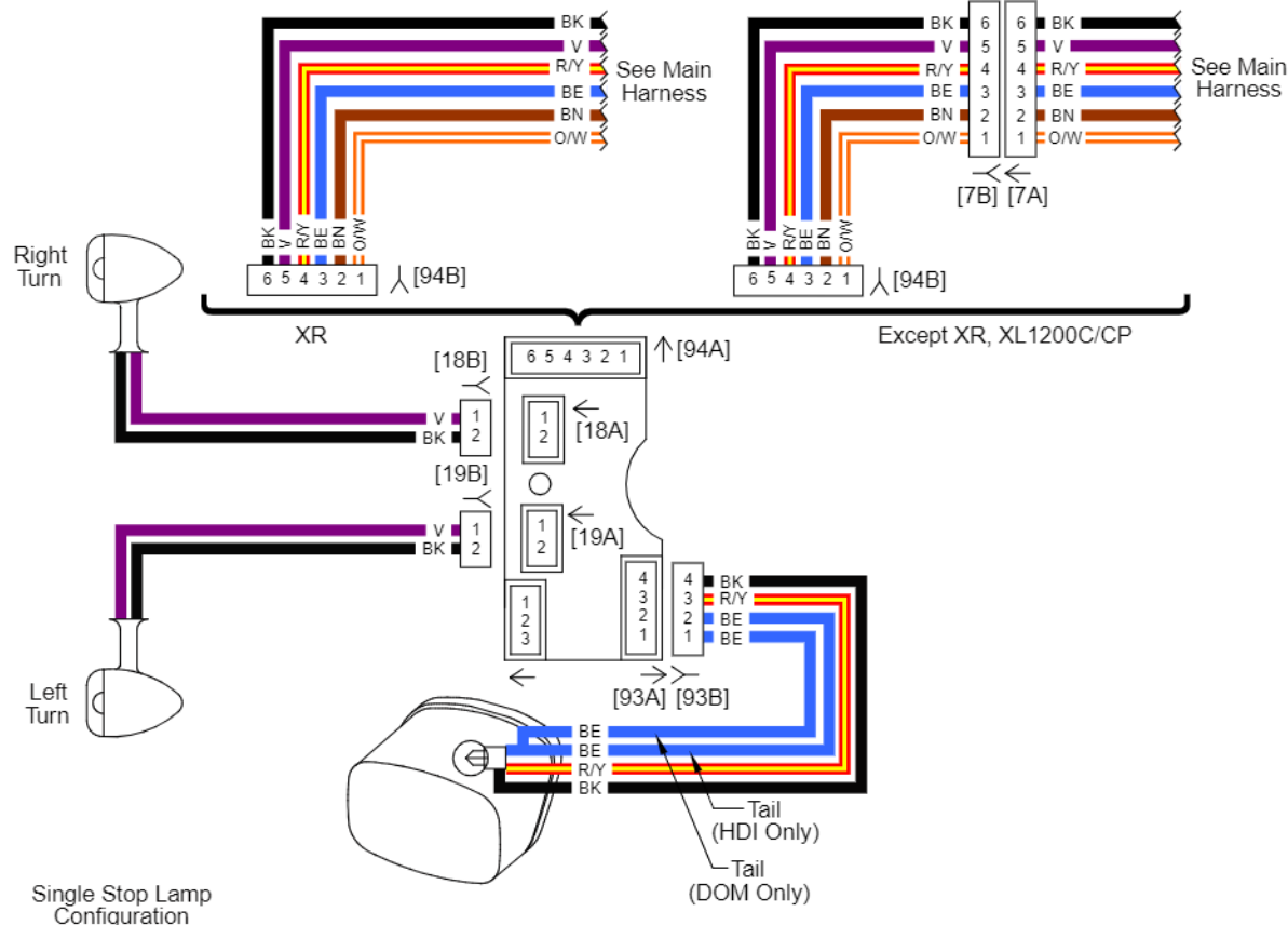
Lighting (2 of 2): 2012 Sportster
