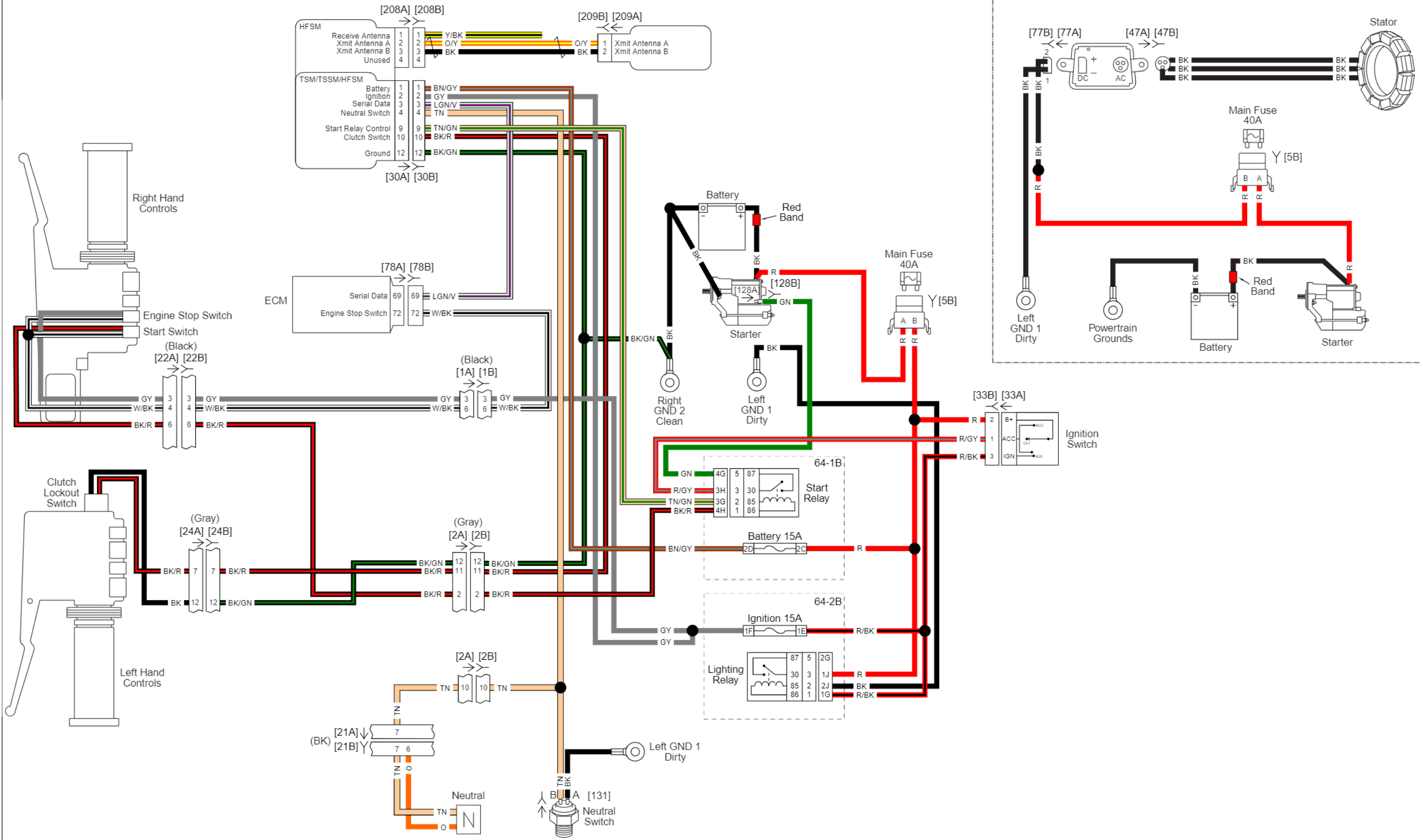
Starting and Charging System: 2012 FLHTCUSE7
