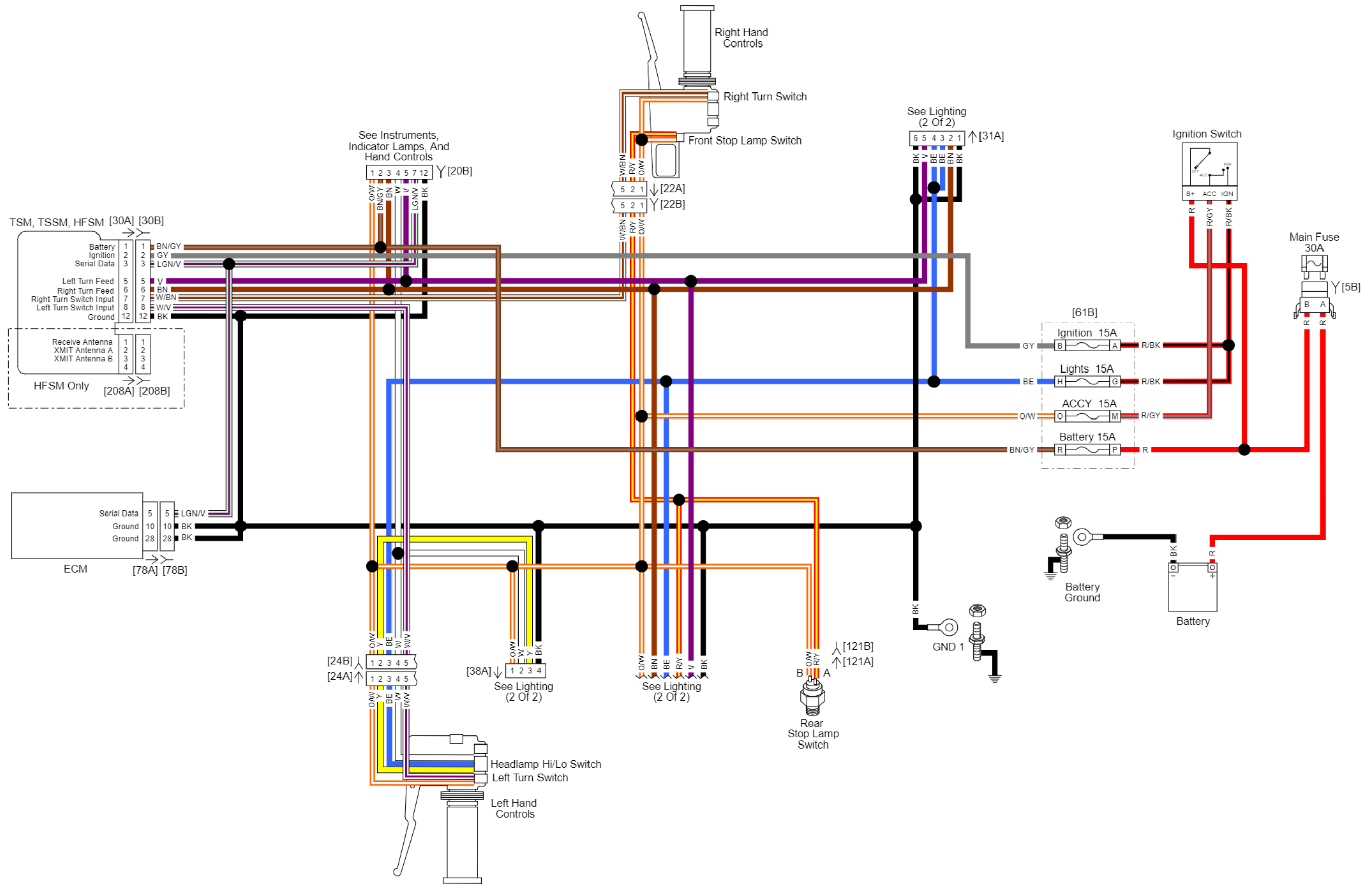
Lighting (1 of 2): 2012 Sportster
