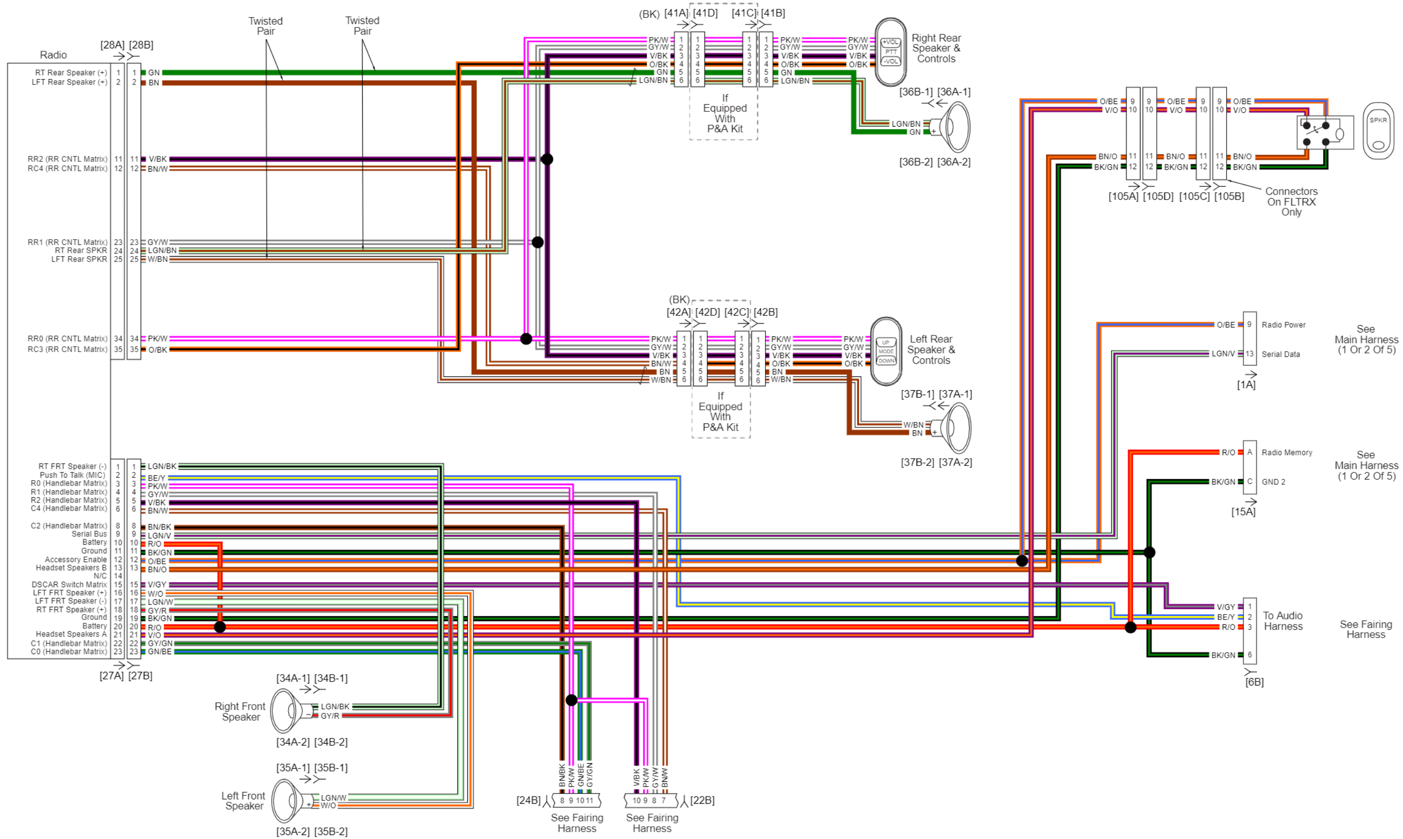
Classic Radio Circuit: 2012 Touring
