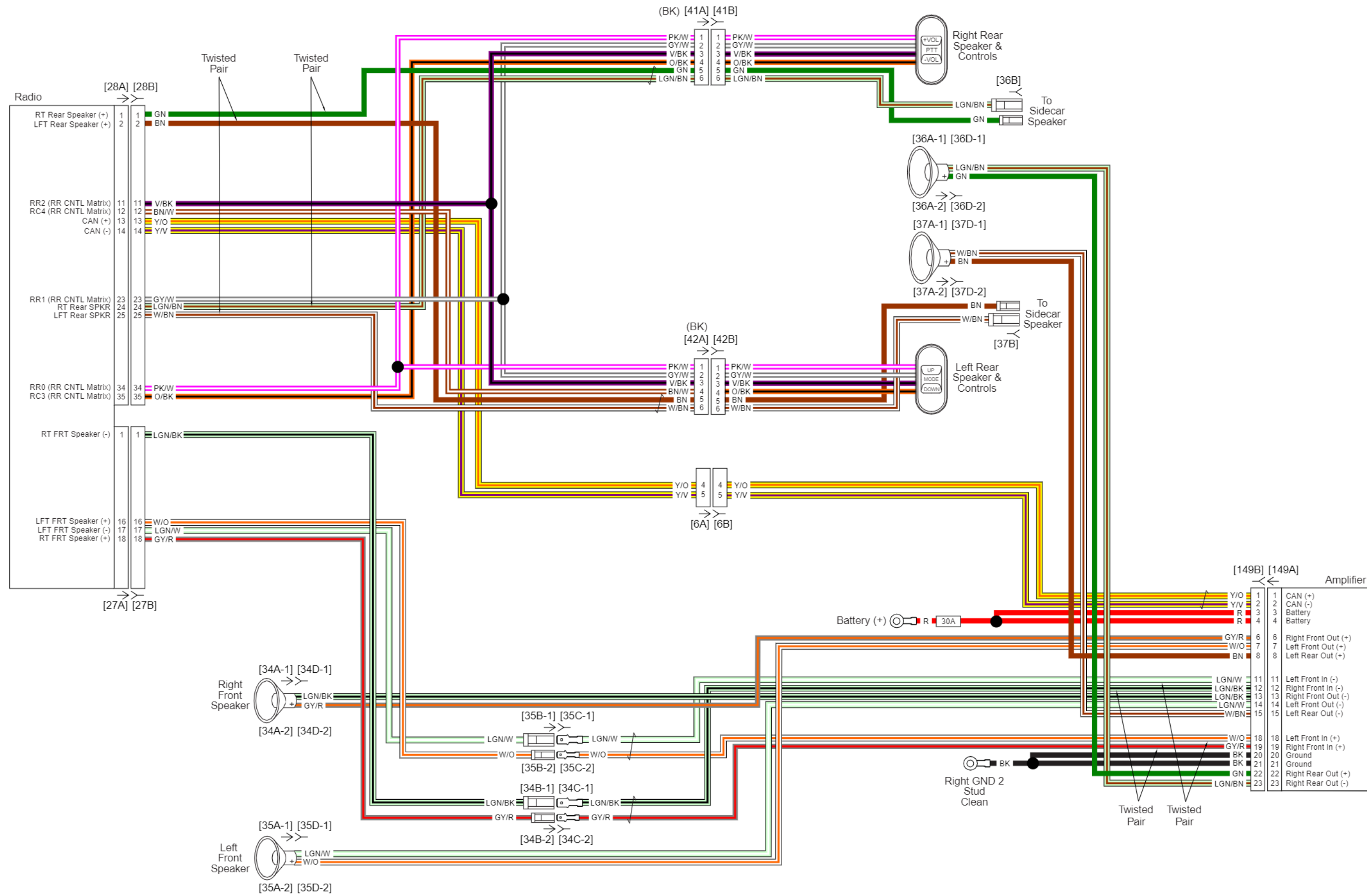
Ultra Radio Circuit: 2012 Touring
