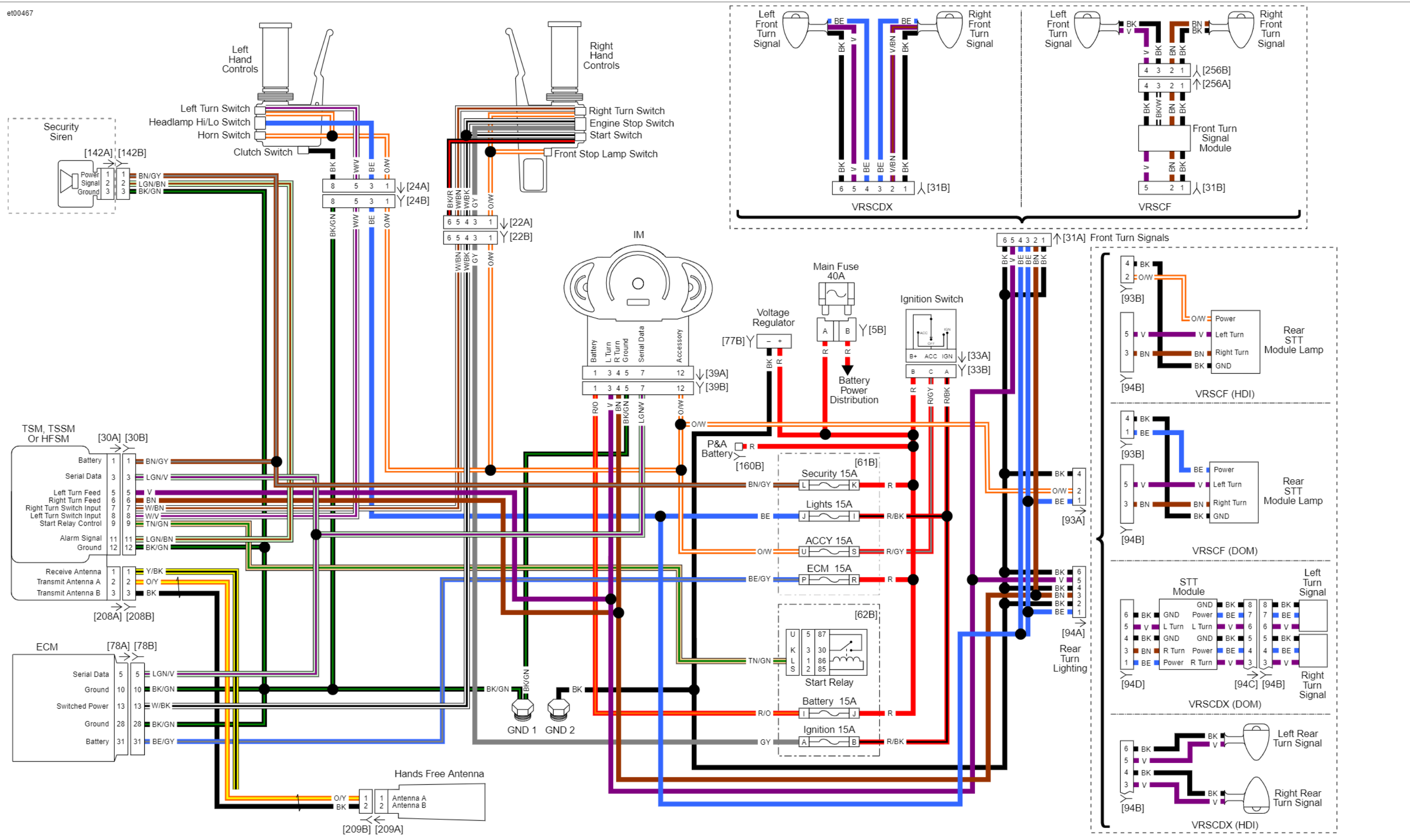
Security Circuit Without Anti-Theft Tracking Module: 2012 VRSC
