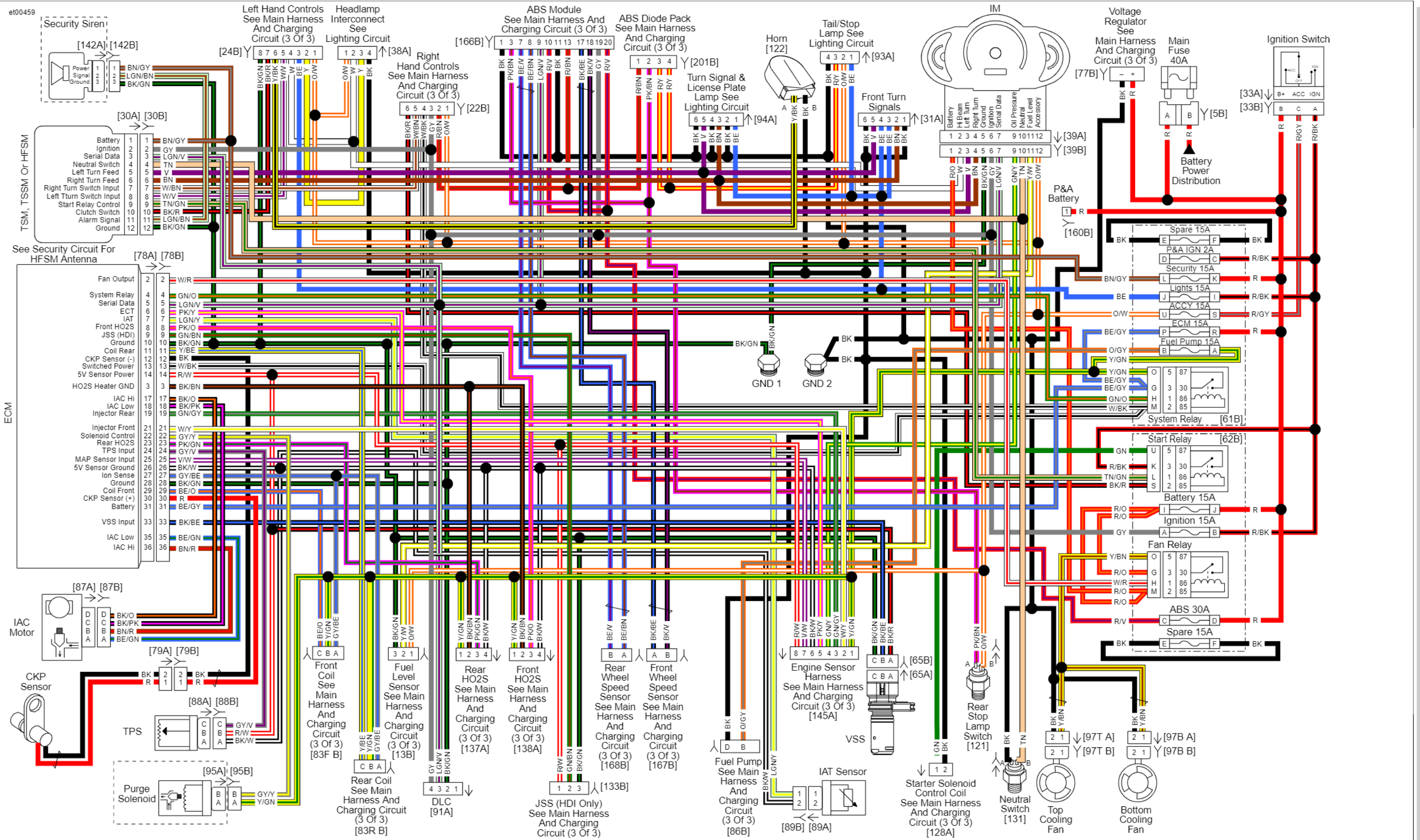
Main Harness (1 of 3): 2012 VRSC with ABS
