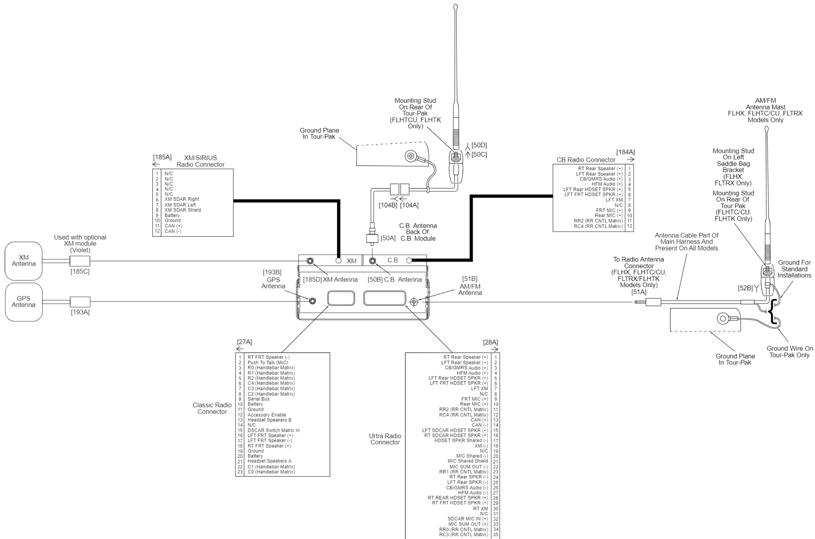
Ultra Radio RF Interconnect Circuit: 2012 Touring
