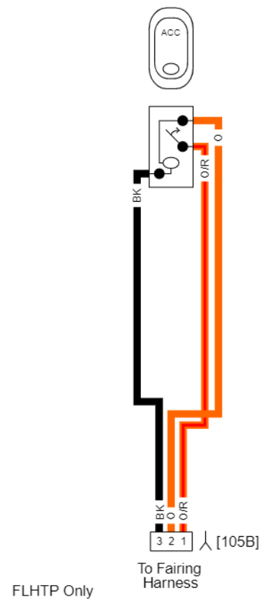
Indicators, Fairing Switch and Handlebar Switches: 2012 FLHTP, FLHP
