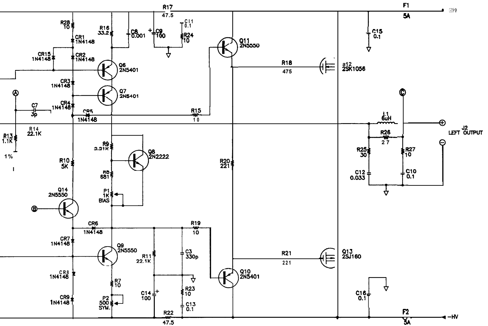
) CIRCUIT SCHEMATIC DIAGRAM REVISED 9/3/92
