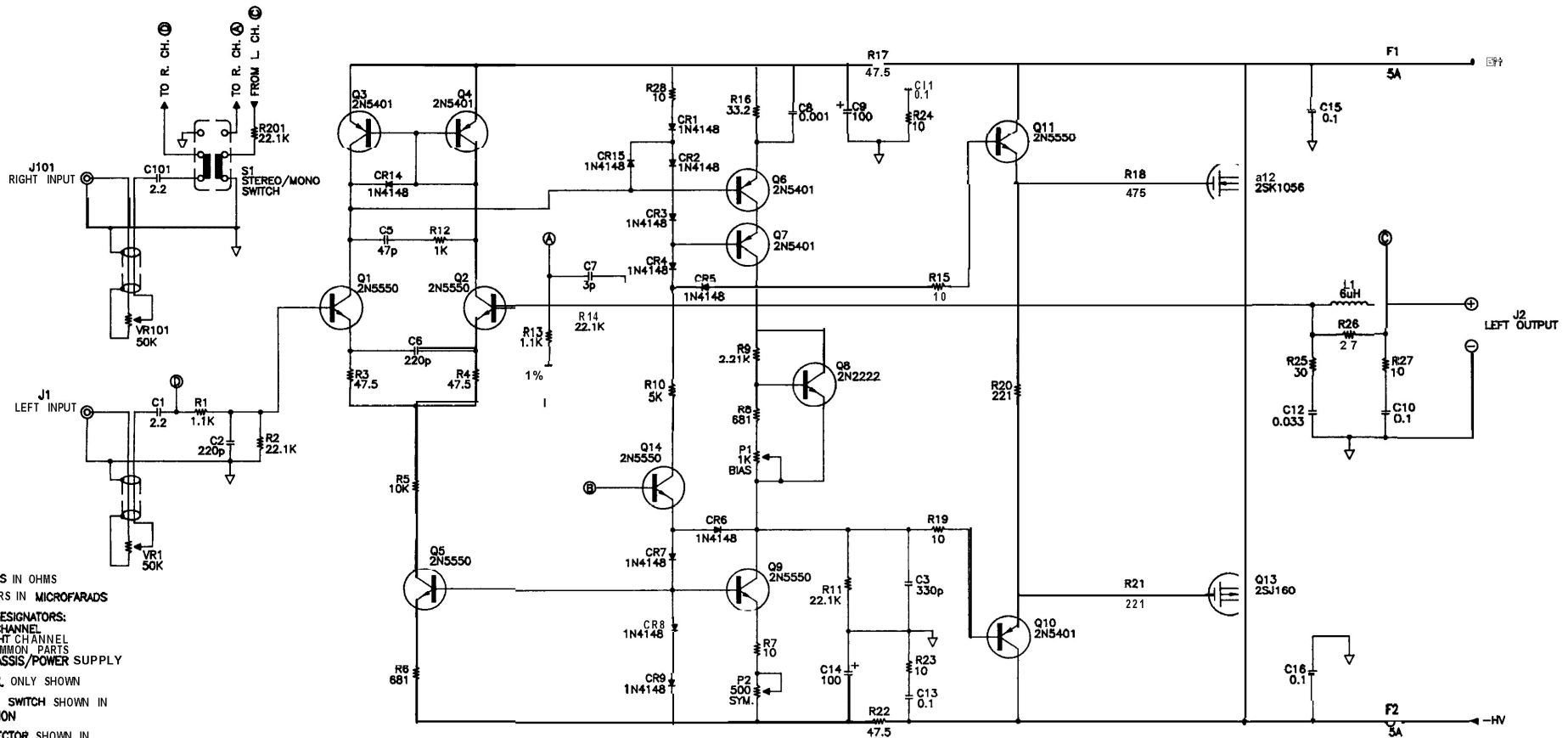
9 130) CIRCUIT SCHEMATIC DIAGRAM REVISED 9/3/92
