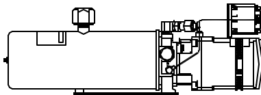
SIDE VIEW PUMP/MANIFOLD-AP7337
