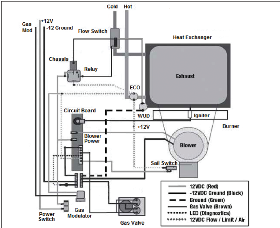
Figure 10 - WIRING DIAGRAM
