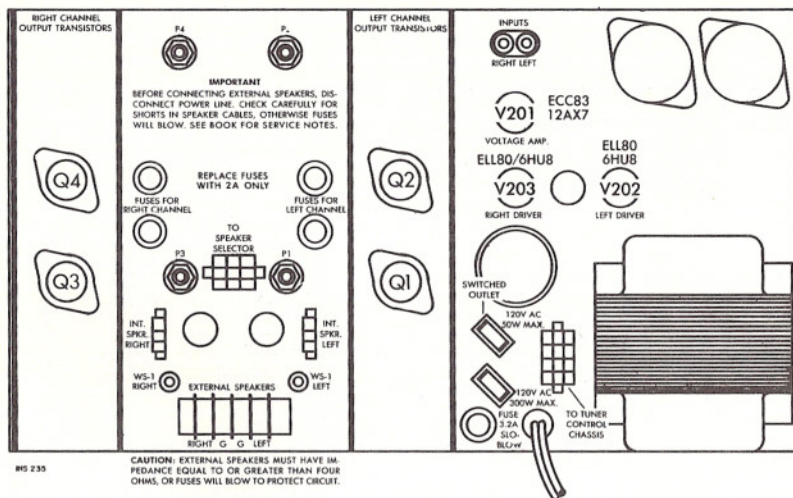
FIGURE 4. Chassis Layout of Power Amplifier Section
