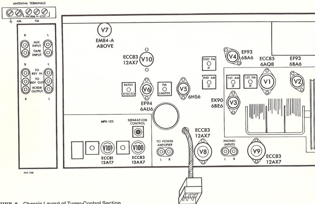
FIGURE 3. Chassis Layout of Tuner-Control Section
