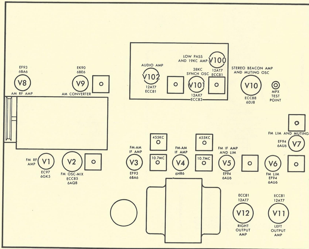
FIGURE 6. Tube layout chart of the Tunes
