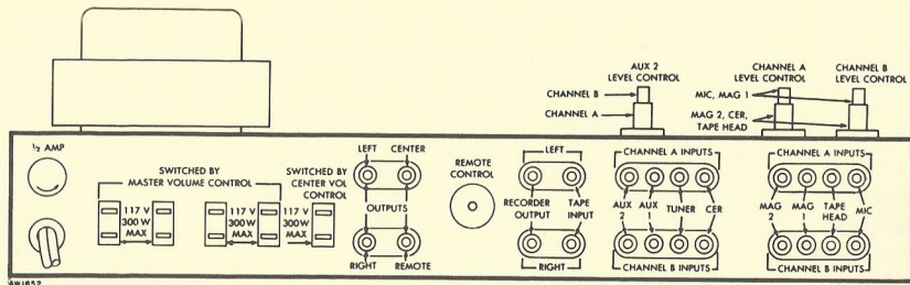
FIGURE 2. Rear panel of the Master Audio Control
