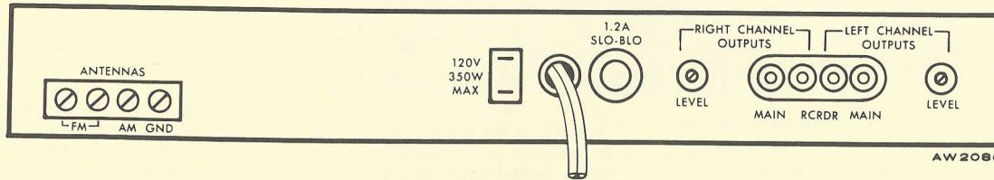
FIGURE 3. Rear panel of the Tuner
