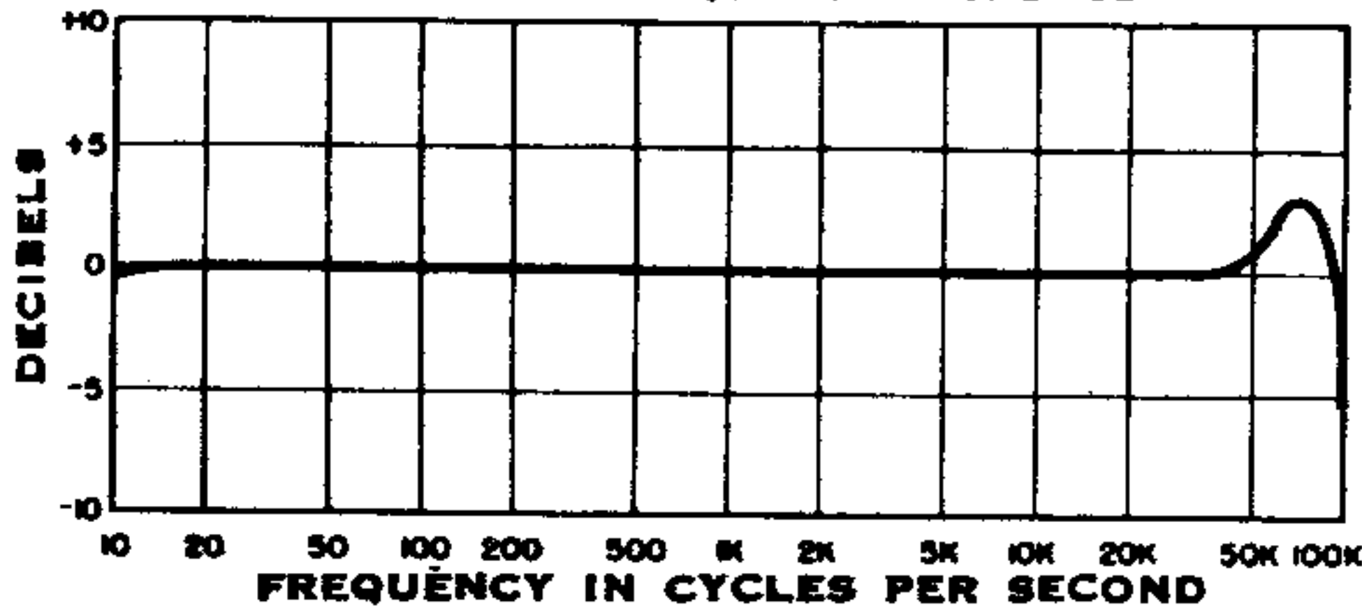
FIGURE 2. FREQUENCY RESPONSE
