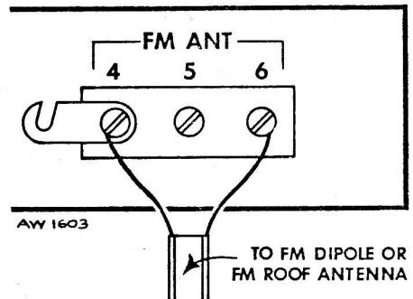
FIG. 3: Connections and position of link for installing an FM antenna in a strong signal area.
