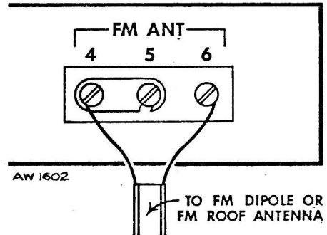
FIG. 1: Connections to antenna terminal strip for FM and AM reception, as wired at factory
