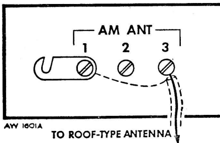
FIG. 2: Terminal connections for installing a roof-type AM antenna. The link between terminals 1 and 2 is detached.
