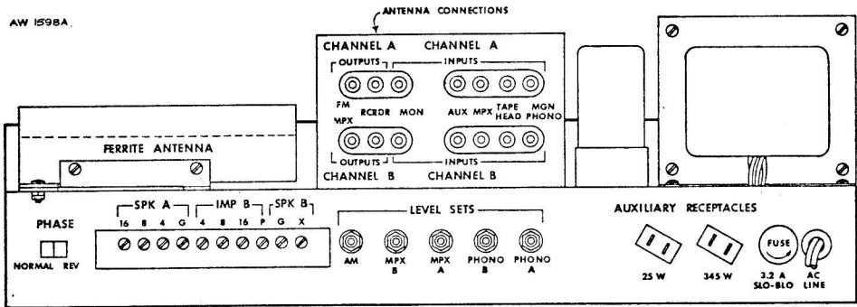
FIG. 5: Rear panel of the receiver chassis showing location of jack bracket for making connections to external equipment.
