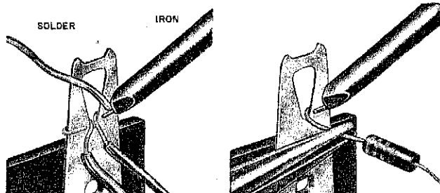
B. APPLY SOLDER TO LUG, WIRE AND IRON
