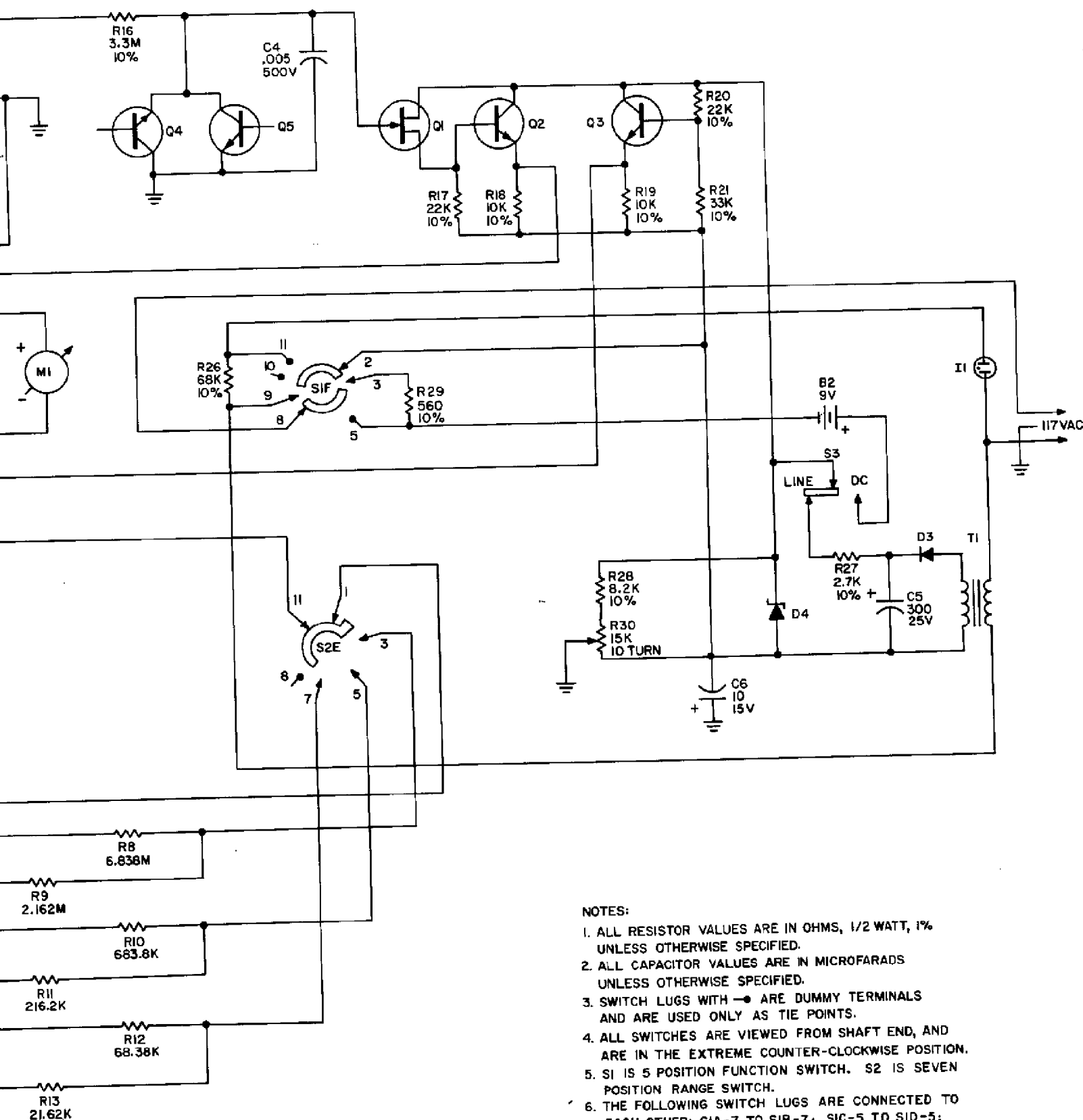
SCHEMATIC DIAGRAM
