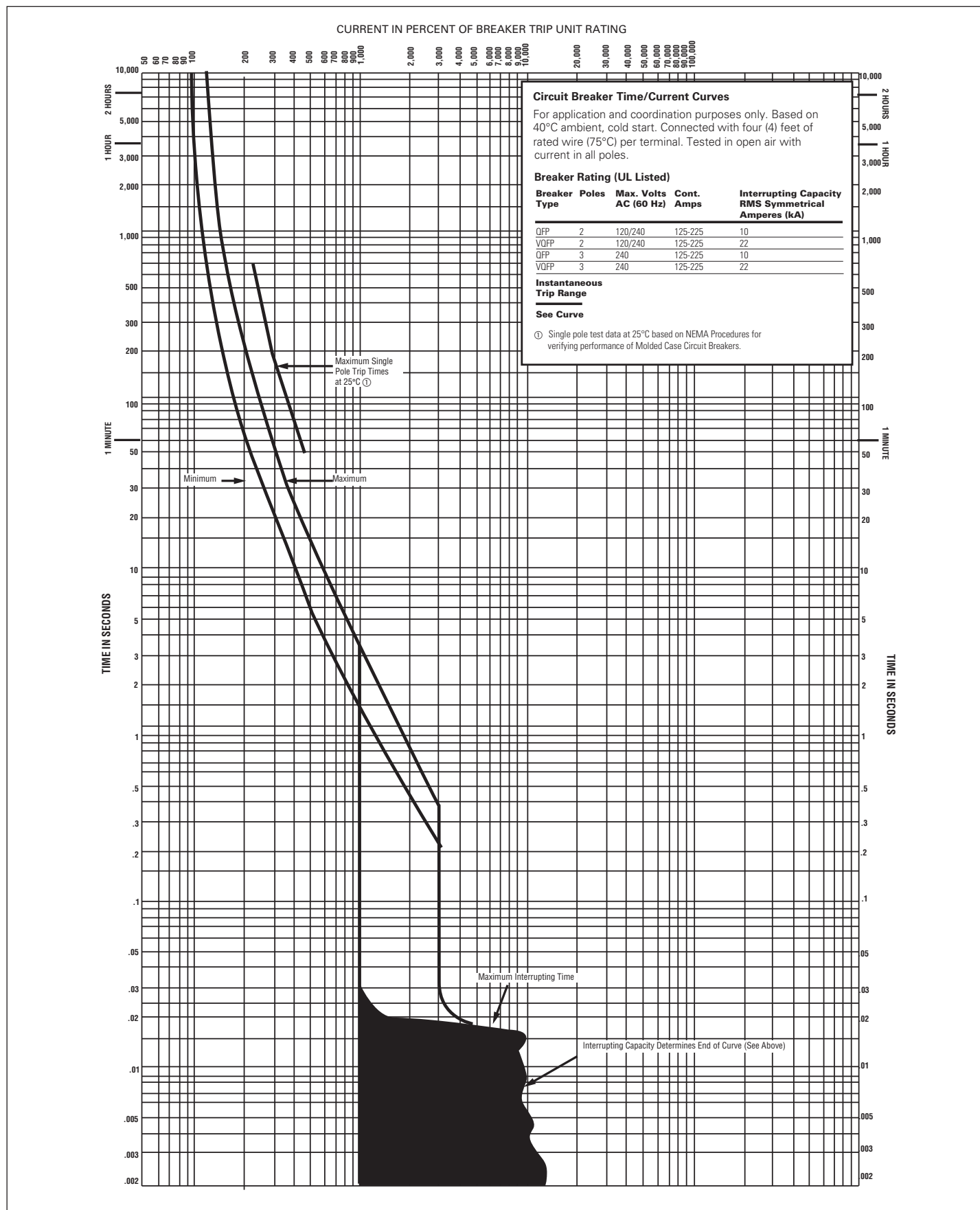
Figure 6. Types QFP, VQFP - 125–225 Amperes, 2 and 3 Poles.
