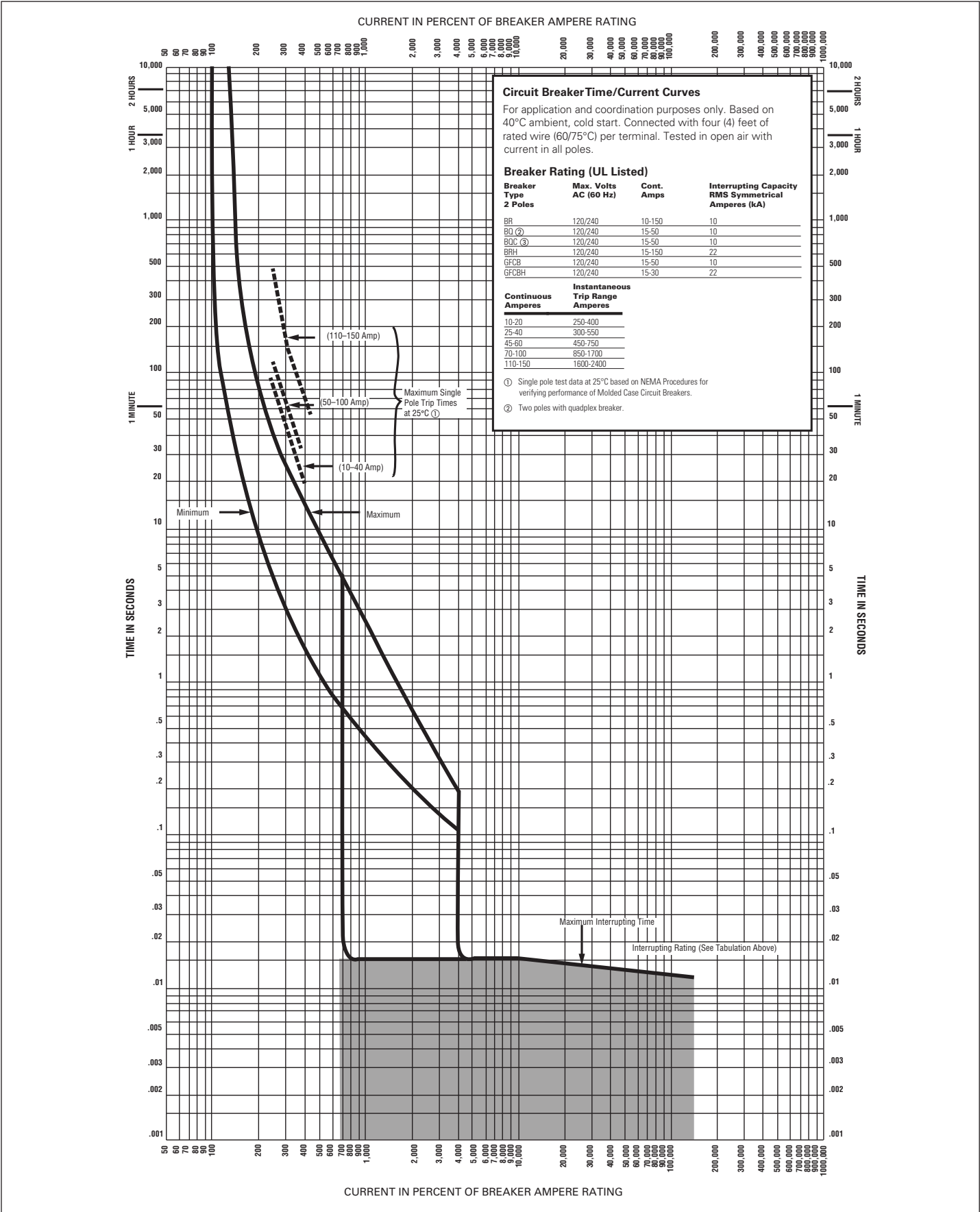
Figure 3. Types BR, BQ, BQC, BRH, GFCB, GFCBH - 10-150 Amperes, 2 Poles.
