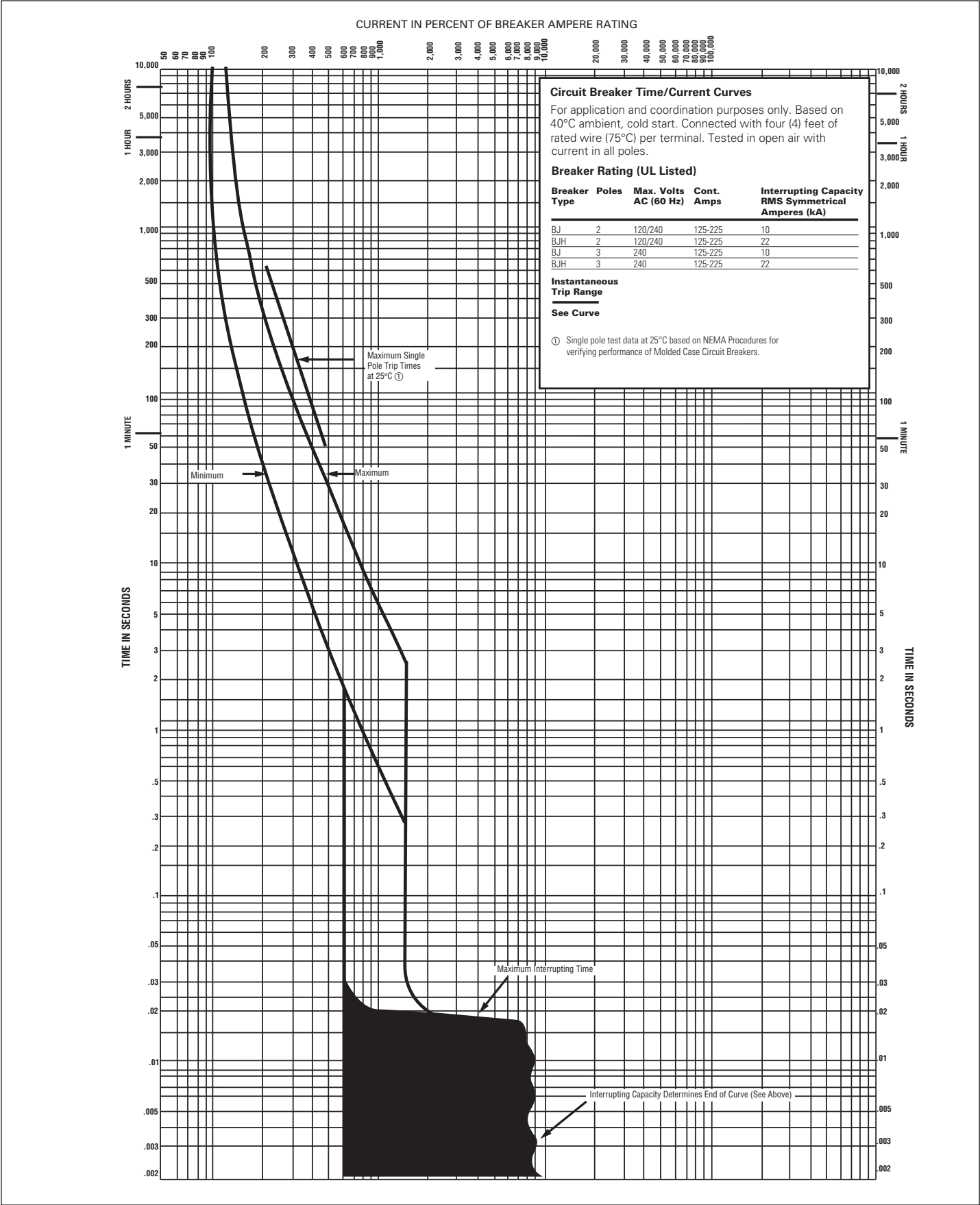
Figure 5. Types BJ and BJH - 125–225 Amperes, 2 and 3 Poles.
