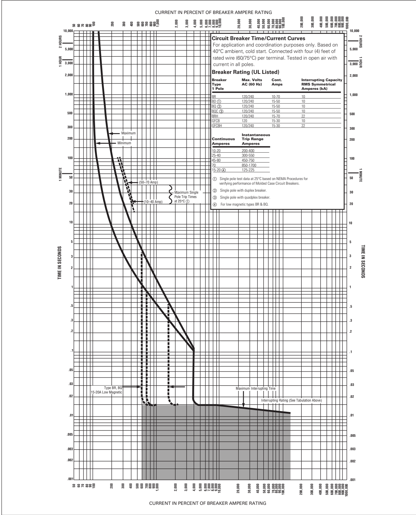
Figure 1. Types BR, BD, BQ, BQC, BRH, GFCB, GFCBH - 10-70 Amperes, 1 Pole.
