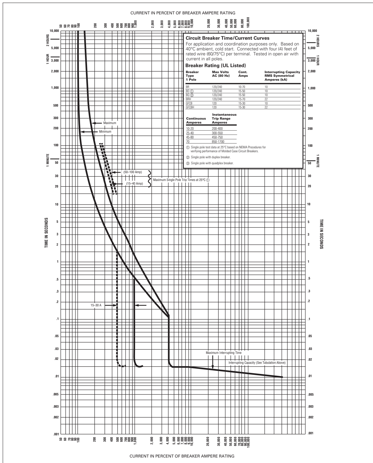
Figure 2. Types BR, BD, BQ, BRH, GFCB, GFCBH - 10-70 Amperes, 1 Pole.
