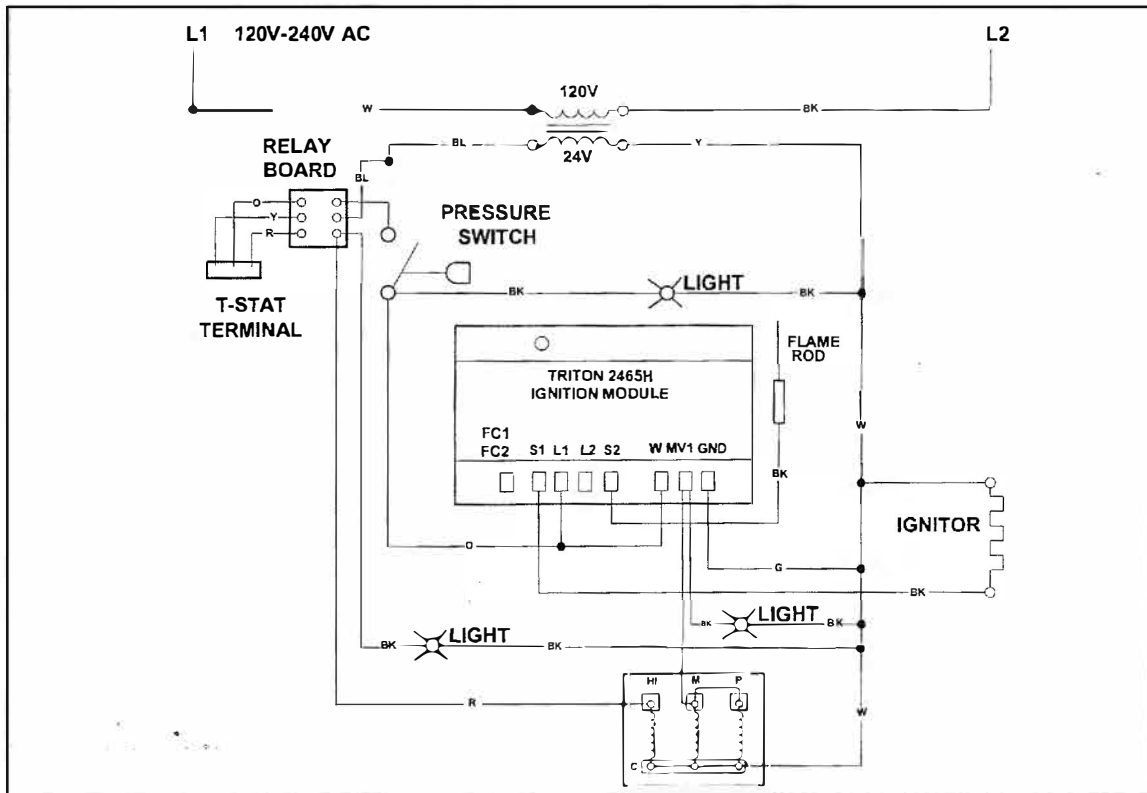
Figure 4-2 Ladder Wiring Diagram
