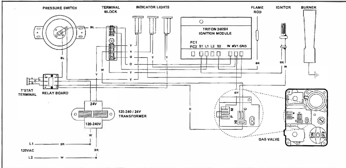
Figure 4-1 Block Wiring Diagram
