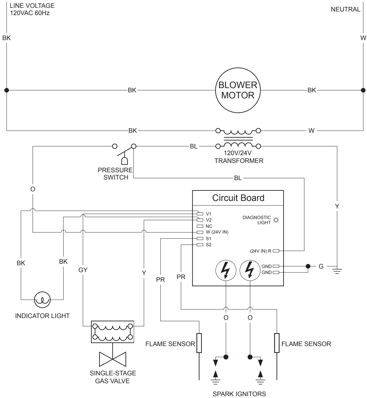
Figure 3.23 • Internal Ladder Wiring Diagram
