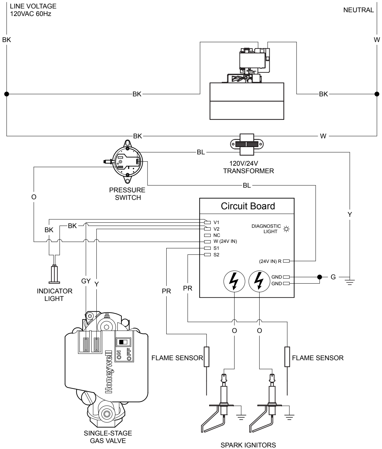
Figure 3.24 • Internal Block Wiring Diagram
