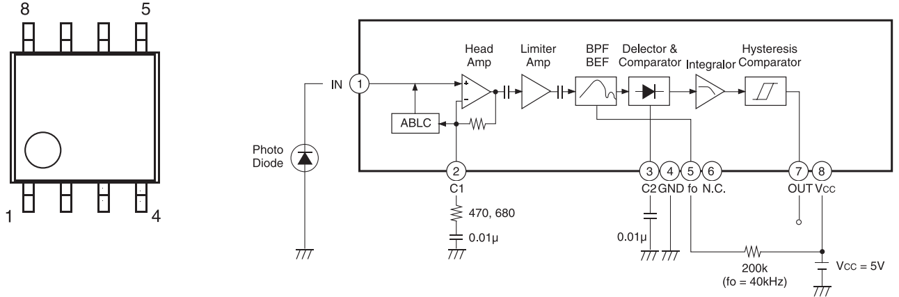
Block Diagram and Pin Configuration
