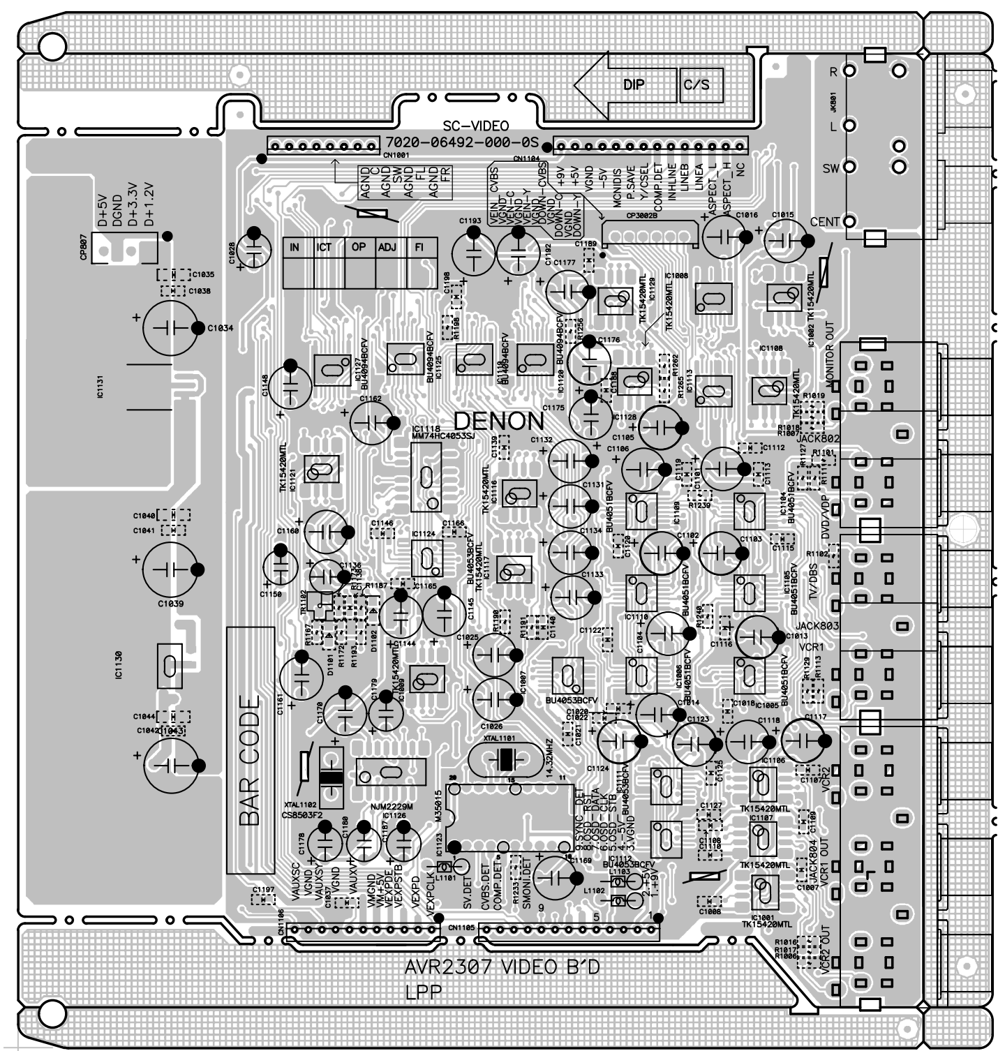
COMPONENT SIDE
