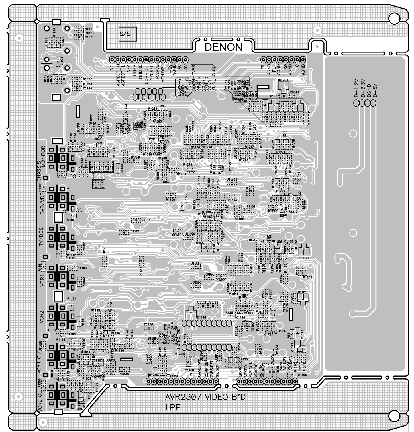
FOIL SIDE
