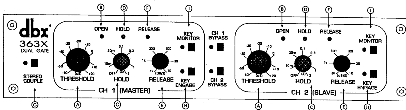
Figure 10: Front Panel
