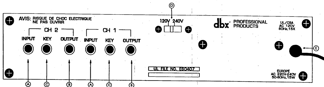
Figure 3: Rear Panel
