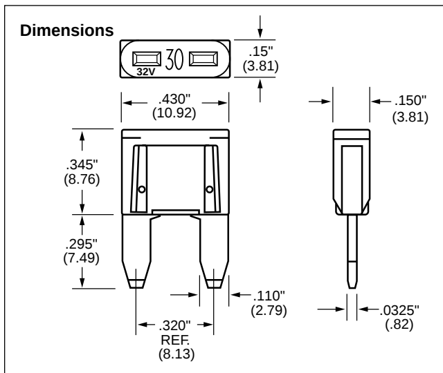
ATM Mini® - Fuse Fast Acting
