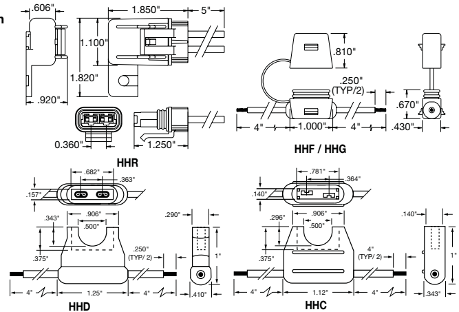
Dimensions - in
