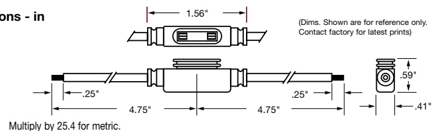
Dimensions - in
