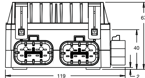
Standard VEC shown with vented cover
