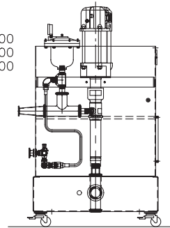
APPLICATOR TANK
