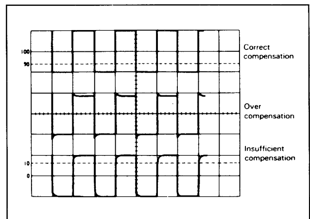
Fig. 5. Probe Compensation Adjustment.
