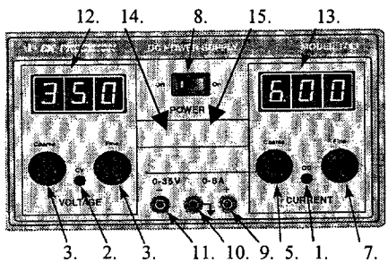
Figure 1. Front Panel Controls (1744 top – 1745 bottom).
