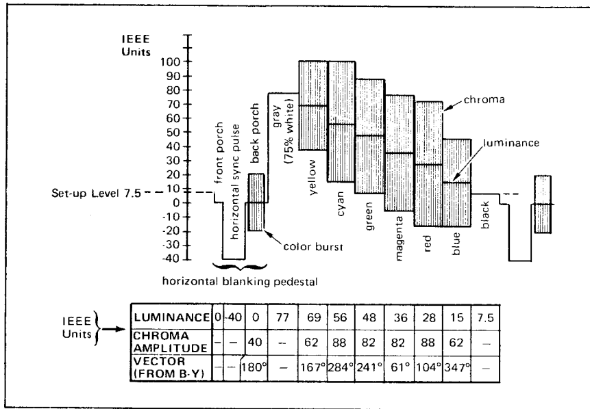
Fig. 1. Composite Video Signal; One Horizontal Line of NTSC Color Bars Signal.
