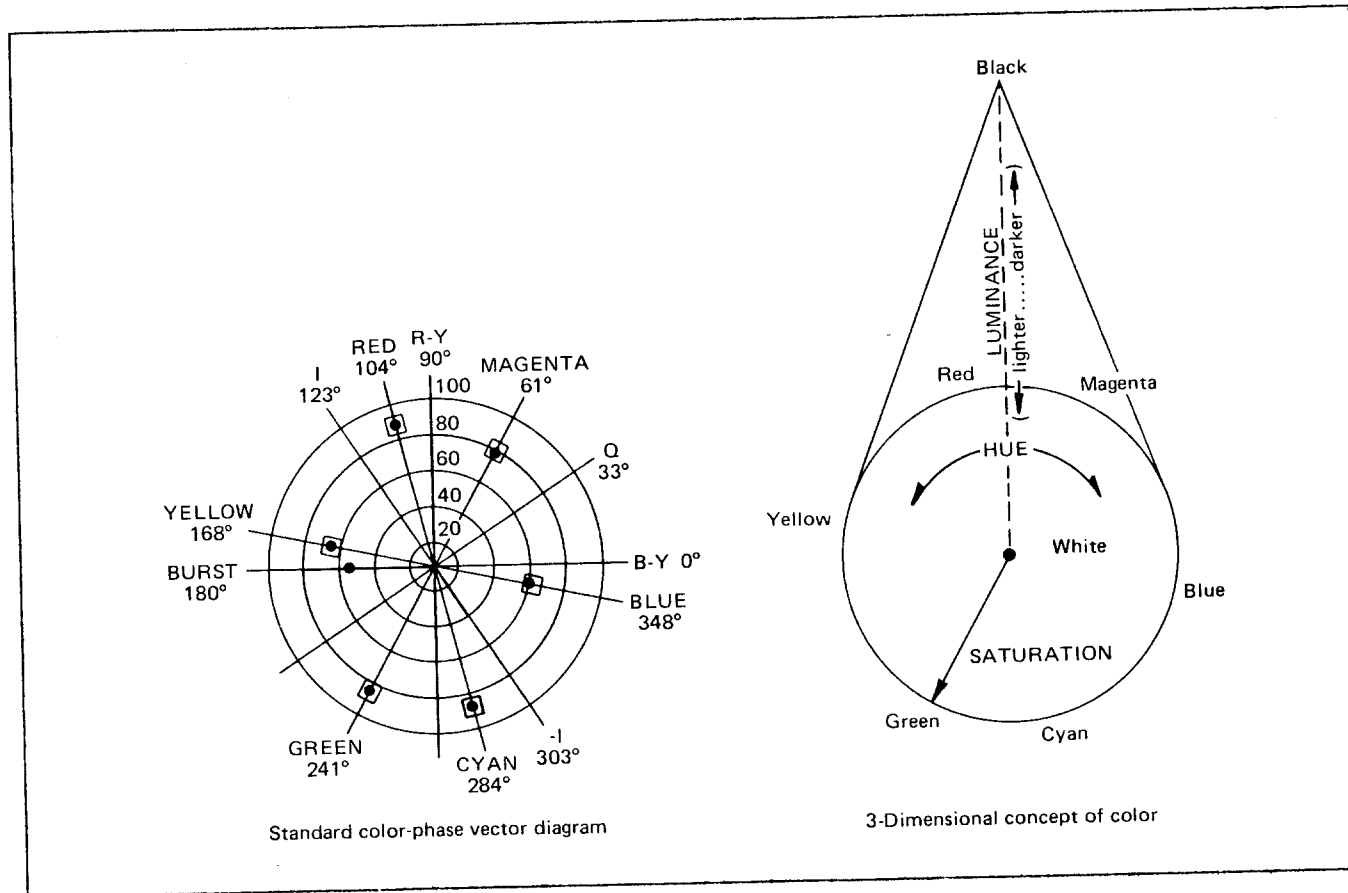
Fig. 3. Elements of Color Television Signal.
