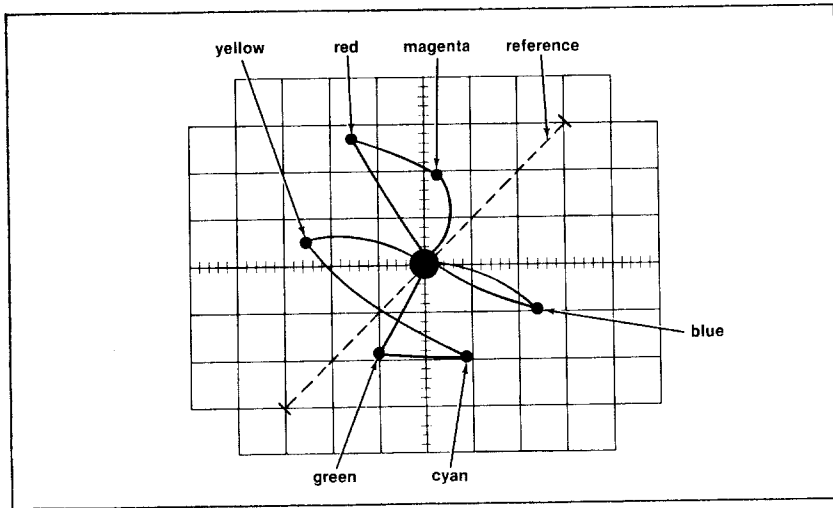
Fig. 7. Typical Vectorscope Display of Demodulated Color Bars Pattern Viewed on Conventional Oscilloscope.
