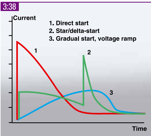
Starting current with different starting methods.
