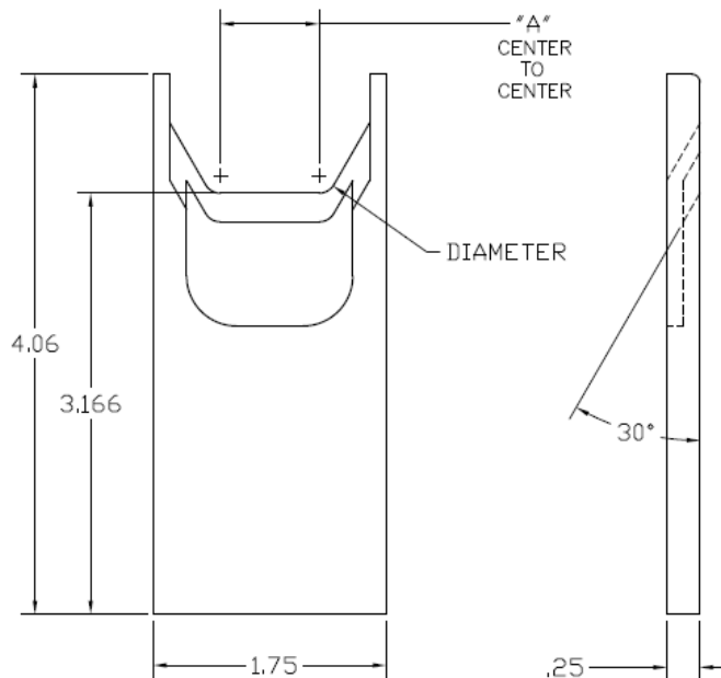
123758-x Oval cord stripping blade
