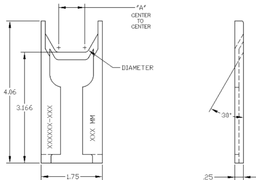
150104-x Oval cord stripping blade
