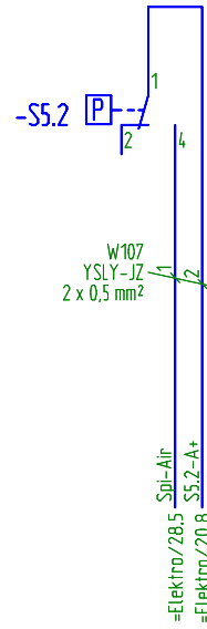
compressed air switch drill spindle
