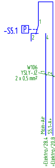
compressed air switch main air
