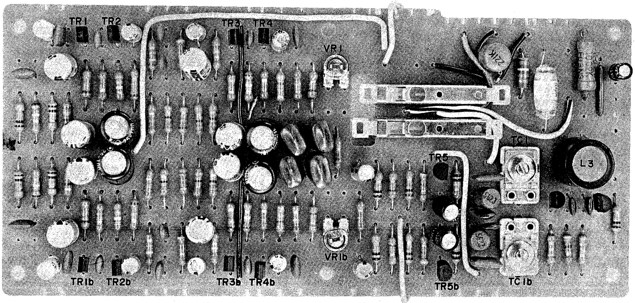
Fig. 22 REC. AMP./OSC. P.C. BOARD TD-5003 (Front Side)
